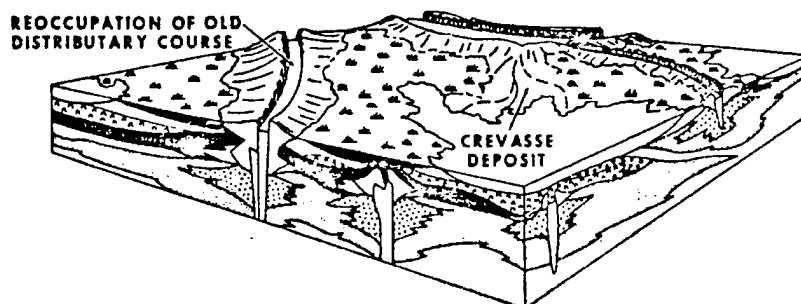
Figure 21. Deltaic environments of deposition (from Frazier and Osanik, 1969)
