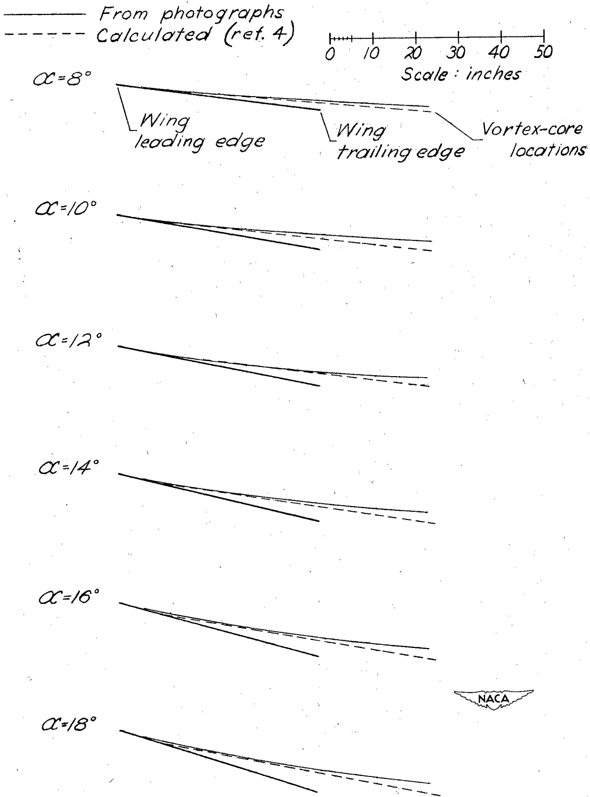
Figure 7.- Vortex-core locations in the vertical plane for a modified flat-plate rectangular wing of aspect ratio 0.25.
