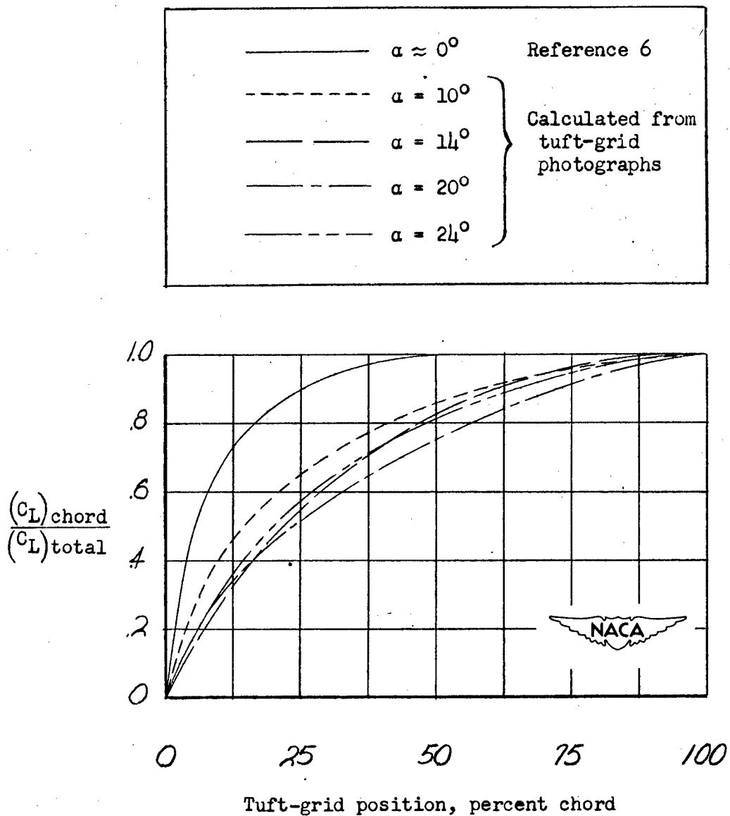
Figure 10.- Chordwise growth of lift on modified flat-plate wing of aspect ratio 0.25. Comparison of theoretical values and values calculated from tuft-grid photographs. Wing chord, 48 inches.
