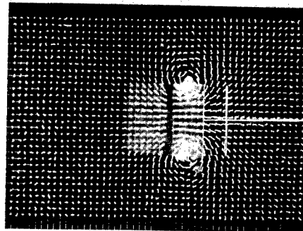
125 percent chord
