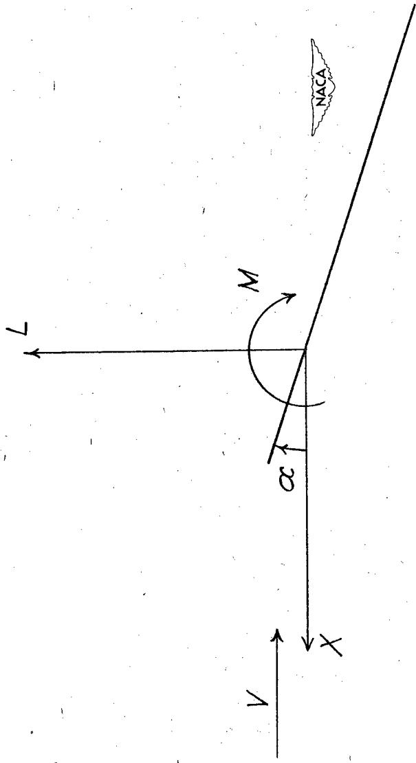
Figure 1.- System of axes used. Arrows indicate positive directions of forces, moment, and angle.
