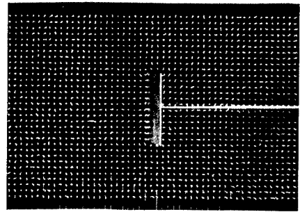
37.5 percent chord
