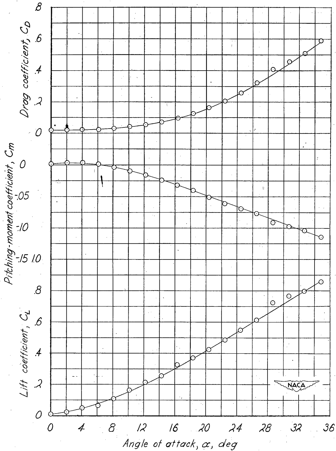
(a) Lift, pitching-moment, and drag coefficients.
