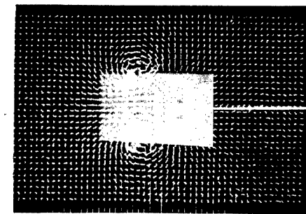
50.0 percent chord
