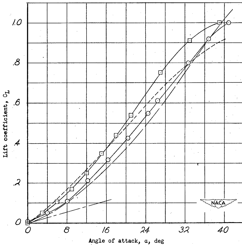
Figure 4.- Comparison of lift curves of a rectangular wing of aspect ratio 0.25 obtained from various sources.
