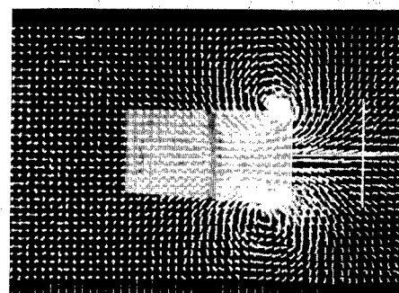
75.0 percent chord
