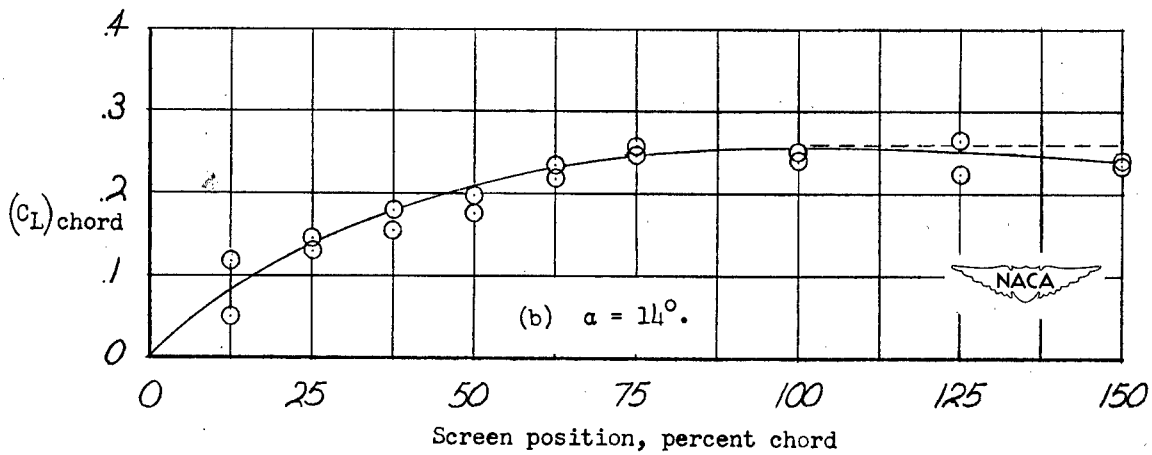
Figure 9.- Chordwise growth of lift on modified flat-plate wing of aspect ratio 0.25 for several angles of attack. Calculated from trailing-vortex strengths using tuft-grid photographs. Wing chord, 48 inches.
