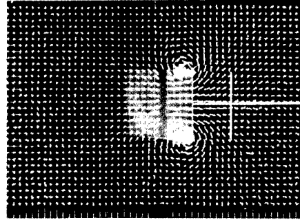
150 percent chord
