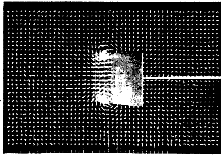
37.5 percent chord
