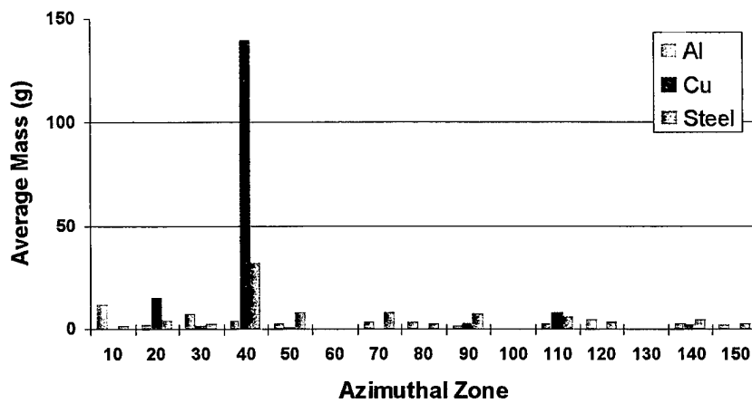
Figure 30. Distributions With Azimuth of the Number of Fragments, the Total Fragment Mass, and the Average Fragment Mass - Boxed Hellfires.
