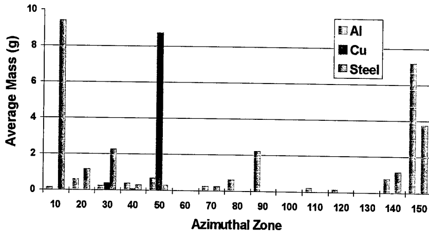
Figure 24. Distributions With Azimuth of the Number of Fragments, the Total Fragment Mass, and the Average Fragment Mass - Single Hellfire.
