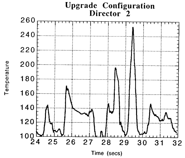
Figure 11. Temperature time history at Director 2 for (a) baseline configuration and (b) upgrade configuration for a 20 kt ship speed and 20 kt wind speed at 0° (headwind).
