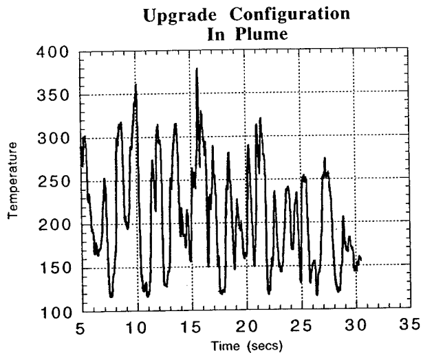
Figure 35. Temperature time history at location 'In Plume' for (a) baseline configuration and (b) upgrade configuration for a 14 kt ship speed and 20 kt wind speed at 180° (tailwind).
