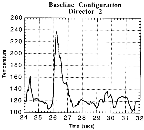
Figure 11. Temperature time history at Director 2 for (a) baseline configuration and (b) upgrade configuration for a 20 kt ship speed and 20 kt wind speed at 0° (headwind).
