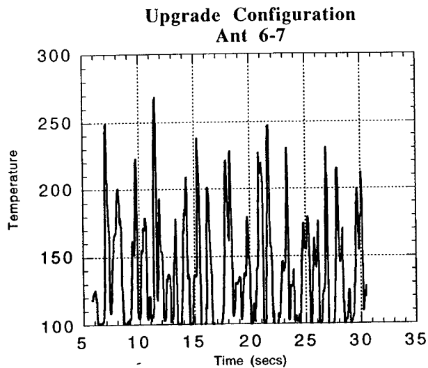
Figure 34. Temperature time history at Ant. 6-7 for (a) baseline configuration and (b) upgrade configuration for a 14 kt ship speed and 20 kt wind speed at 180° (tailwind).
