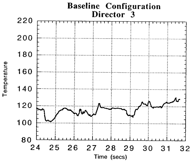
Figure 12. Temperature time history at Director 3 for (a) baseline configuration and (b) upgrade configuration for a 20 kt ship speed and 20 kt wind speed at 0° (headwind).
