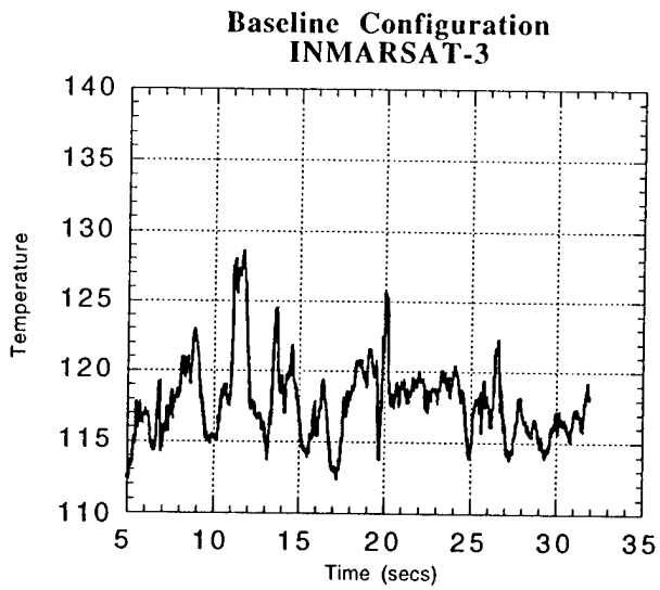
Figure 20. Temperature time history at INMARSAT-3 for (a) baseline configuration and (b) upgrade configuration for a 14 kt ship speed and 20 kt wind speed at 180° (tailwind).
