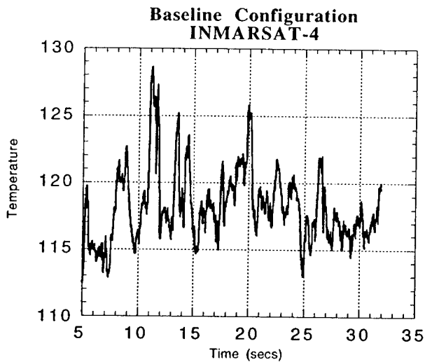
Figure 21. Temperature time history at INMARSAT-4 for (a) baseline configuration and (b) upgrade configuration (missing data) for a 14 kt ship speed and 20 kt wind speed at 180° (tailwind).
