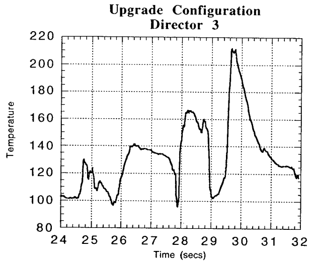
Figure 12. Temperature time history at Director 3 for (a) baseline configuration and (b) upgrade configuration for a 20 kt ship speed and 20 kt wind speed at 0° (headwind).
