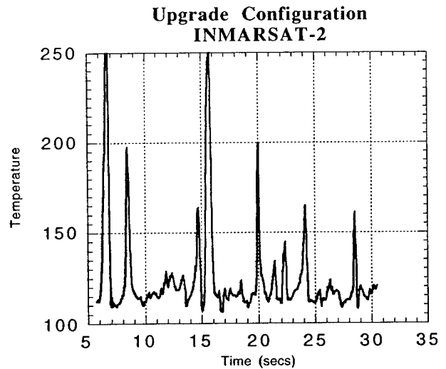
Figure 19. Temperature time history at INMARSAT-2 for (a) baseline configuration and (b) upgrade configuration for a 14 kt ship speed and 20 kt wind speed at 180° (tailwind).
