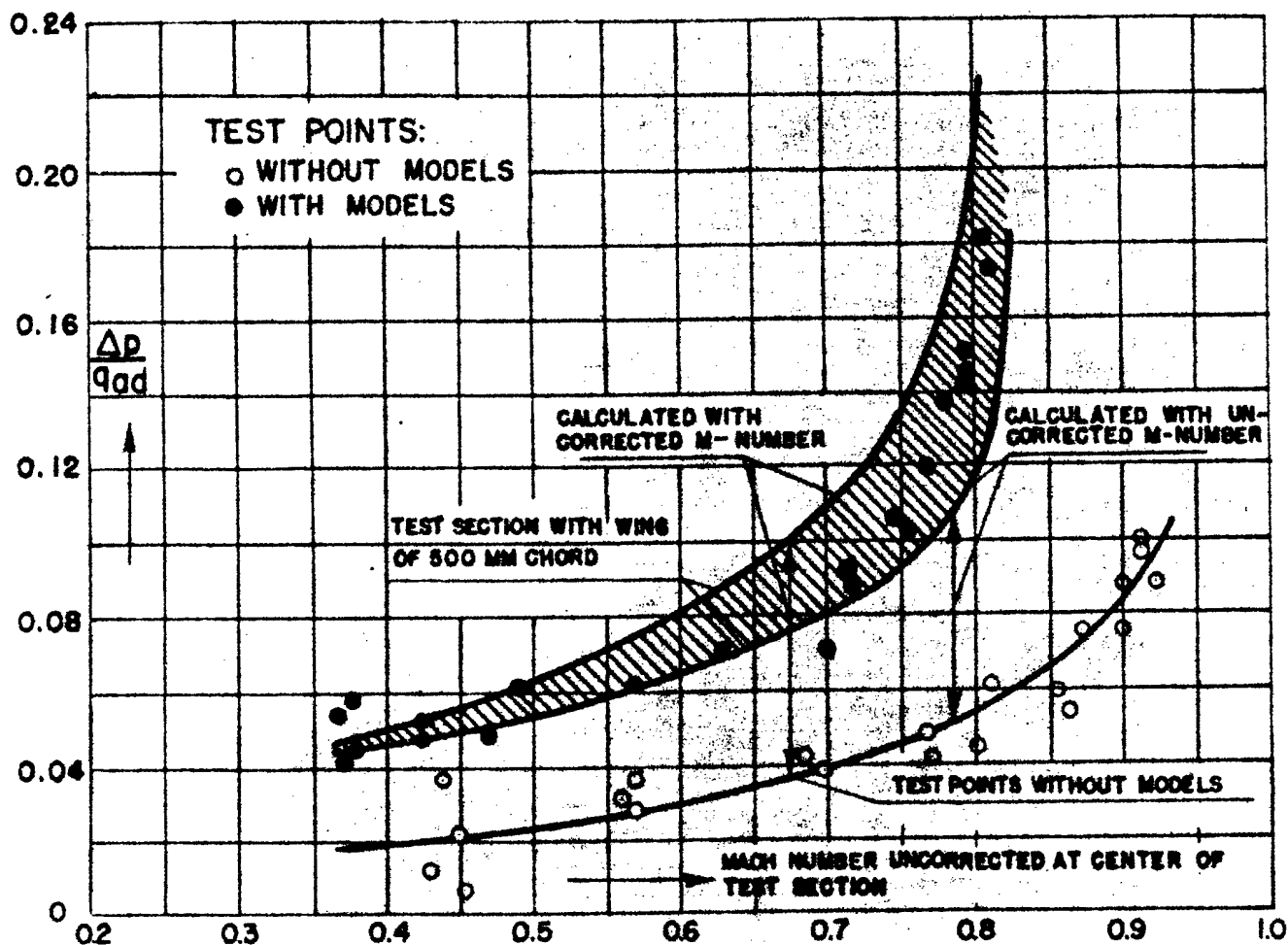
Fig. 17 - Pressure Drop p in Test Section with and without Model \Delta p = p Beginning - P end = Difference of Wall Pressure Between q_{ad} = P_0 - P_{t s} = Adiabatic Dynamic Pressure at Tunnel Center
