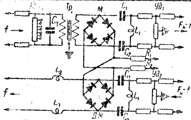
Fig. 3.4 Circuits of individual converters.
