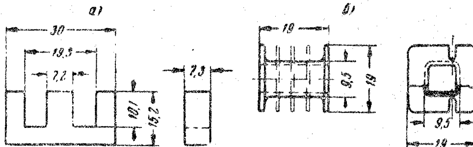
Fig. 1.9. Ferrocort transformer core type OSh-7. Frame of coil OSh-7.
