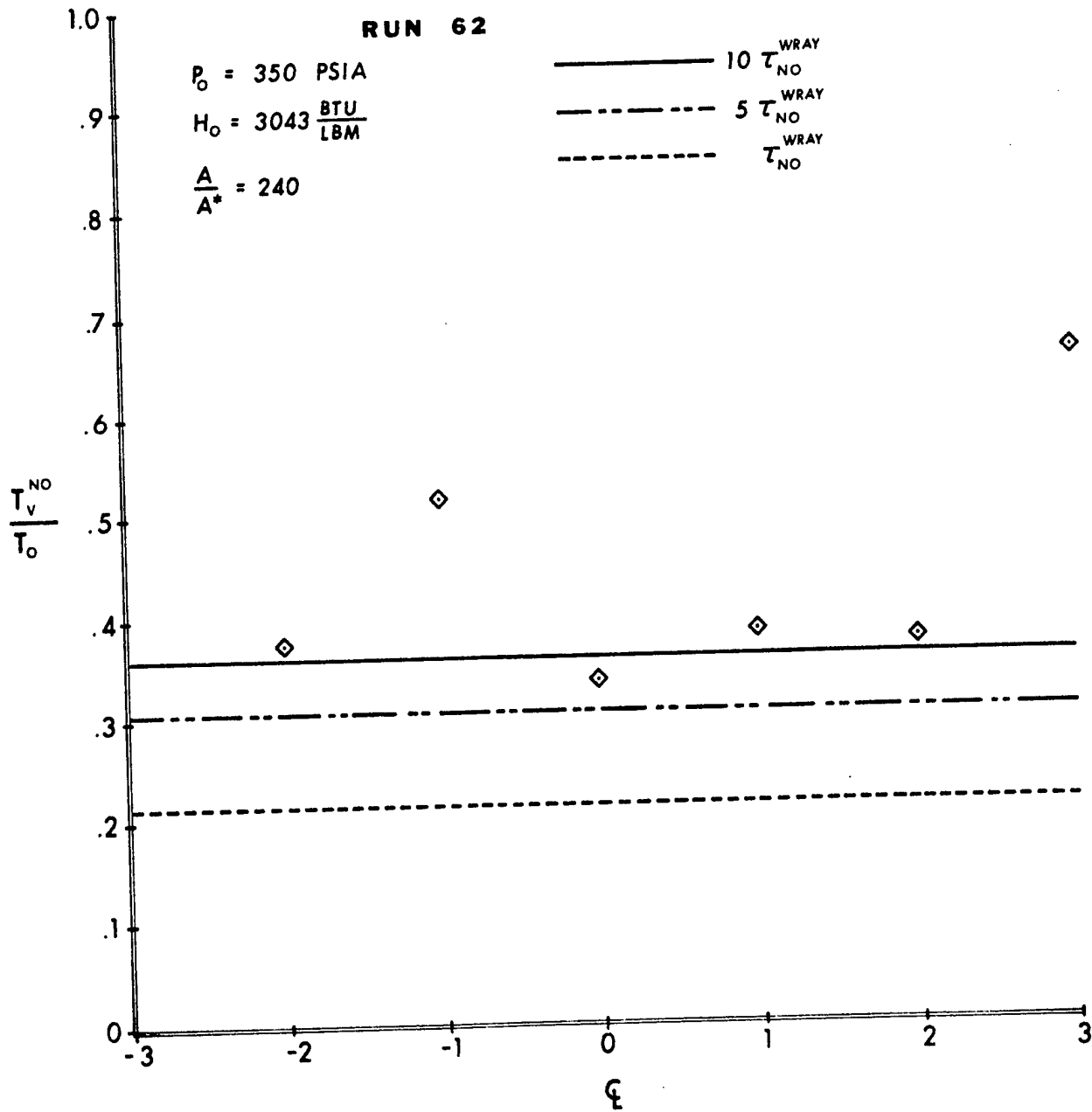
FIGURE 2. COMPARISON OF NO VIBRATIONAL TEMPERATURE DATA WITH NONEQUILIBRIUM CALCULATIONS ( T_0 = 4356^\circ\text{K} , P_0 = 350 \text{ psia} , A/A^* = 240 )
