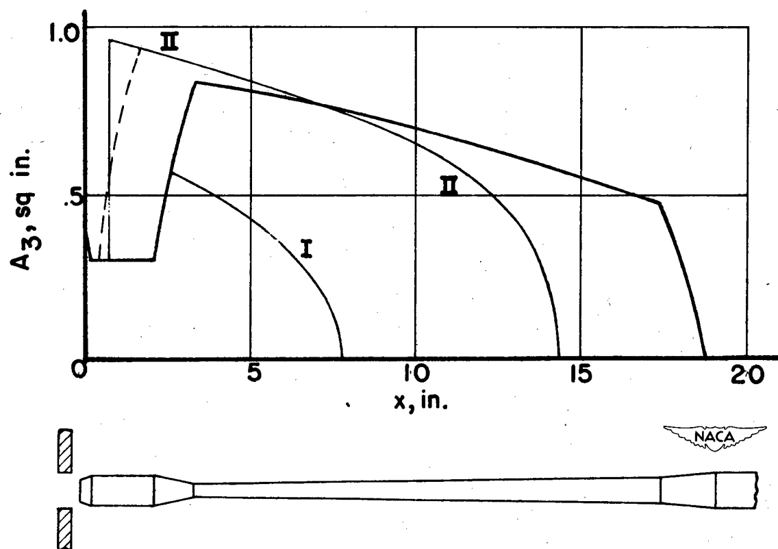
Figure 13.- Cross section of metering pin.
