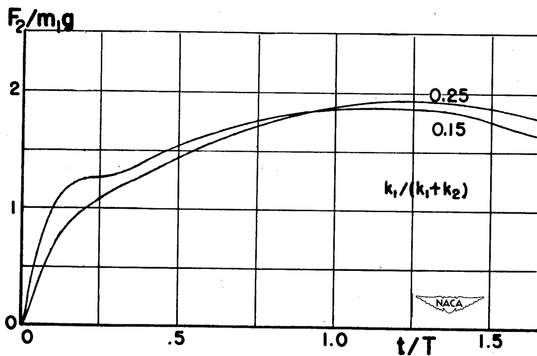
(b) Force on wheel.
