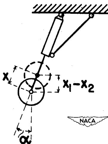
Figure 20.- Example of landing gear with shock strut inclined from vertical.
