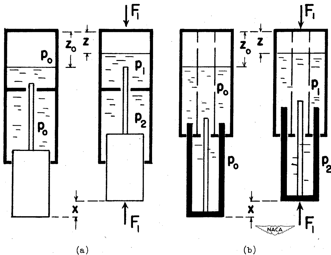
Figure 10.- Different forms of oleo struts.
