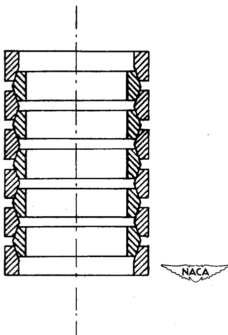
Figure 26.- Ring-pile spring.
