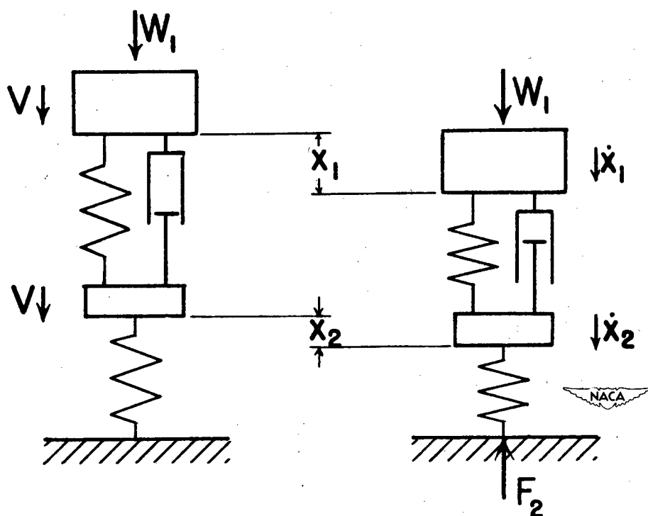
Figure 1.- Representation of shock strut by spring and damper arranged in parallel.
