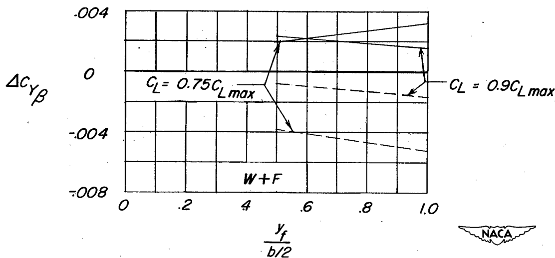
(c) \Delta C_{y\beta} against \frac{y_f}{b/2} .
