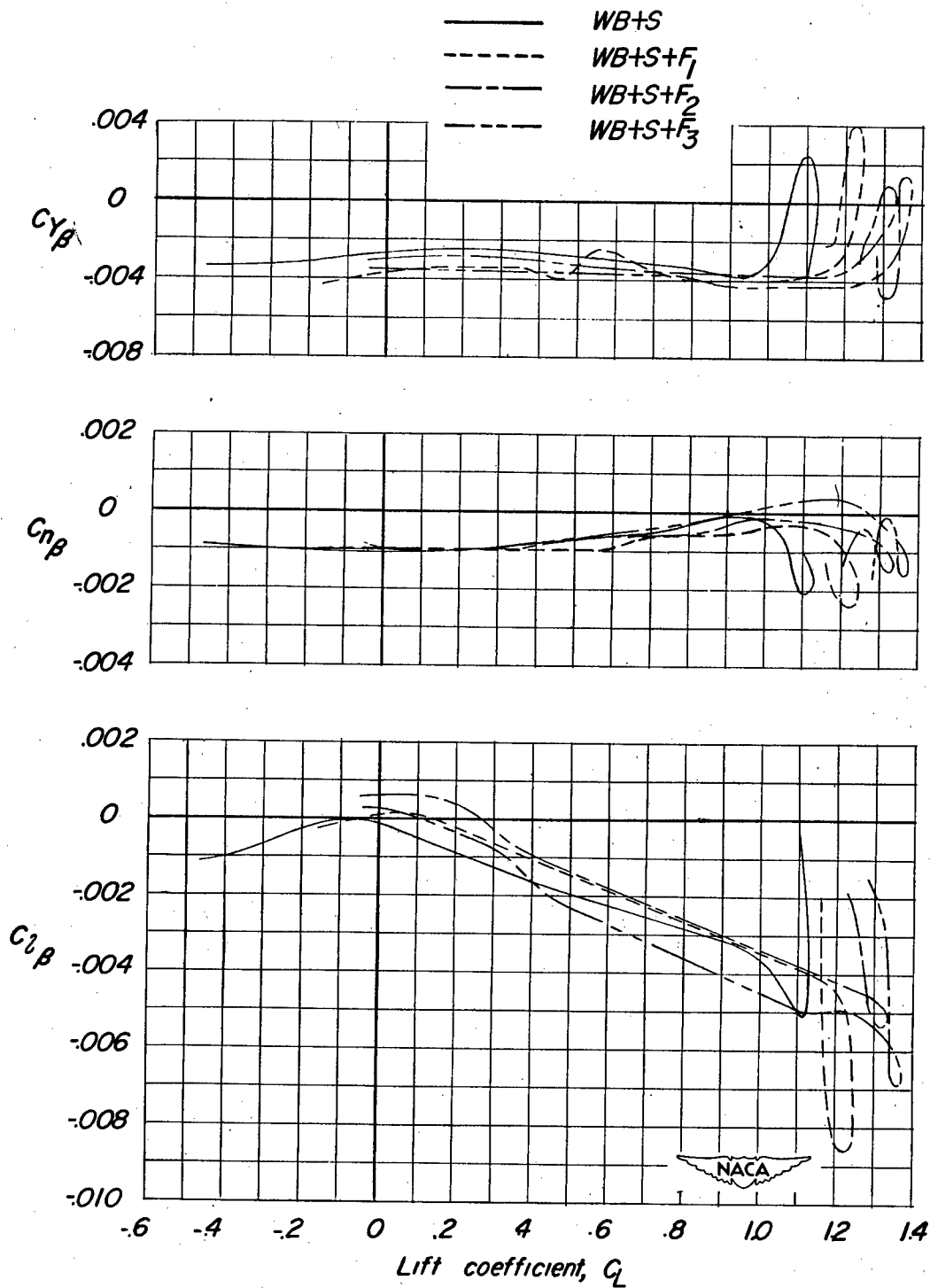
(c) Wing-body configuration with slats extended and plain flaps deflected.
