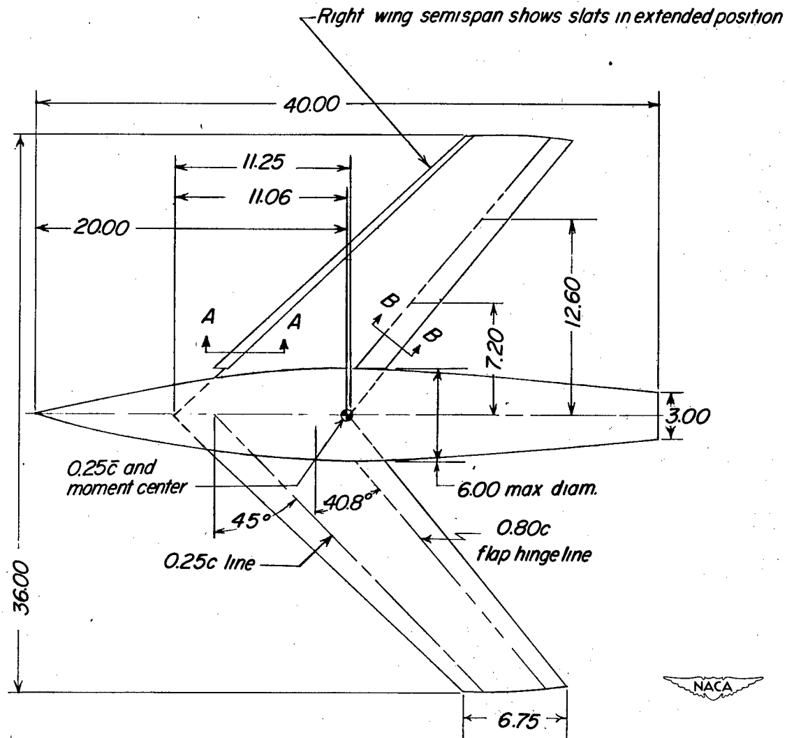
Figure 2.- Dimensions of the model. Wing has aspect ratio of 4, taper ratio of 0.6, and was mounted along the body center line. All dimensions are in inches.
