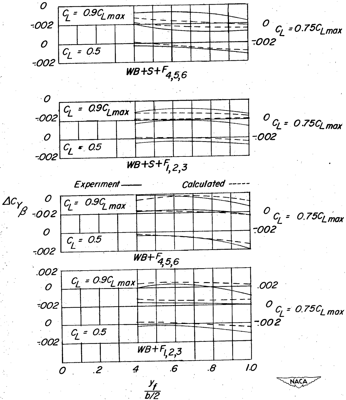
(c) \Delta C_{Y\beta} against \frac{y_f}{b/2} .
