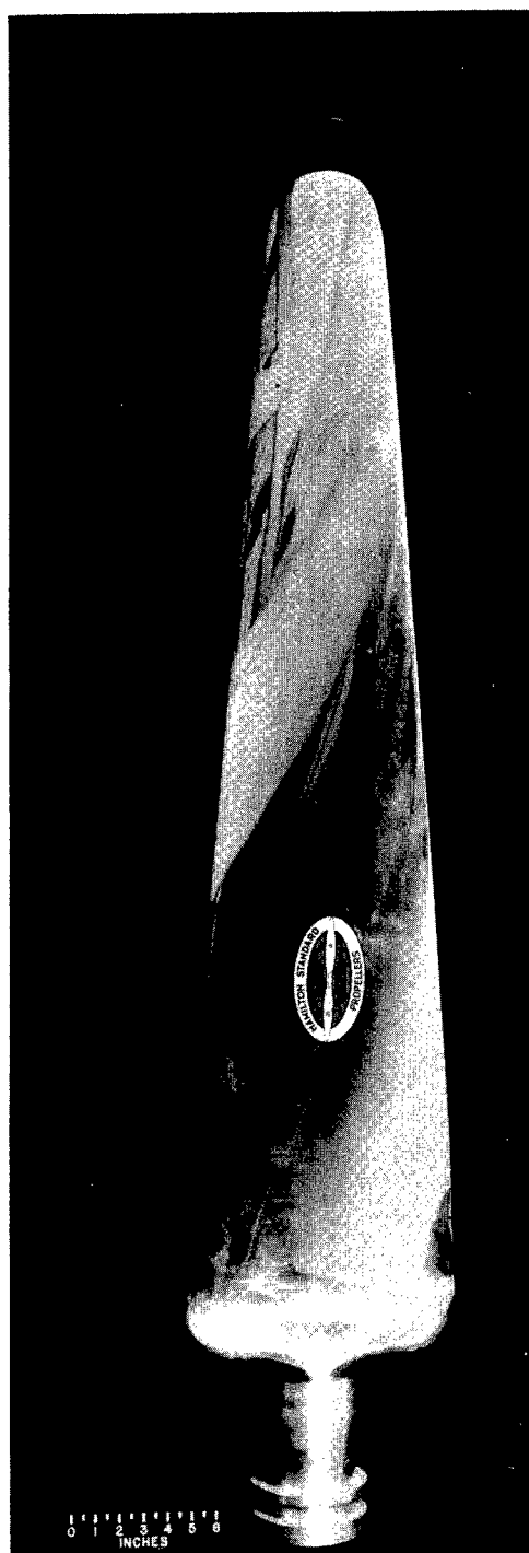
Figure 17.- Blade of NACA 10-(3)(08)-03 propeller.
