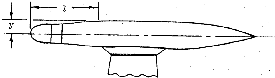
ORDINATES FOR THE DYNAMOMETER-FAIRING PROFILE
