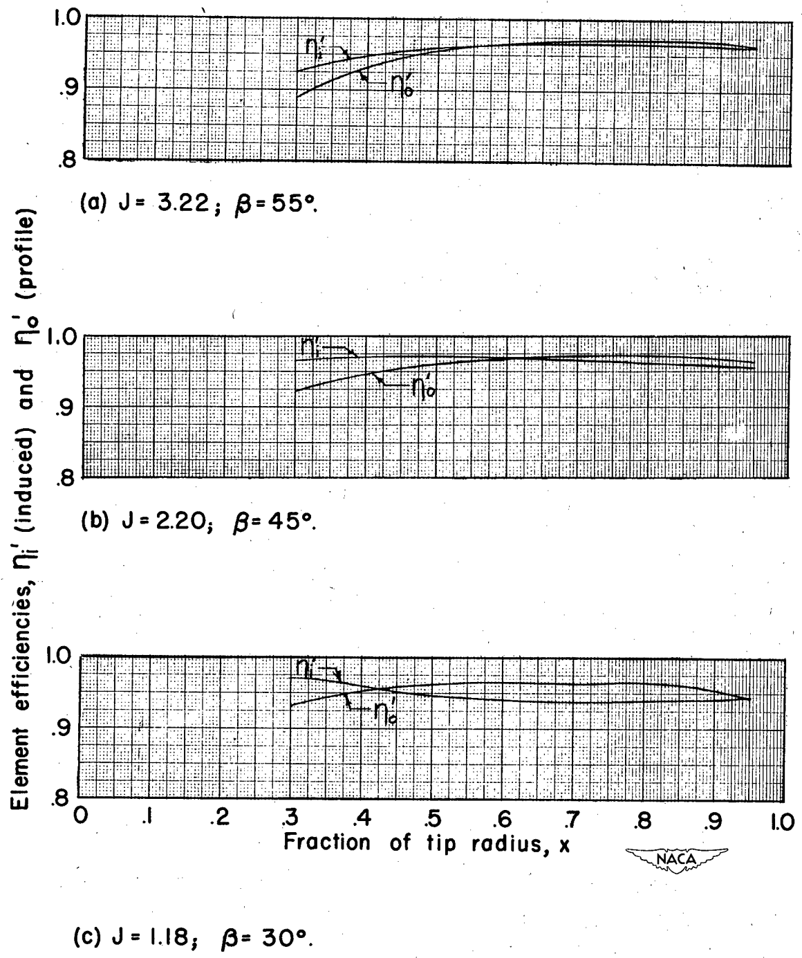
Figure 33.- Calculated distribution of induced and profile efficiencies along the NACA 10-(3)(08)-03 propeller blade at 1,140 rpm.
