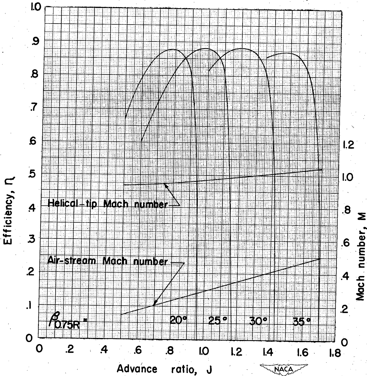
Figure 23.- Concluded. Rotational speed, 2,000 rpm.
