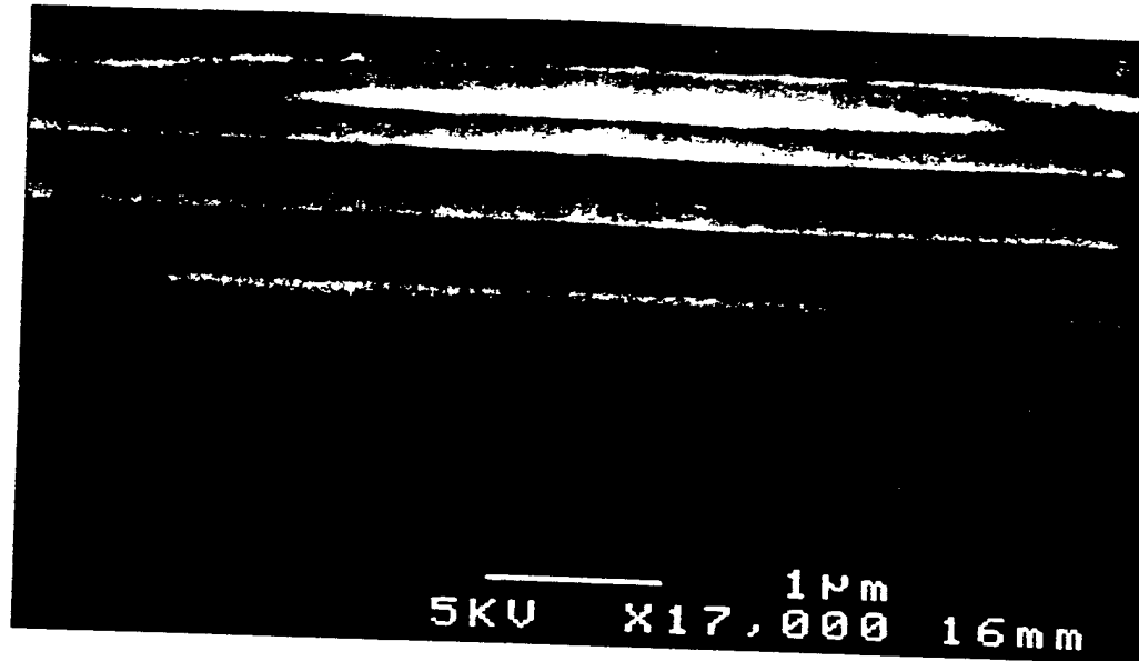
Figure 7-9: An SEM showing two oxide fronts can bow the semiconductor surface before closing off. (The fronts were closing off a 100\mu\text{m} wide mesa after being in the furnace for 30' at 450^\circ\text{C} . The top AlGaAs layer is 246nm of 97.5% Al with a 10nm layer of AlAs in the middle. The layer is beneath 100nm of GaAs)
