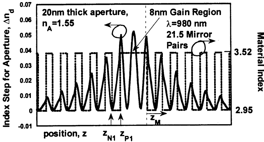
Figure 4-5: Plot of the distributed index step, \Delta n_d calculated for a 20nm thick oxide ( n=1.55 ) aperture vs. position in the cavity. The refractive index distribution in the unapertured cavity is indicated by the dashed line.
