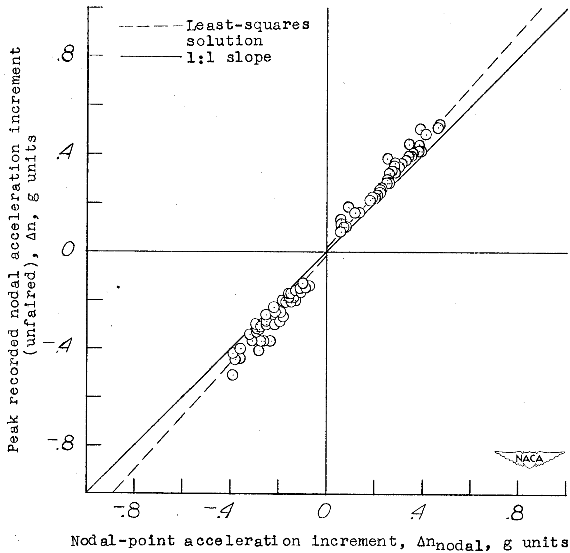
Figure 12.- Peak recorded nodal accelerations (unfair) as a function of nodal-point accelerations.
