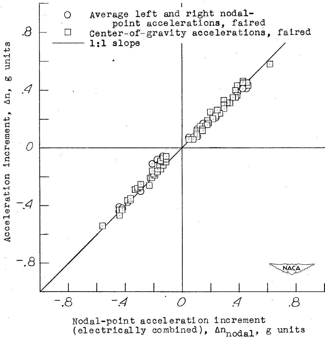
Figure 7.- Comparison of means of determining nodal-point acceleration.
