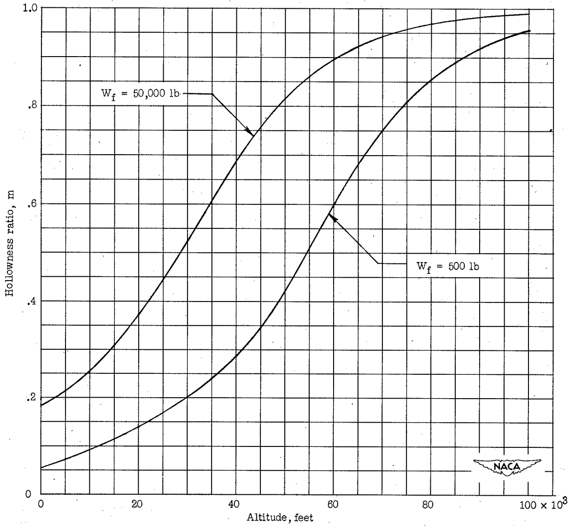
Figure 8.- Hollowness ratio of diamond wings. General method and approximate method I ( \eta = 0 ). \frac{\sigma_a}{n_{max}} = 5,000 pounds per square inch; double-wedge profile; aspect ratio, 4.0; Mach number, 2.0; aluminum wings; r = m ; C_{D_f} = 0.005 ; n = 1 .
