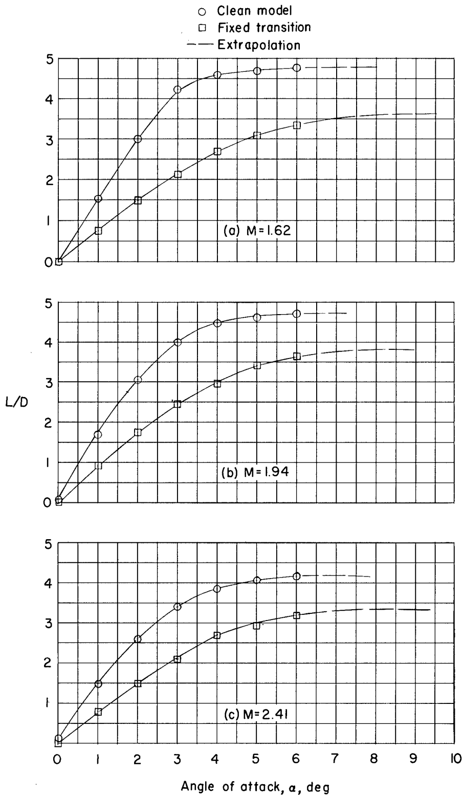
Figure 6.- Variation of L/D with angle of attack.
