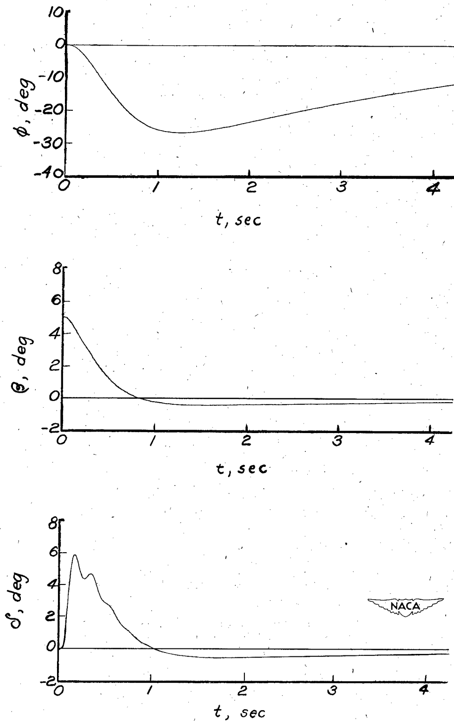
Figure 19.- Airplane and rudder motions with autopilot designed for maximum possible damping with \zeta = 0.3 . K = 0.5386 deg/deg/sec; \omega_0 = 33.3 radians per second; \zeta = 0.3 .
