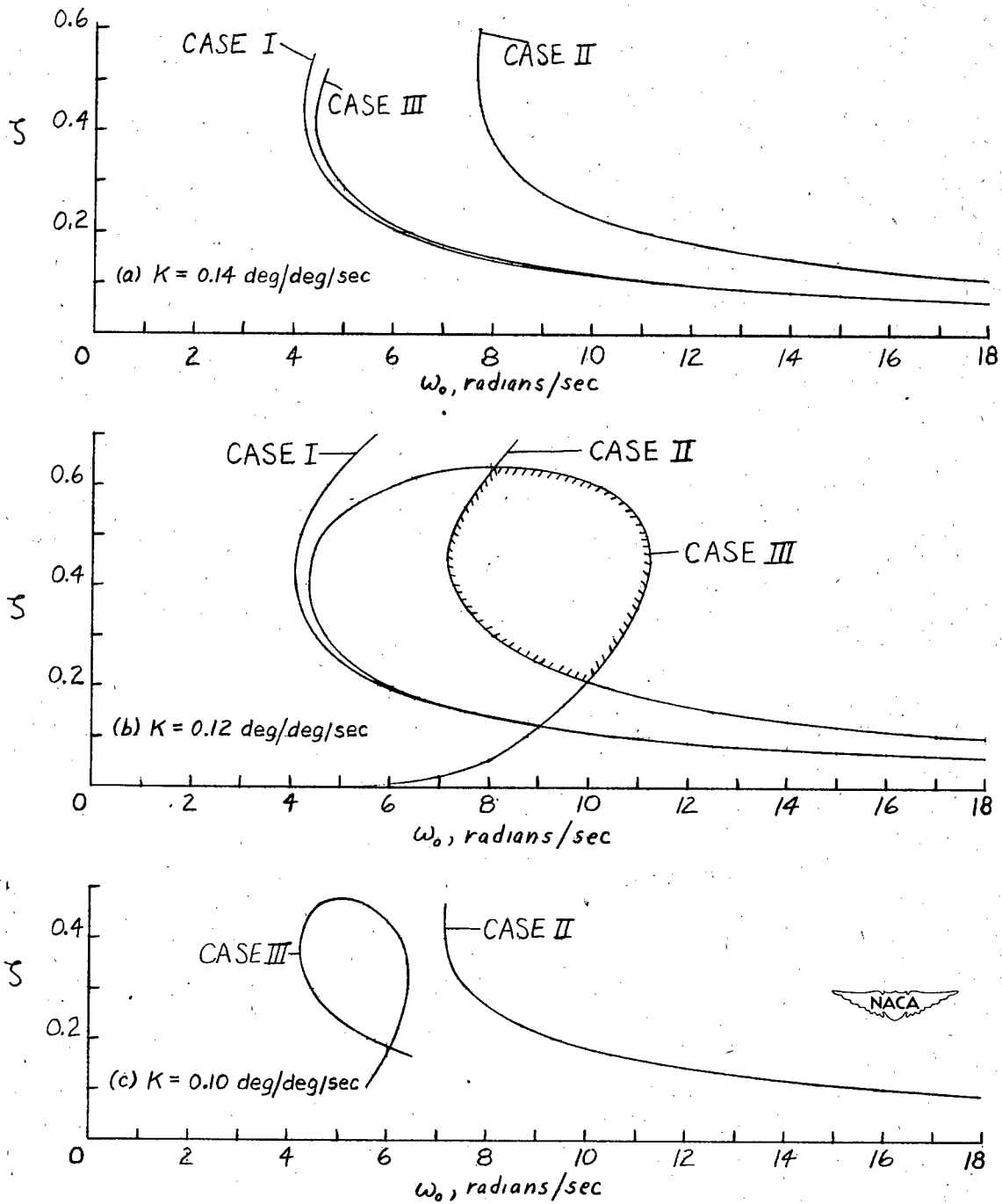
Figure 22.- Boundaries of the region where T_{1/2} < 1.00 second in the \zeta\omega_0 -plane for three flight conditions of the airplane when a yaw damper with three different gearings is used.
