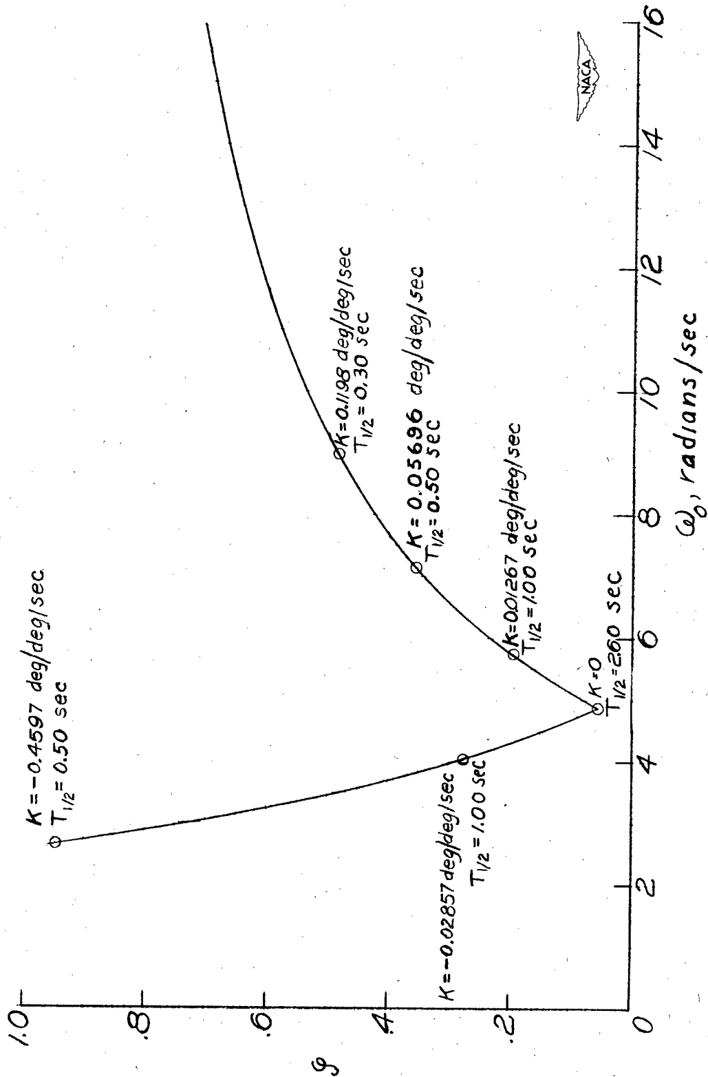
Figure 10.- Variation of optimum points in the \zeta\omega_0 -plane for varying autopilot gearing ratio.
