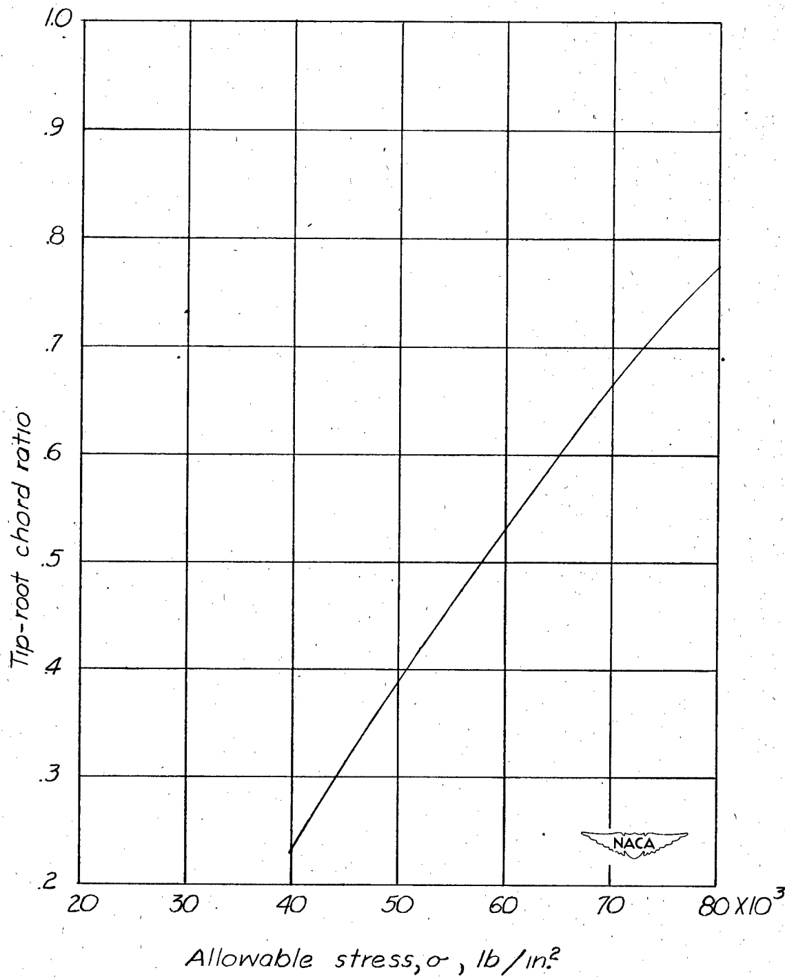
Figure 2.- Effect of allowable stress on tip-root chord ratios for steel propellers of constant centrifugal stress. \frac{h}{b} = Constant; J = 2.0 ; M = 0.9 ; altitude, 40,000 feet.
