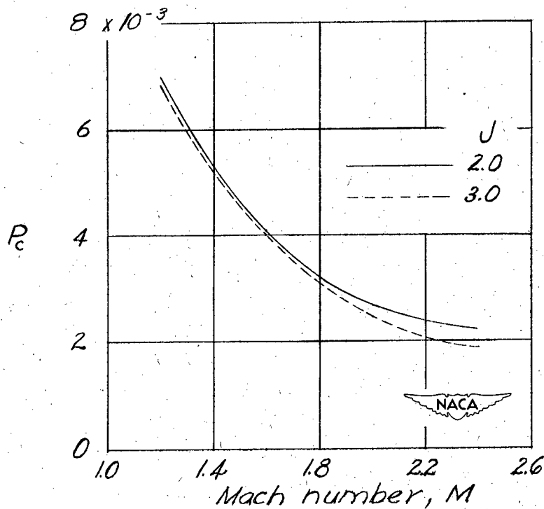
Figure 10.- Power absorption for propellers of constant centrifugal stress. \frac{h}{b} = 0.02 ; \sigma = 48,000 pounds per square inch; altitude, 40,000 feet.
