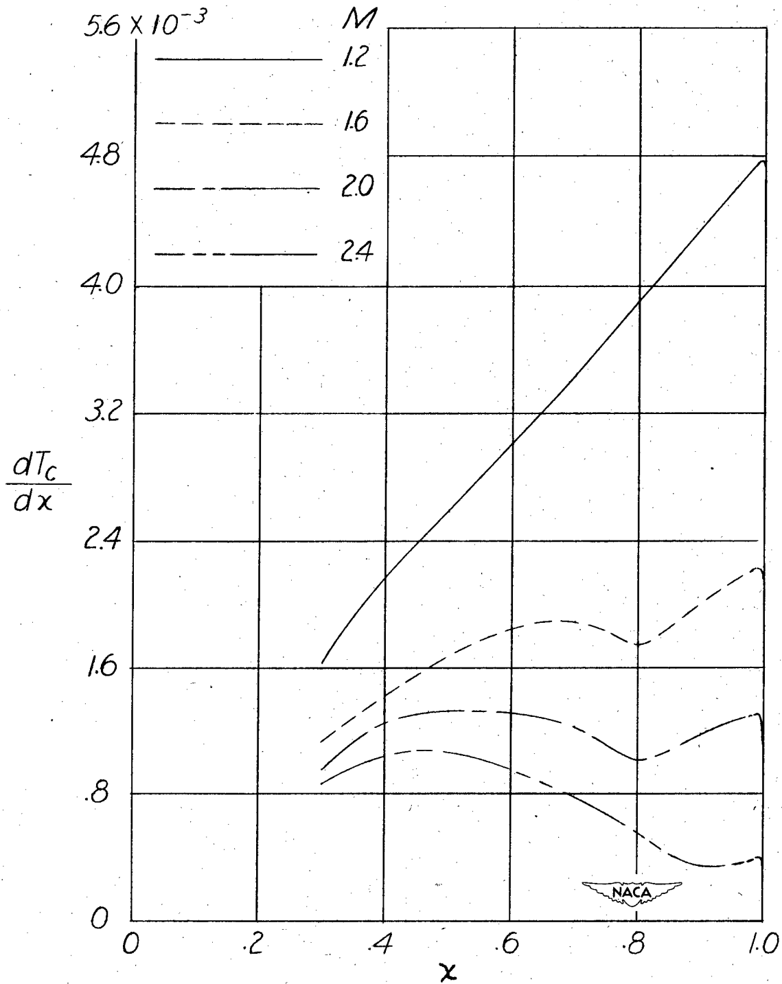
Figure 7.- Thrust-gradient curves for propellers of constant centrifugal stress at an advance ratio of 3.0. \frac{h}{b} = 0.02 ; altitude, 40,000 feet; \sigma = 48,000 pounds per square inch.
