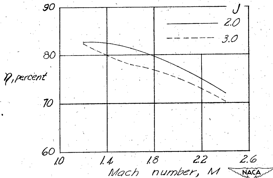
Figure 9.- Efficiency for propellers of constant centrifugal stress. \frac{h}{b} = 0.02 ; \sigma = 48,000 pounds per square inch; altitude, 40,000 feet.
