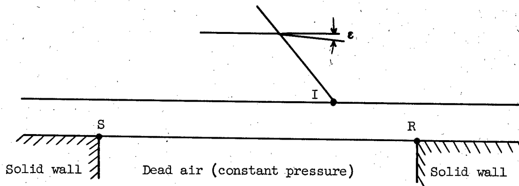
(a) Schematic.
