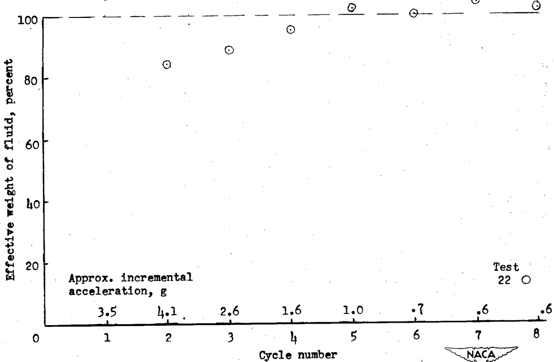
(h) Tank 80 percent full.
