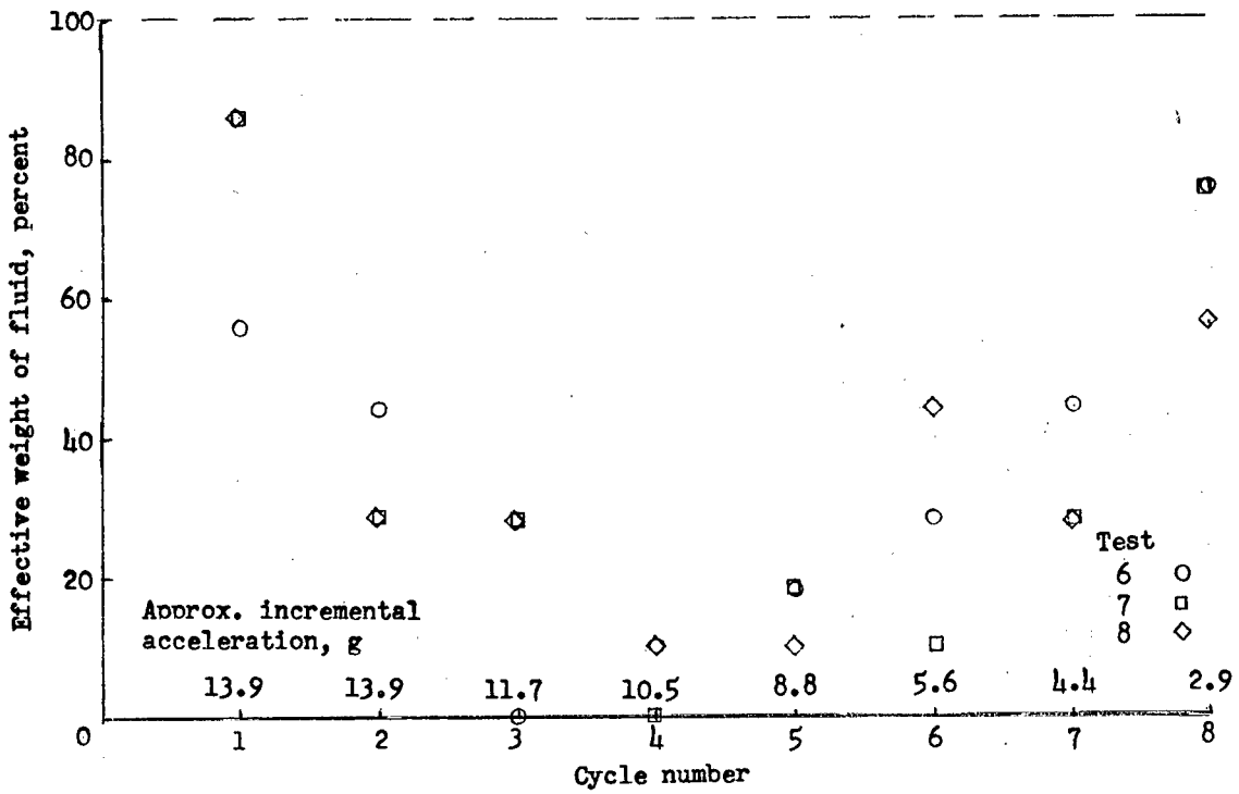
(a) Tank 10 percent full.
