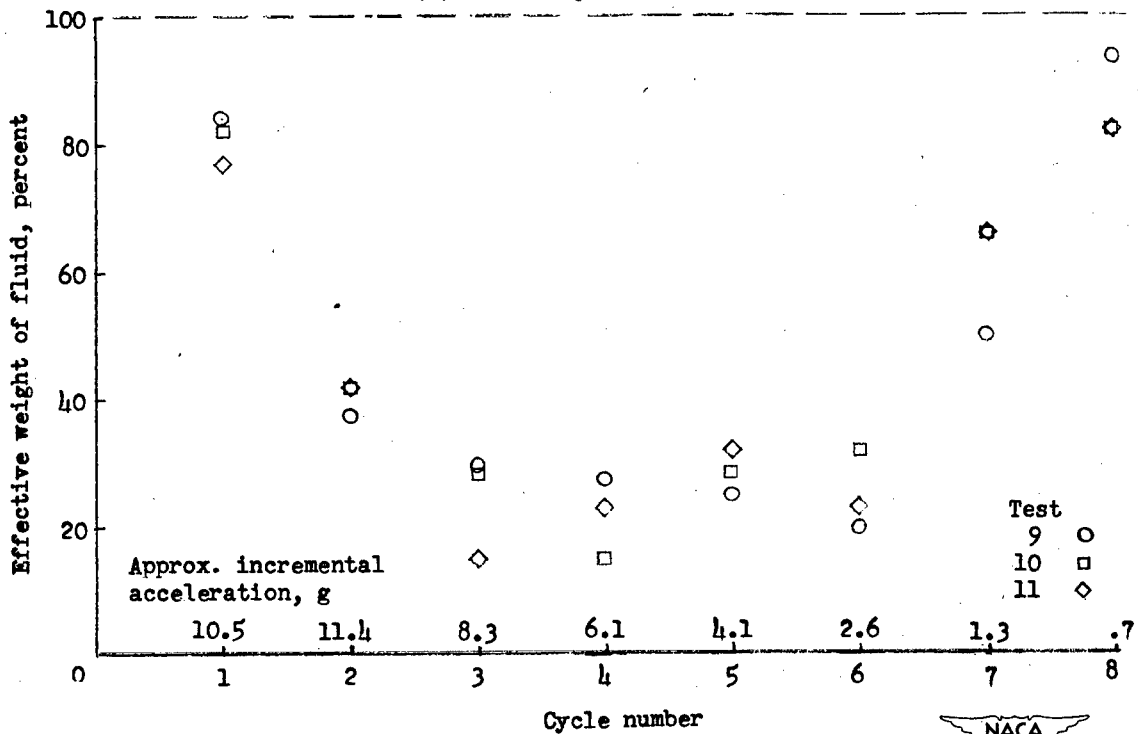
(b) Tank 20 percent full.
