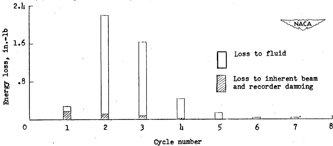
(b) Energy lost by beam during each cycle.
