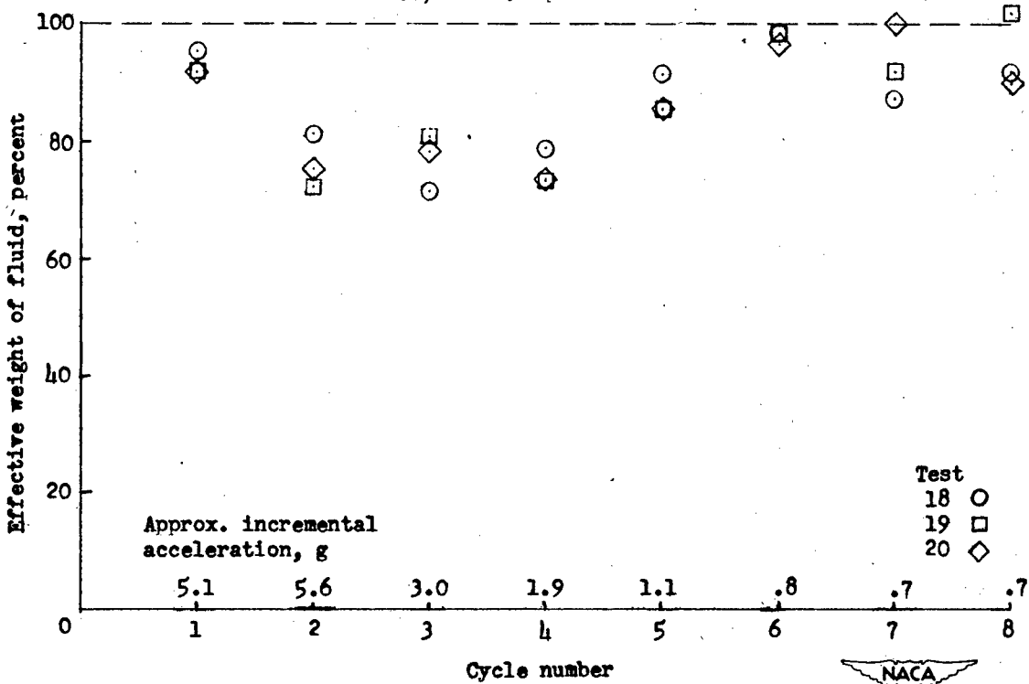
(f) Tank 60 percent full.
