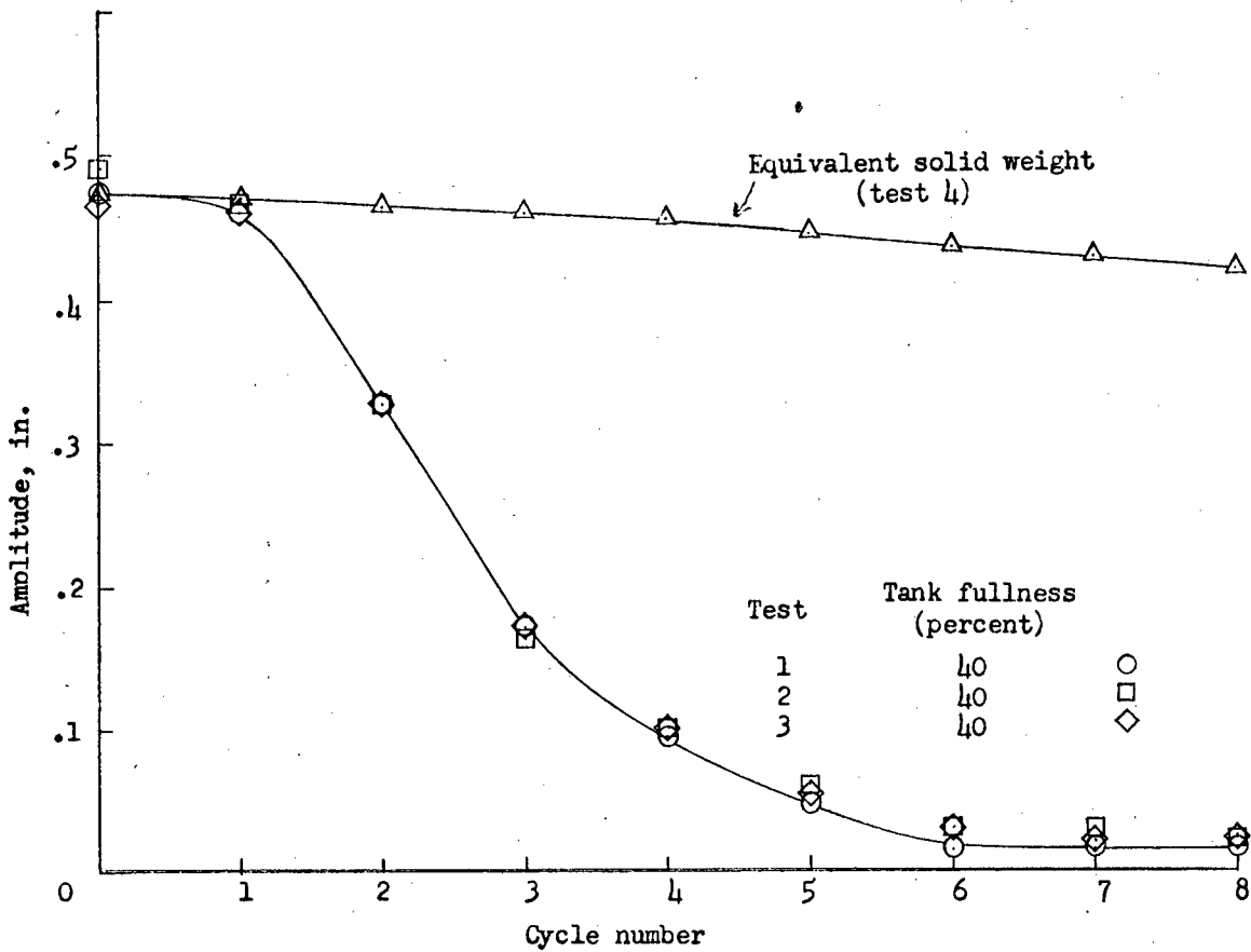
(a) Envelope curves for partly filled tank and equivalent solid weight.
