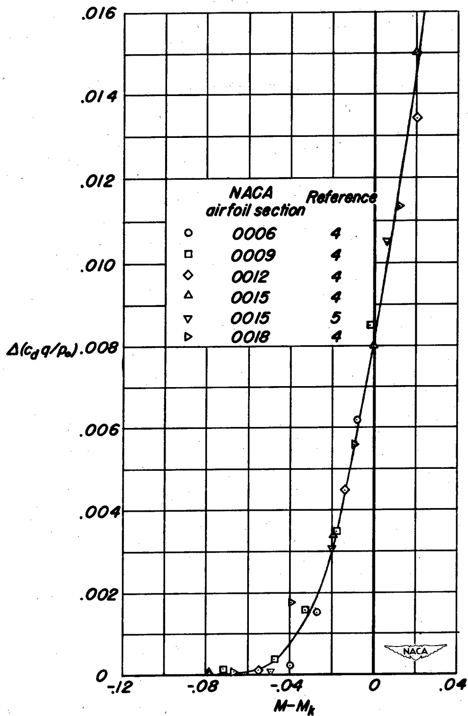
Figure 2. - Correlation of pressure-drag coefficient for several NACA 4-digit series airfoil sections. Angle of attack, 0^\circ .
