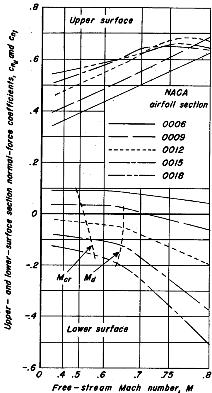
Figure 10.— Variation with free-stream Mach number of upper- and lower-surface normal-force coefficients for several NACA OOX airfoil sections at 4° angle of attack.
