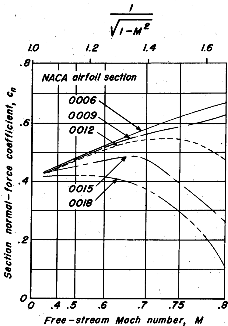
Figure 9.— Variation with free-stream Mach number of section normal-force coefficient for several NACA OOX airfoil sections at 4° angle of attack.
