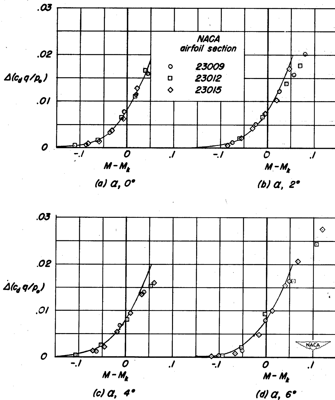
Figure 8.- Correlation of pressure-drag coefficient for several NACA 230-series airfoil sections at various angles of attack.
