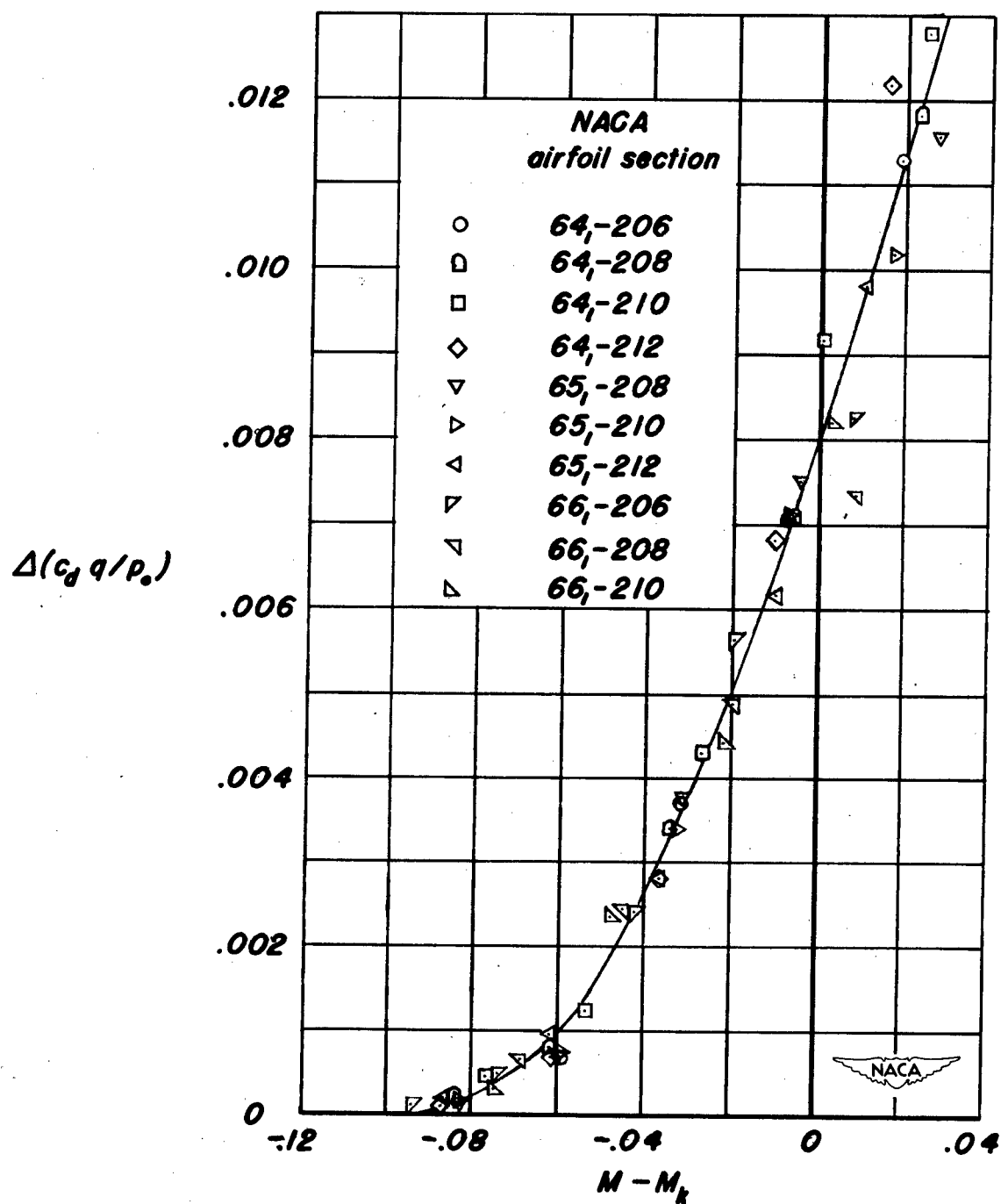
Figure 5.- Correlation of pressure-drag coefficient for several NACA 6-series airfoil sections. Angle of attack, 0^\circ .
