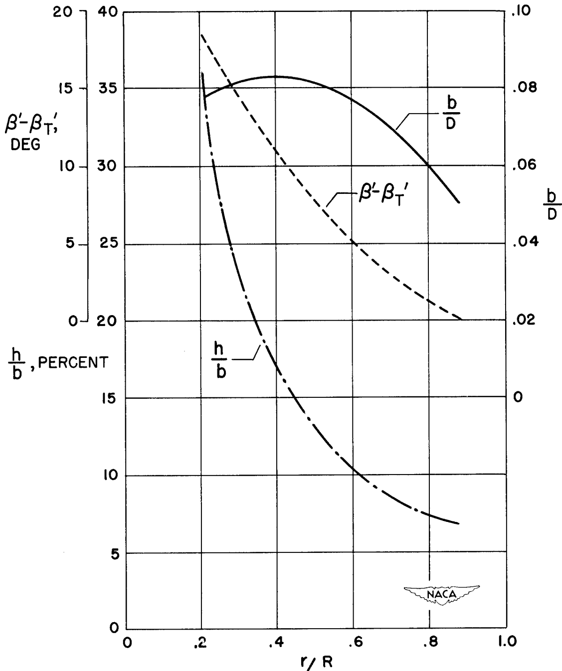
Figure 9.- Blade-form curves for Aeromatic propeller (see table I). D , diameter of propeller; R , tip radius; r , radius of element; b , width (chord) of element; h , maximum thickness of element; \beta' , pitch angle of element; \beta_T' , pitch angle of tip element.
