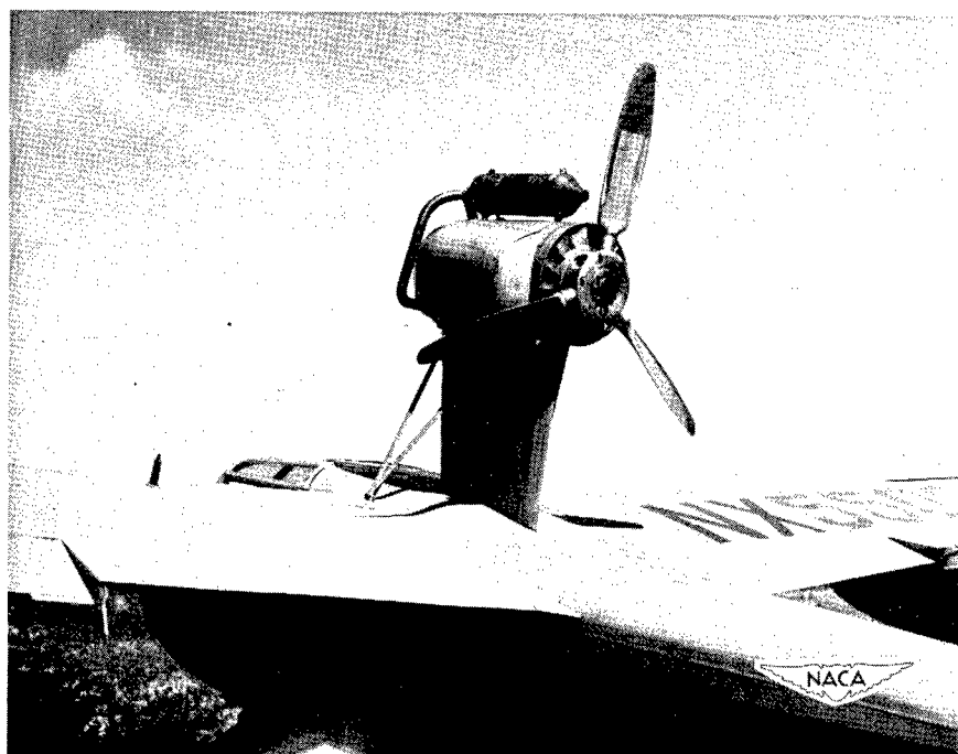
Figure 2.- Modified pusher with geared engine, muffler, and three-bladed propeller, configuration 9A.
