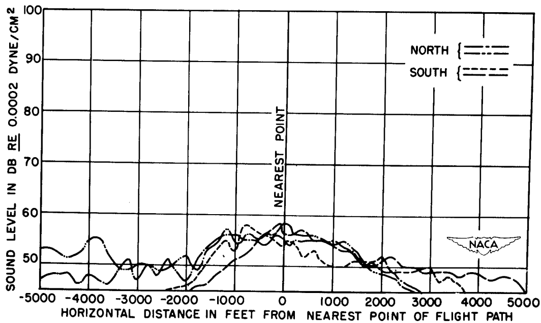
(d) Configuration 5 - standard tractor, two-bladed propeller. 2450 rpm; wind - 0 mph.
