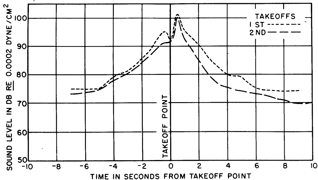
Configuration 9D; 2500 rpm.
