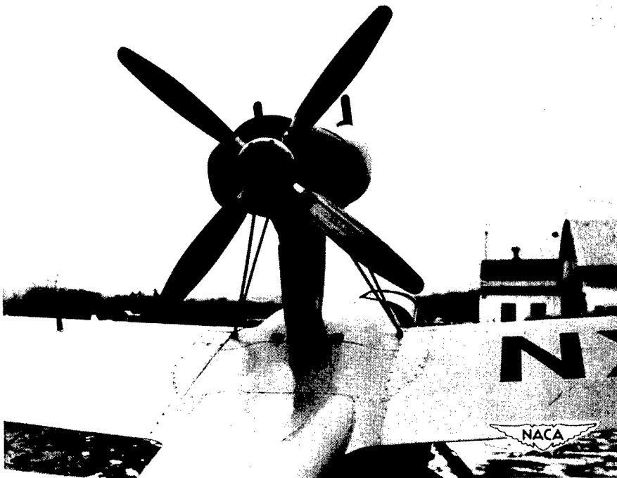
Figure 3.- Modified pusher, unmuffled, with four-bladed propeller, configuration 8.
