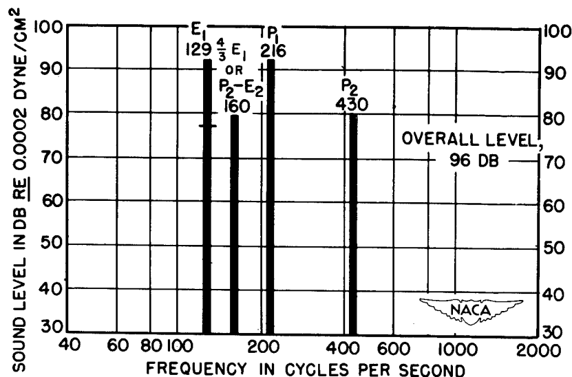
(a) Ground analysis. \theta = 120^\circ left of nose; s = 50 feet.
