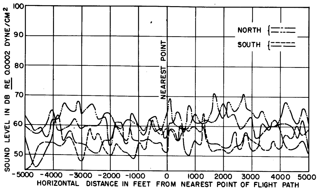
(a) Configuration 6 - standard pusher, Aeromatic propeller. 2600 rpm; wind - west, 3 mph.
