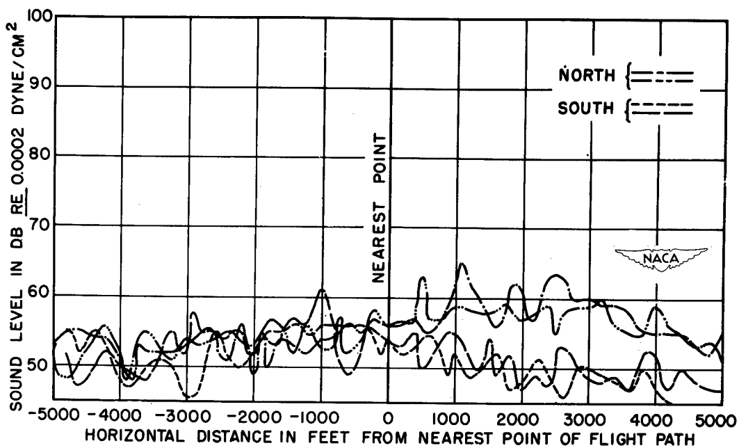
(b) Configuration 8 - modified pusher, unmuffled, four-bladed propeller. 2500 rpm; wind - west, 2 mph.
