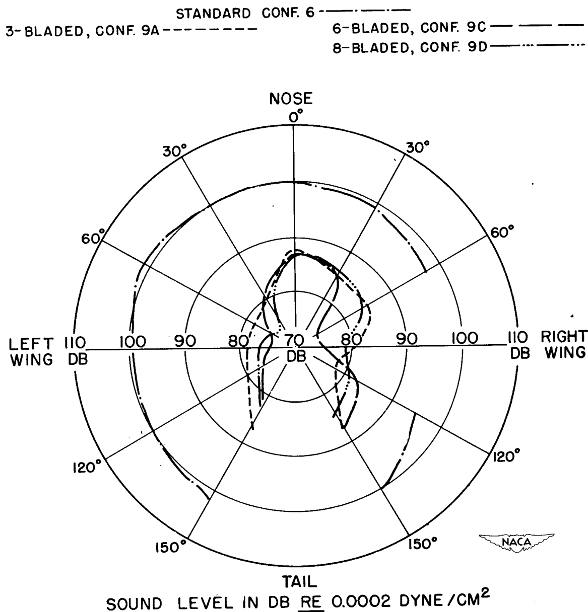
Figure 29.- Comparison of engine fundamentals for configurations of series A from frequency analysis on ground 50 feet from hub. Flat weighting. Fundamental for configuration 6 not measurable at 90° right position; fundamental for configuration 9B masked by propeller. Refer to table II for engine powers, tip speeds, and propeller diameters. RE indicates "referred to a level of."
