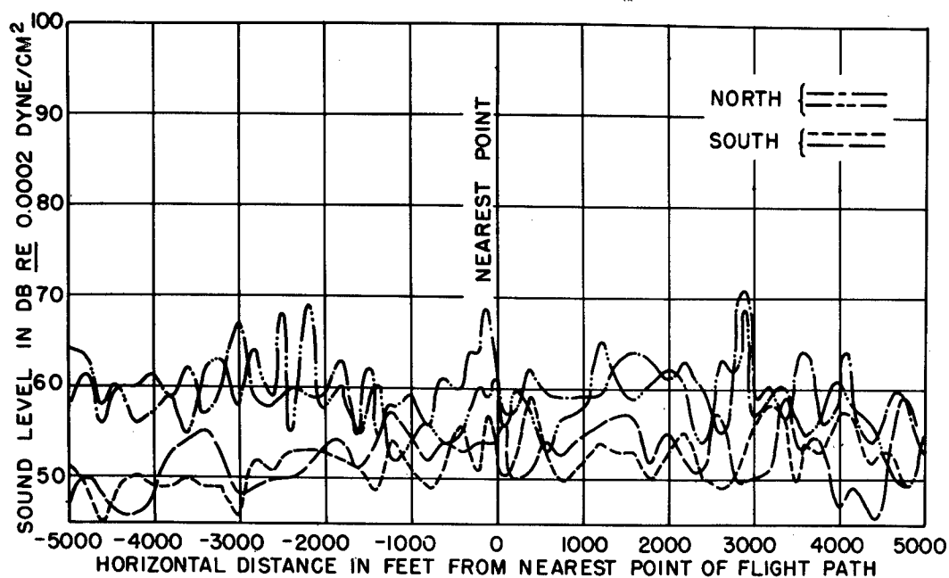
(a) Configuration 6 - standard pusher, Aeromatic propeller. 2450 rpm; wind - west, 3 mph.
