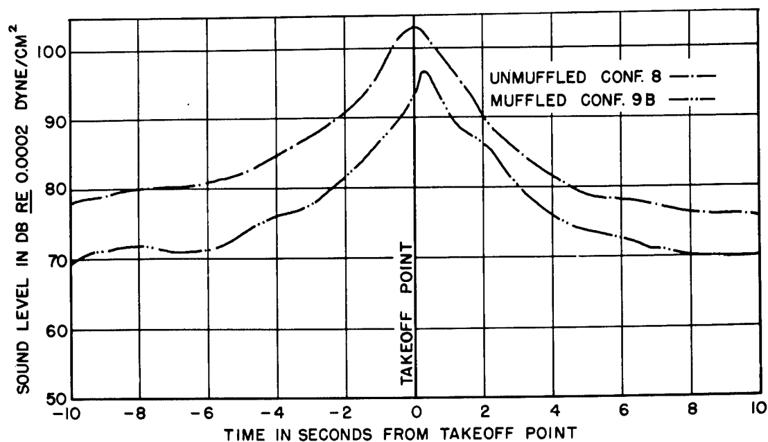
(a) Averages of take-offs. Flat weighting; airplane leaving ground as it passes 50 feet from microphone.
