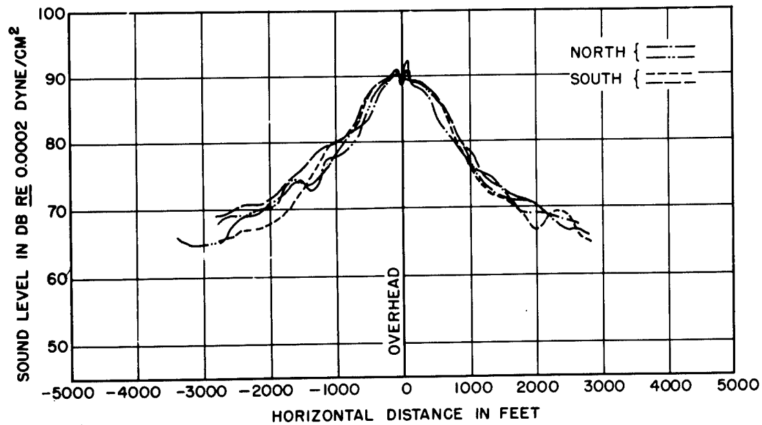
Configuration 8; 2250 rpm; wind - west, 1 mph.
