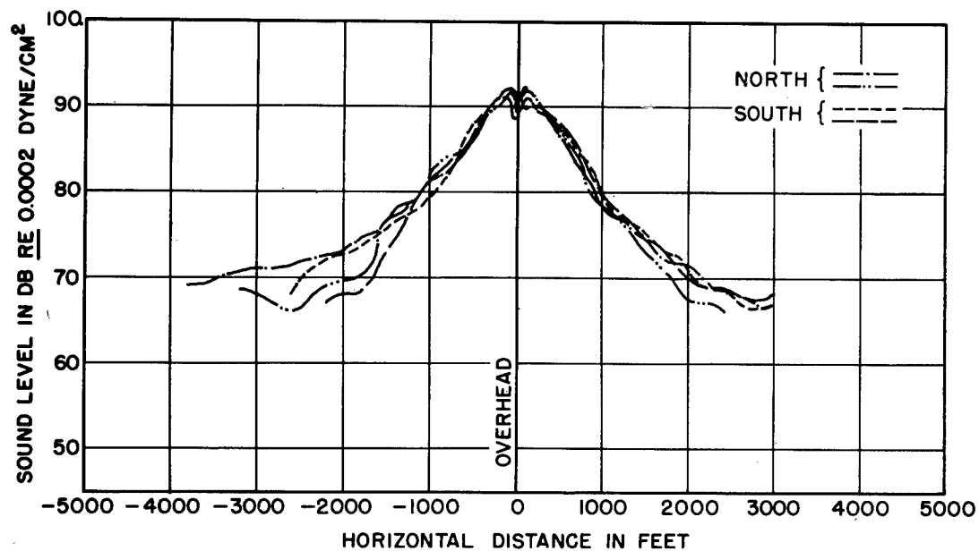
Configuration 8; 2500 rpm; wind - west, 1 mph.
