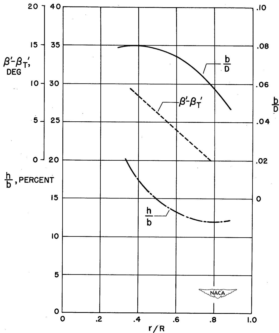
Figure 10.- Blade-form curves for fixed-pitch, solid, four-bladed propeller (see table I). D , diameter of propeller; R , tip radius; r , radius of element; b , width (chord) of element; h , maximum thickness of element; \beta' , pitch angle of element; \beta_T' , pitch angle of tip element.
