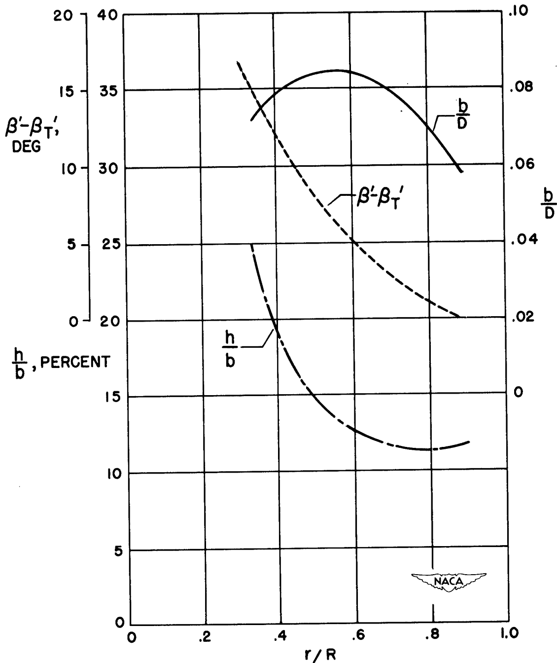
Figure 11.- Blade-form curves for medium-bladed propeller (see table I).
