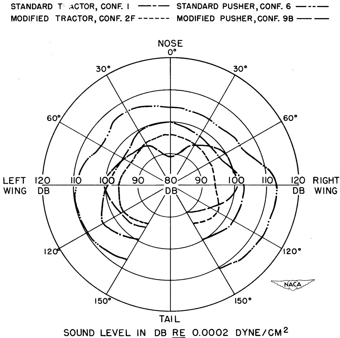
Figure 49.- Comparison of over-all levels from frequency analysis on ground 50 feet from hub for standard and modified configurations of series F. Flat weighting. Refer to table II for engine powers, tip speeds, and propeller diameters. RE indicates "referred to a level of."
