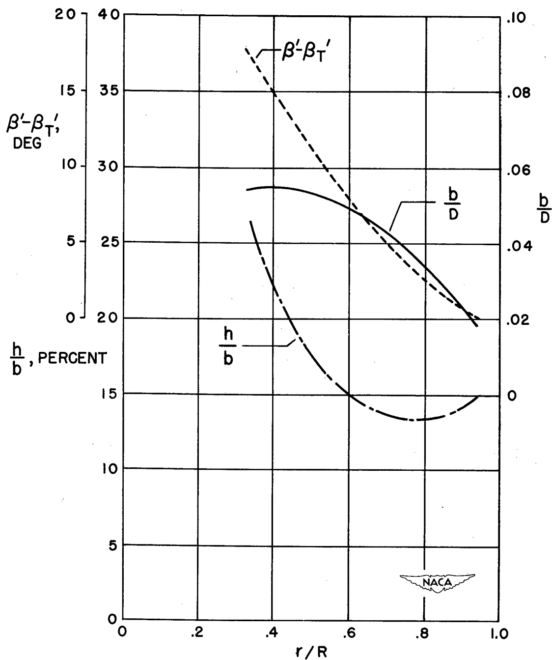
Figure 12.- Blade-form curves for thin-bladed propeller (see table I).
