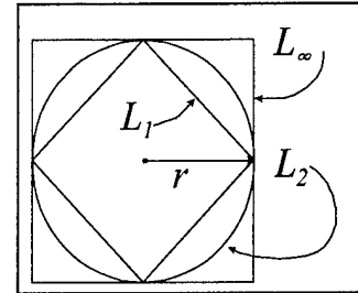
Figure 4 - The shapes of L_\infty , L_1 and L_2 norms in 2-d.
