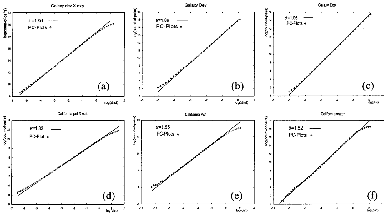
Figure 9 - PC plots and the pair-count exponents \phi of geographical data. First row: Galaxy datasets (a) cross join of 'dev' and 'exp', (b) self join of 'dev', (c) self join of 'exp'. Second row California datasets (d) cross join of CA-pol and CA-wat, (e) self join of CA-pol, (f) self join of CA-wat.
