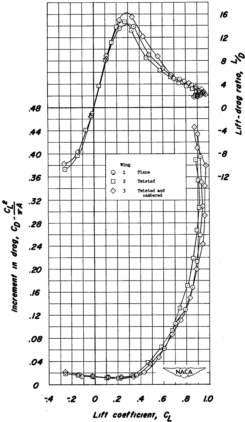
Figure 6.- Effects of twist and camber on variation of L/D and C_D - \frac{C_L^2}{\pi A} with C_L for a 45^\circ sweptback wing of aspect ratio 4 and taper ratio 0.6. Reynolds number = 0.895 \times 10^6 ; Mach number = 0.17; transition strips off.
