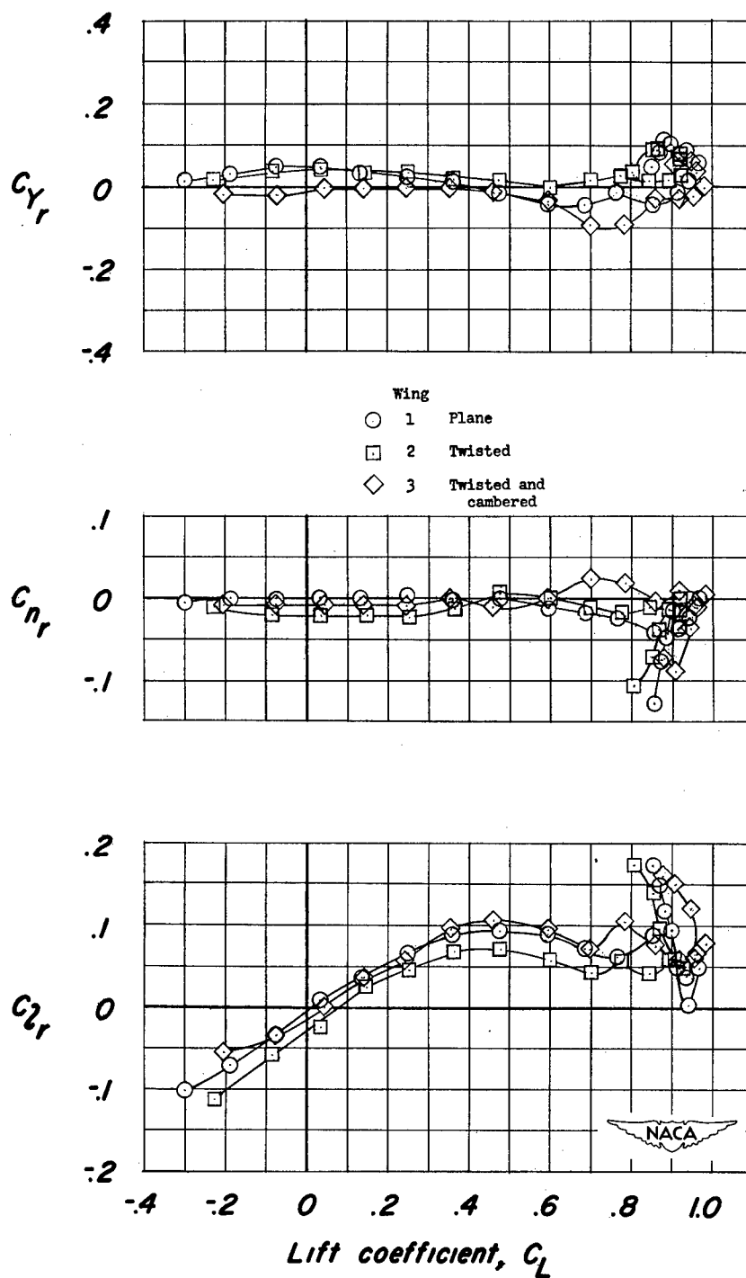
Figure 12.- Effects of twist and camber on variation of C_{Y_r} , C_{n_r} , and C_{l_r} with C_L for a 45^\circ sweptback wing of aspect ratio 4 and taper ratio 0.6. Reynolds number = 0.707 \times 10^6 ; Mach number = 0.13; transition strips off.
