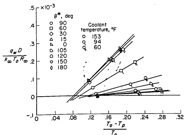
FIGURE 2.—Variation of heat-transfer parameter with wall-temperature parameter at station 2 for typical runs. \Delta = 60^\circ ; T_o \approx 250^\circ \text{ F} ; R_\infty \approx 1.4 \times 10^6 .
