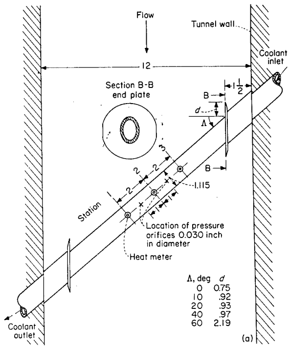
(a) Model installation.
