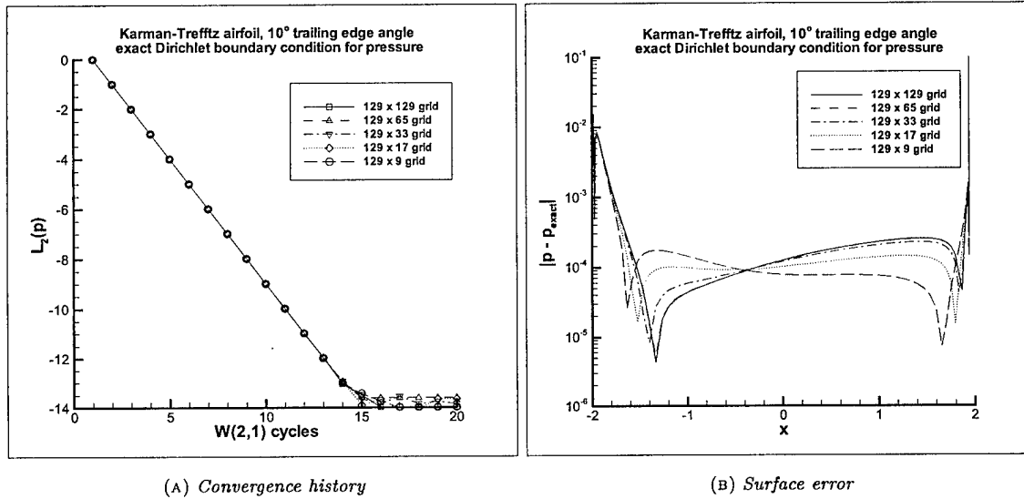
FIG. 3.4. Computation of the flow past an airfoil using exact ABCs.
