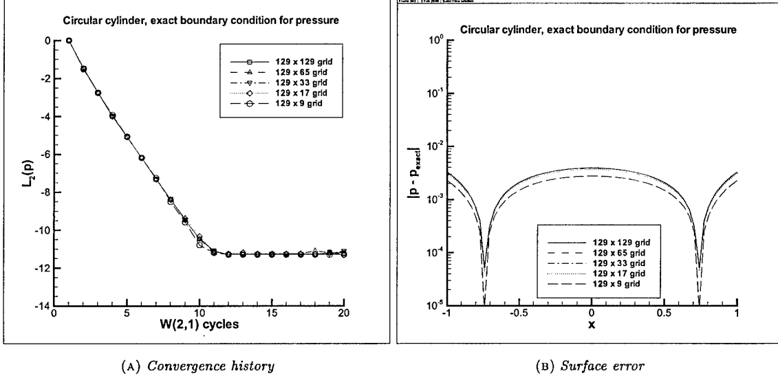
FIG. 3.1. Computation of the flow past a circular cylinder using exact ABCs.
