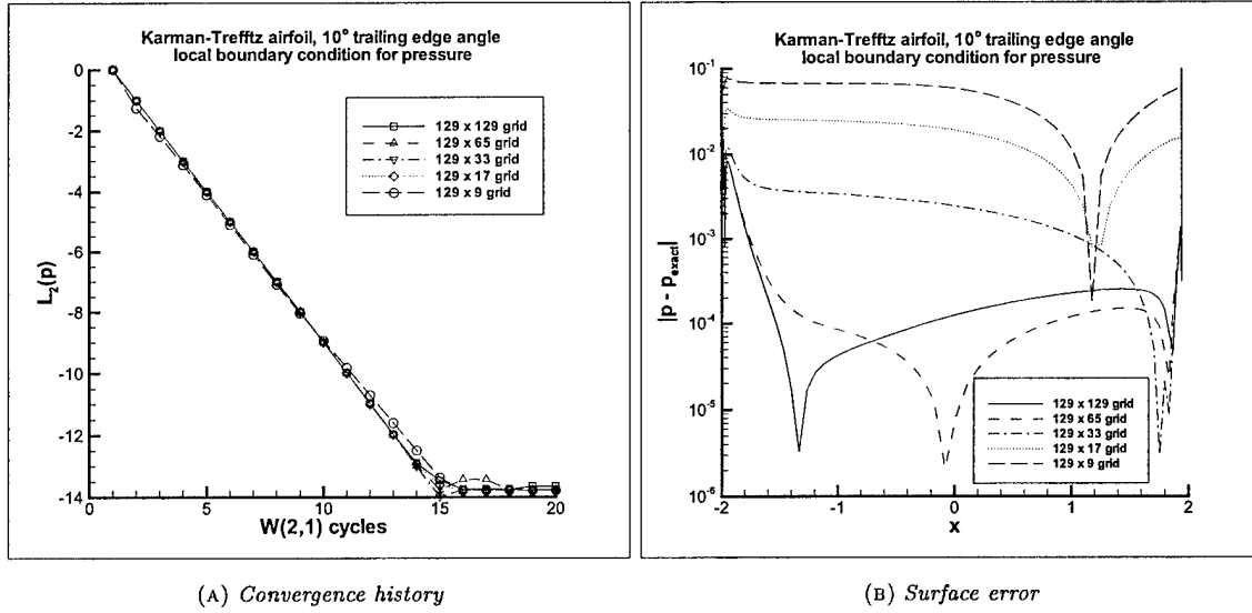
FIG. 3.6. Computation of the flow past an airfoil using local ABCs.
