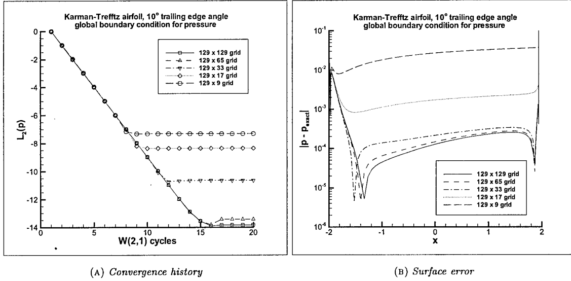
FIG. 3.5. Computation of the flow past an airfoil using global ABCs.
