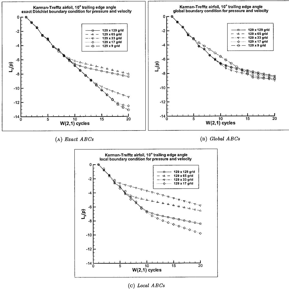
FIG. 3.7. Convergence histories for the flow past an airfoil computed in the framework of the full Euler equations.
