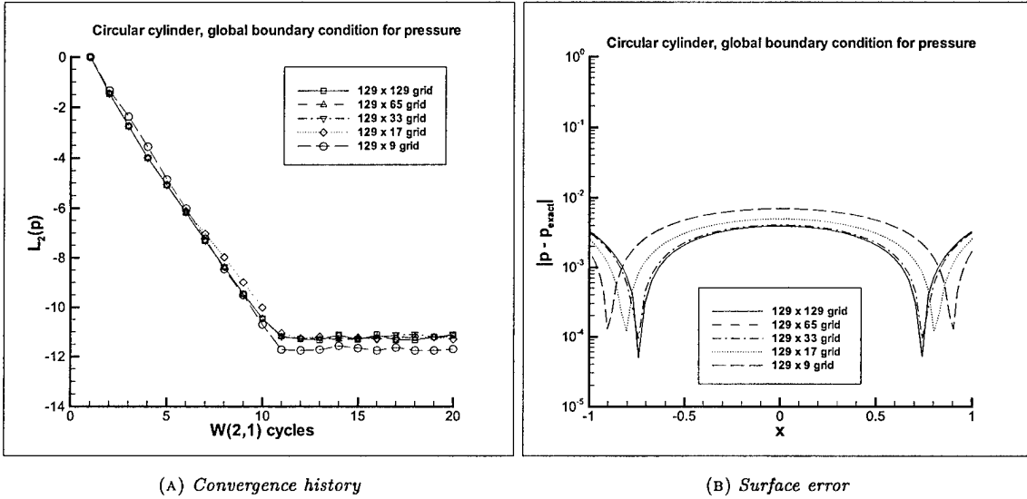
FIG. 3.2. Computation of the flow past a circular cylinder using global ABCs.
