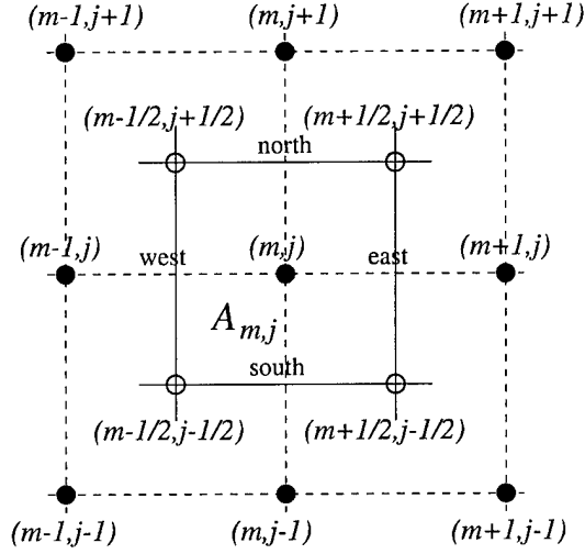
FIG. 2.1. Computational grid segment and a control volume.
