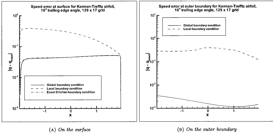
FIG. 3.10. Velocity error profiles for the flow past an airfoil computed in the framework of the full Euler equations on the 129 \times 17 grid.
