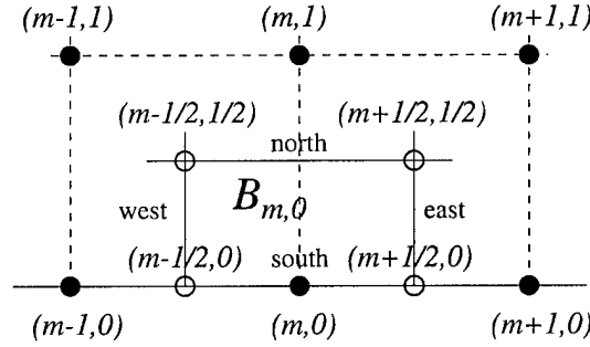
FIG. 2.2. Boundary control volume.
