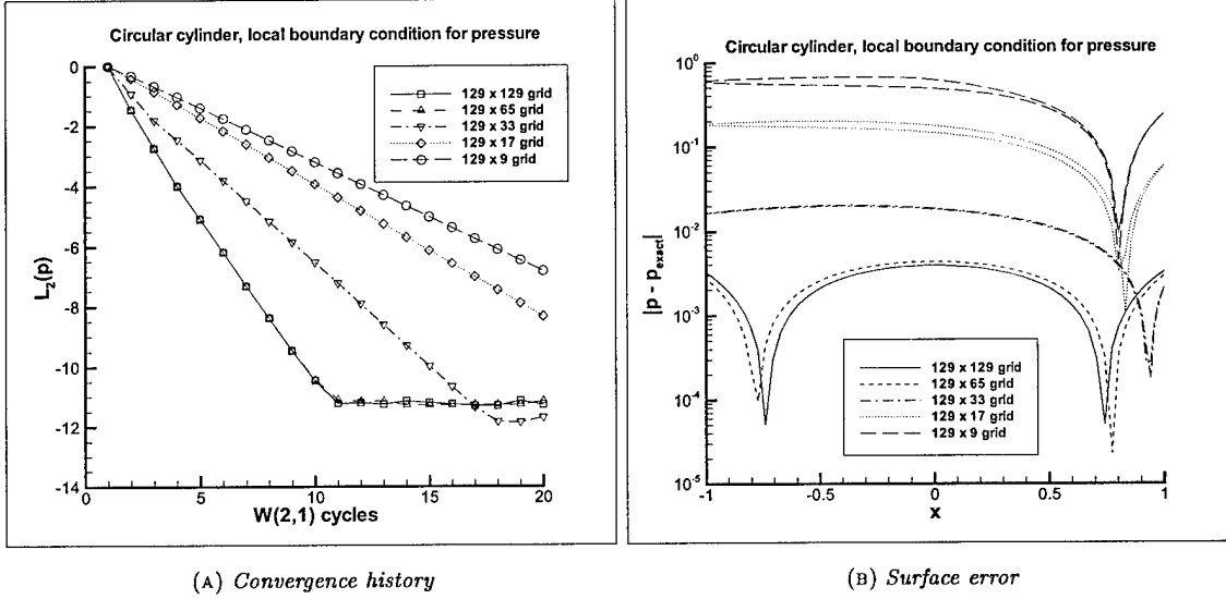
FIG. 3.3. Computation of the flow past a circular cylinder using local ABCs.
