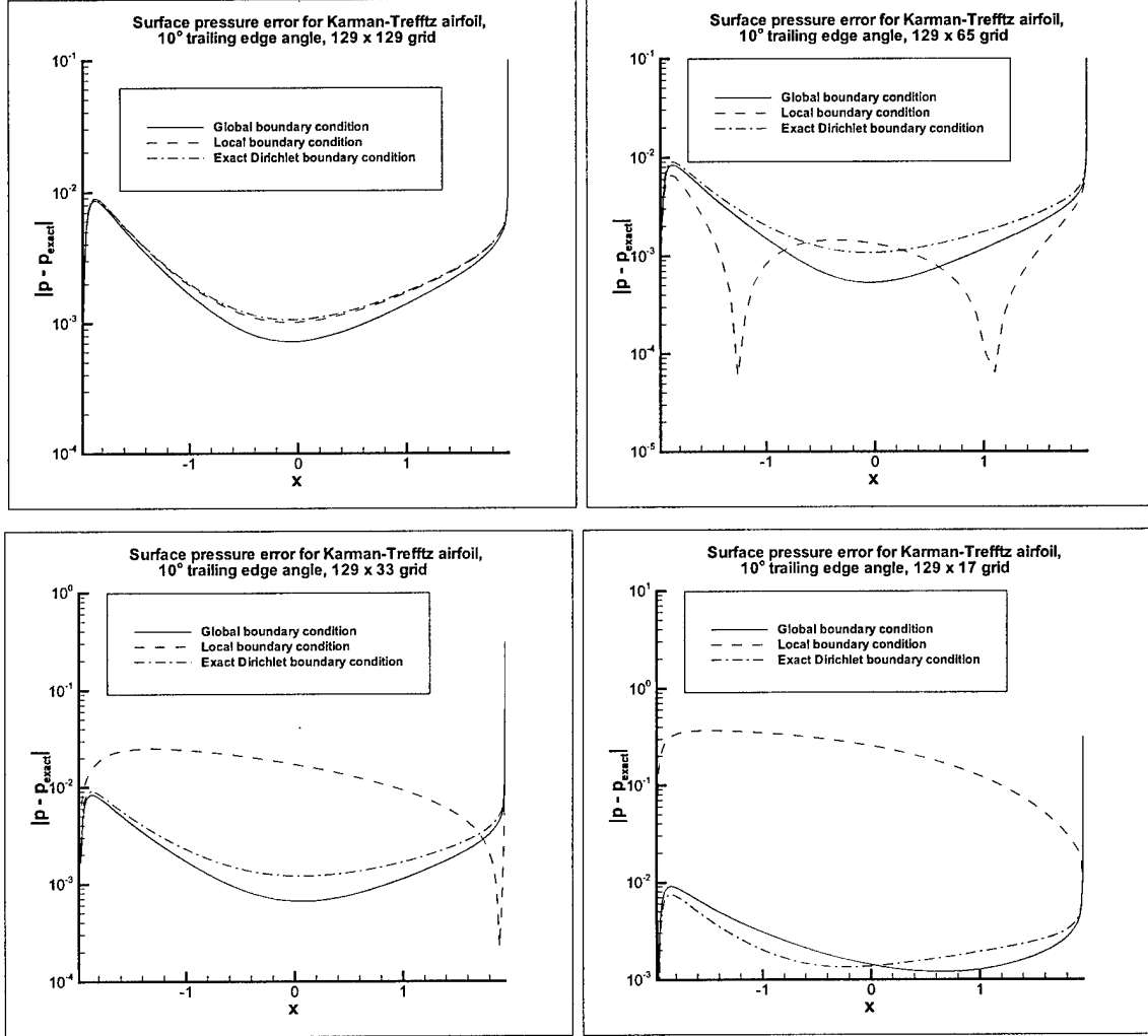
FIG. 3.8. Surface pressure error profiles for the flow past an airfoil computed in the framework of the full Euler equations.
