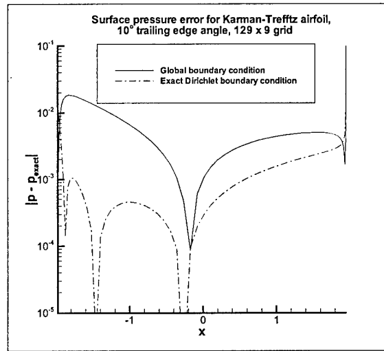
FIG. 3.9. Surface pressure error profiles for the flow past an airfoil computed in the framework of the full Euler equations.
