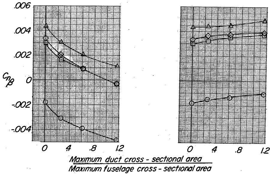
(b) Horizontal ducts on models having a wing of aspect ratio 2.
