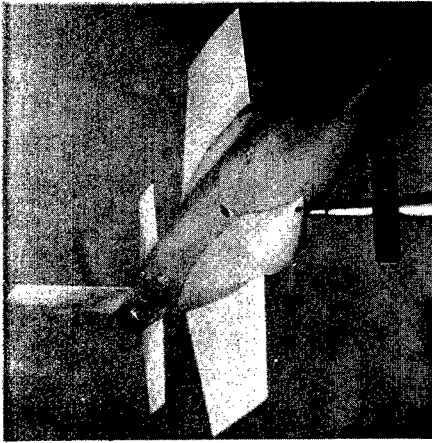
L-82955 (b) Medium ducts on configuration FW 2 VH L .
