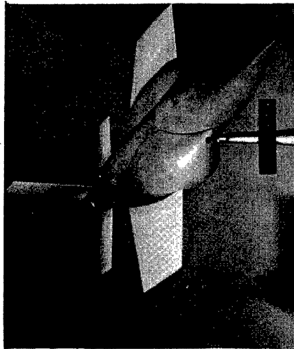
L-82967 (c) Large ducts on configuration FW 2 VH L .
