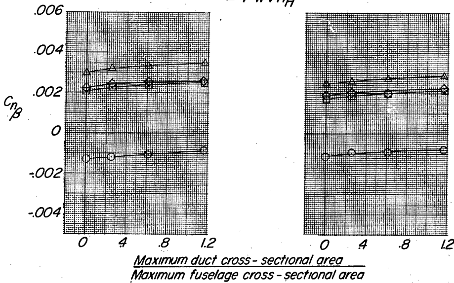
(d) Horizontal ducts on models having a wing of aspect ratio 6.
