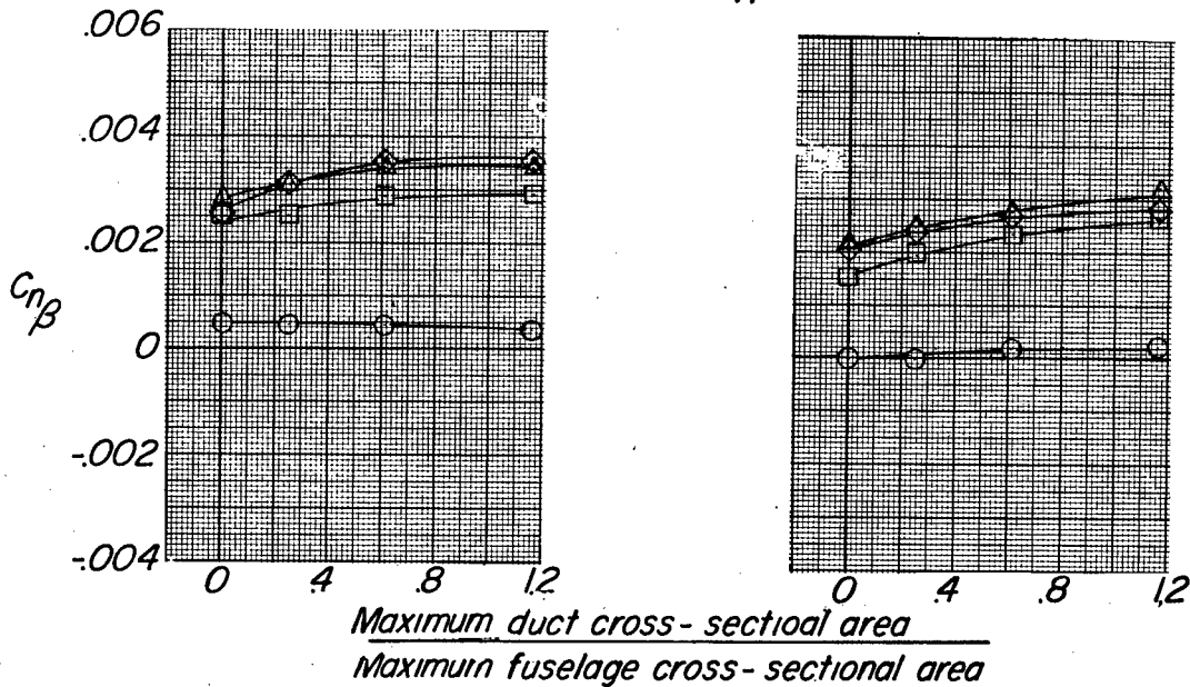
(d) Horizontal ducts on models having a wing of aspect ratio 6.
