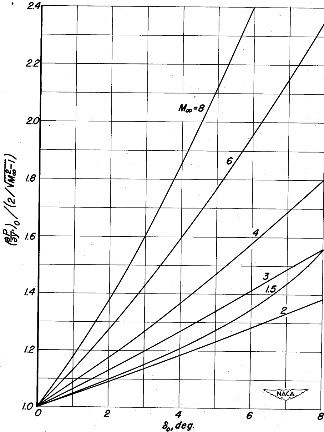
Figure 4.—Curves based on shock-expansion theory showing \frac{(pP/\rho)_0}{2\sqrt{M_\infty^2-1}} as a function of leading-edge deflection angle for various Mach numbers.
