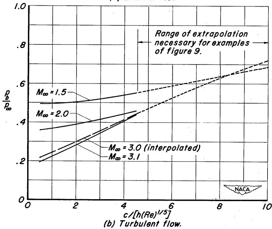
Figure 8.- Average experimental values of base pressure from reference 6.
