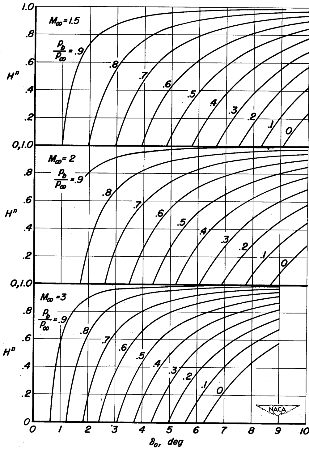
(a) M_\infty = 1.5, 2, 3
