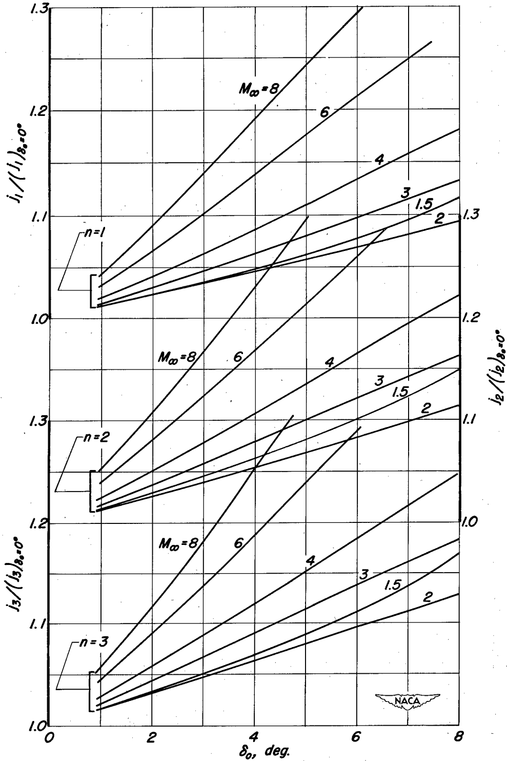
Figure 5.—Curves based on shock-expansion theory showing i_n / (i_n)_{\delta_0=0^\circ} as a function of leading-edge deflection angle for various Mach numbers.
