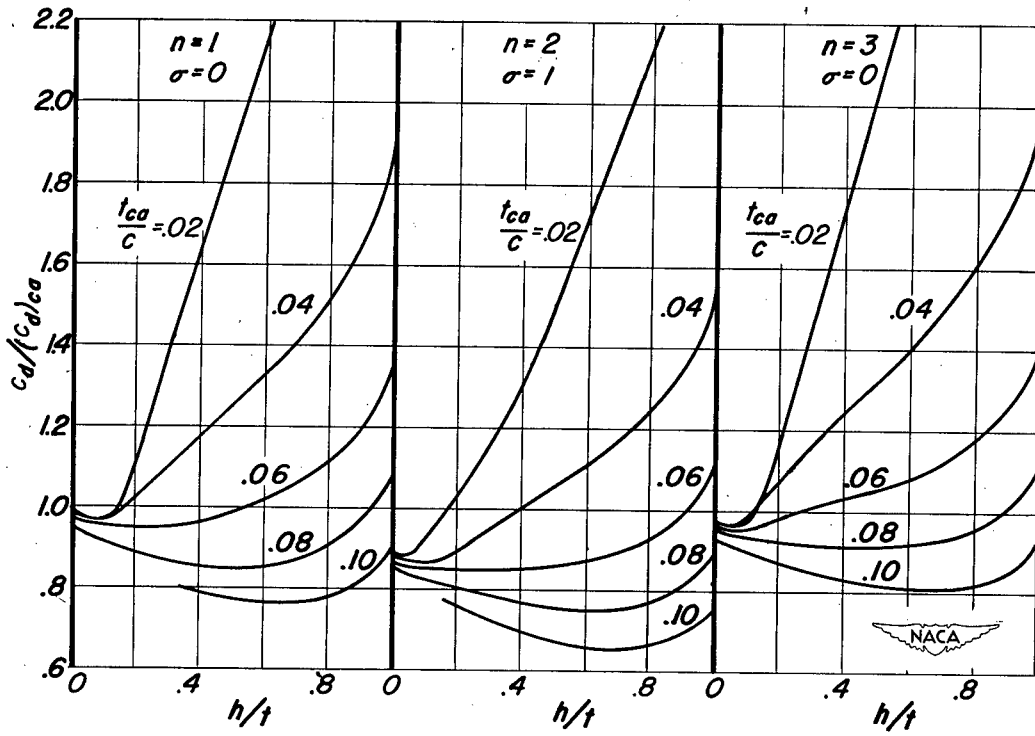
Figure 12.-Effect of trailing-edge bluntness on the relative pressure drag of semioptimum profiles compared to a structurally equivalent circular-arc biconvex profile.
