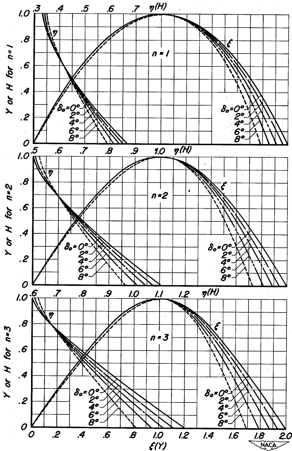
(a) M_\infty = 1.5
