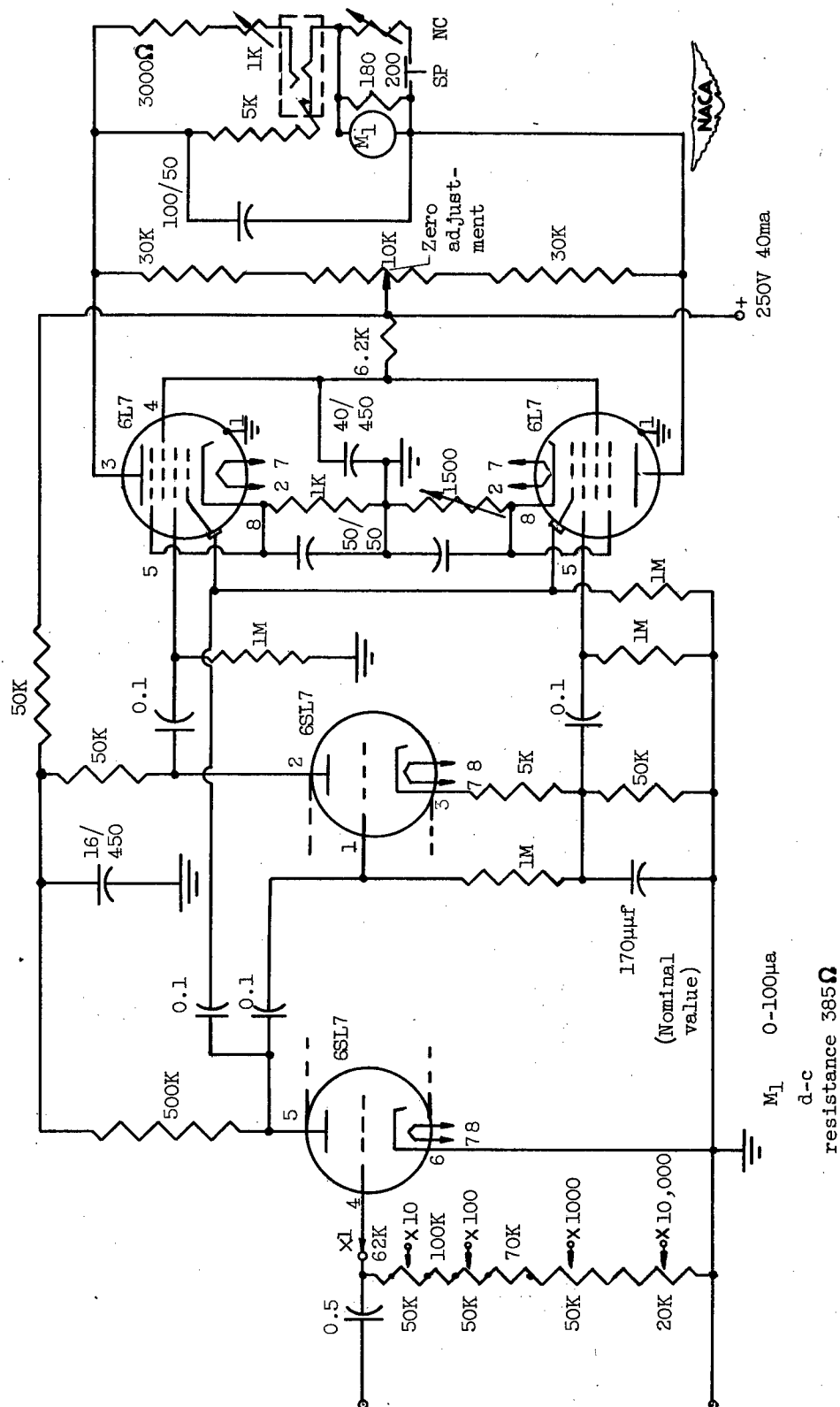
Figure 10. - Average-square computer circuit.
