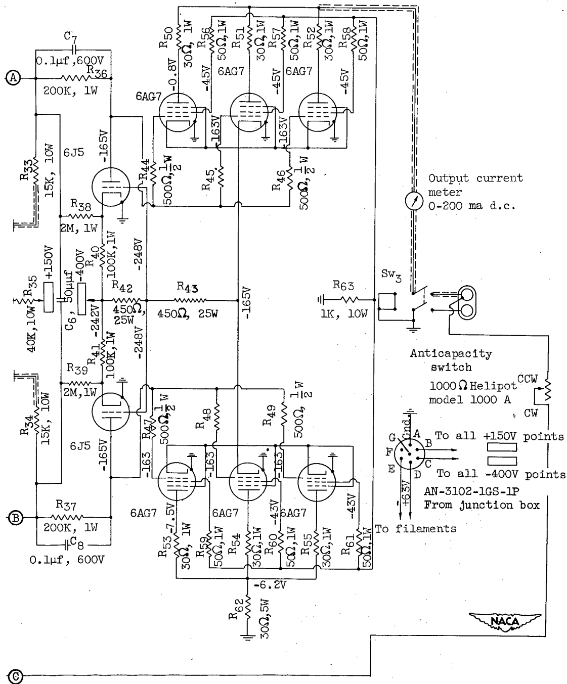
Figure 2. - Hot-wire anemometer with d-c amplifier.
