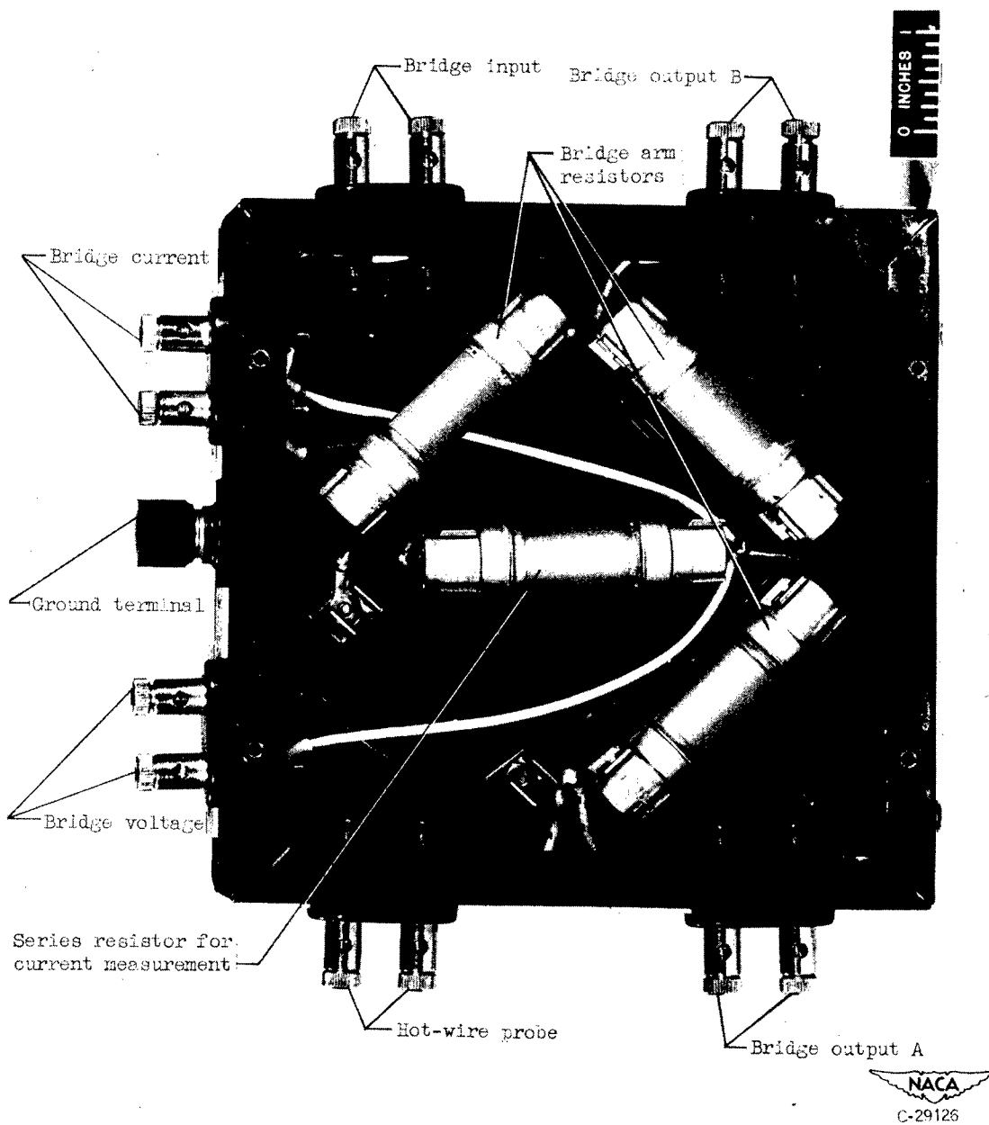
Figure 5. - Hot-wire bridge.
