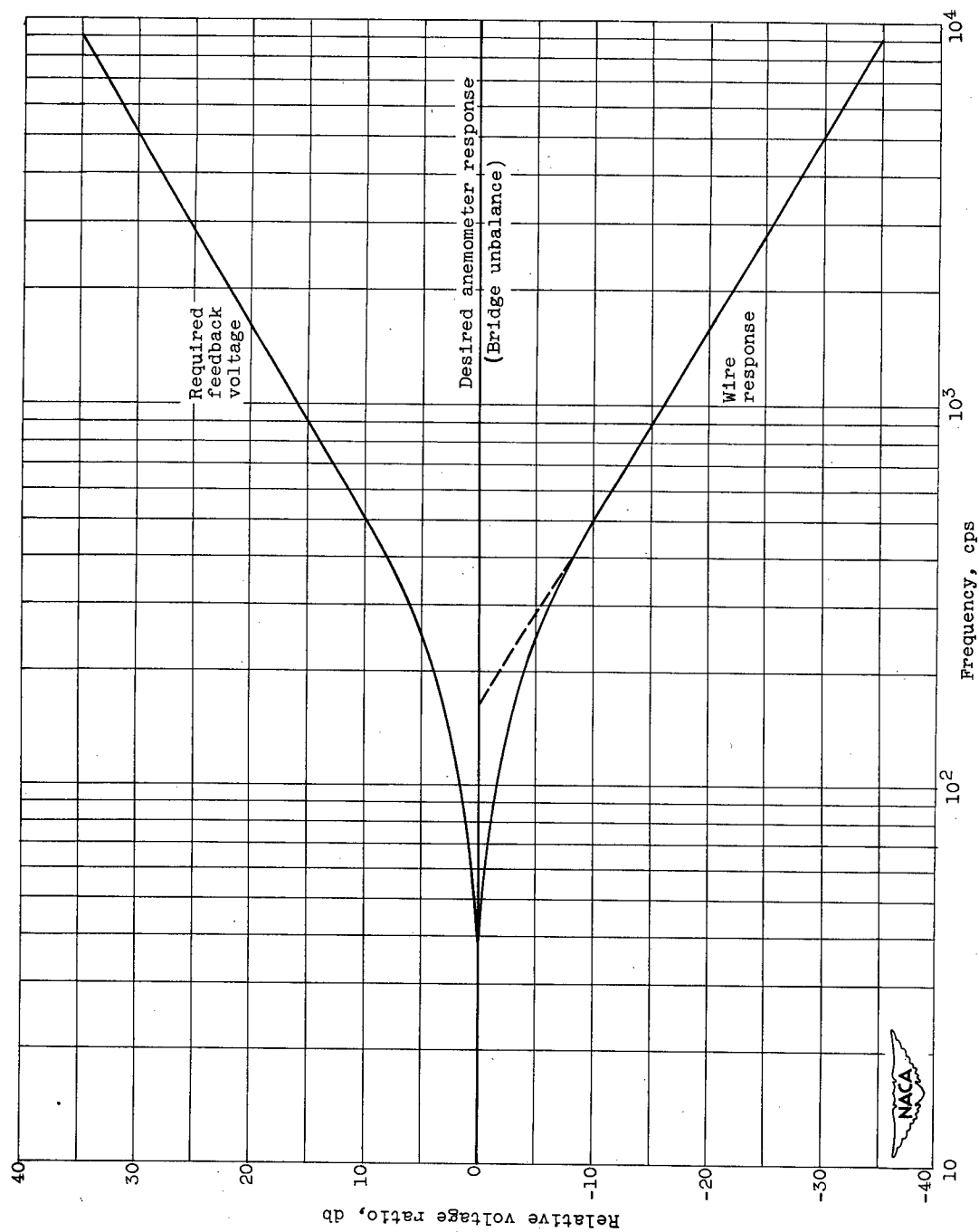
Figure 4. - Theoretical frequency response.
