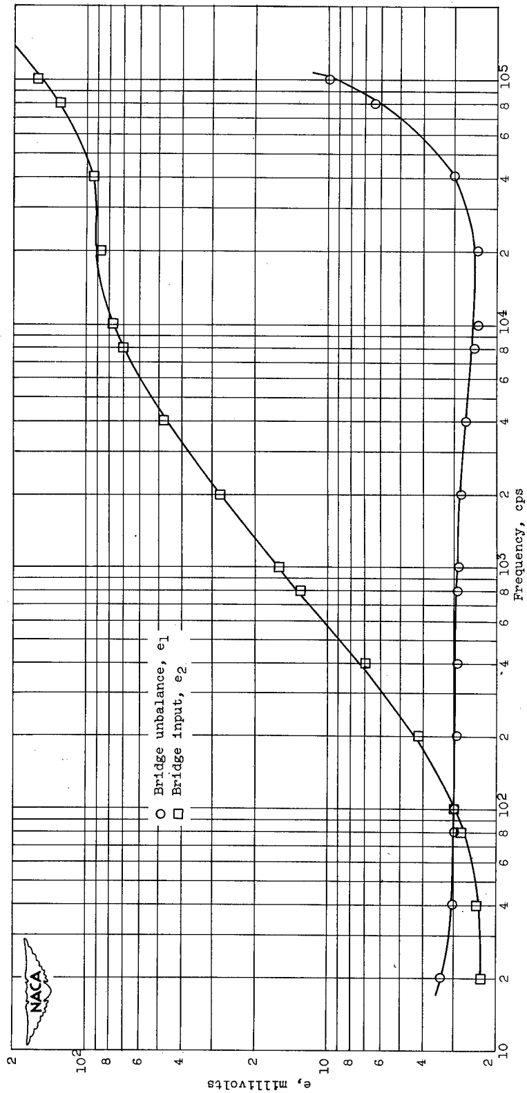
Figure 8. - Response curves of constant-temperature hot-wire anemometer; wire diameter, 0.0002 inch; length, 0.080 inch.
