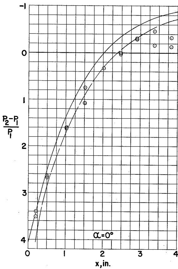
Figure 12.— A comparison between the theoretical and experimental pressure distribution over a circular arc surface where the flow is initially at M=6.86 and R_e=0.98 \times 10^6 .
