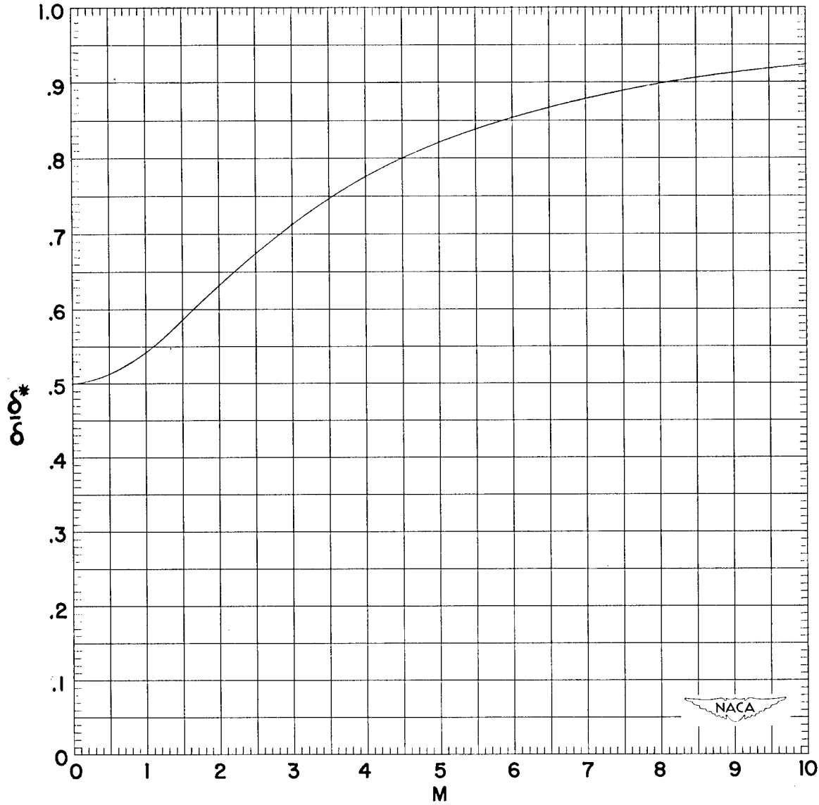
Figure 1.—Ratio of boundary-layer displacement thickness to total thickness as a function of the Mach number at the edge of the boundary layer where the velocity distribution across the boundary layer is linear.
