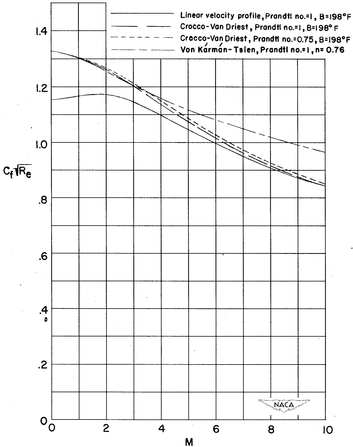
Figure 6.—Comparison of skin-friction coefficients for an insulated flat plate computed from several theories for a free-stream temperature of -67.6° F.
