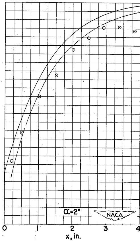
Figure 12.— A comparison between the theoretical and experimental pressure distribution over a circular arc surface where the flow is initially at M=6.86 and R_e=0.98 \times 10^6 .
