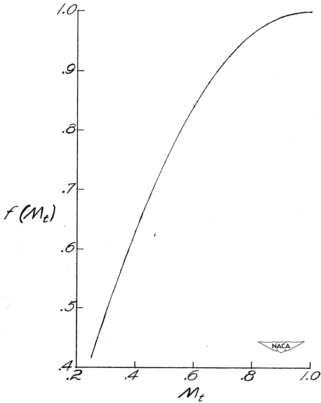
Figure 7.- Variation of Mach number function with Mach number.
