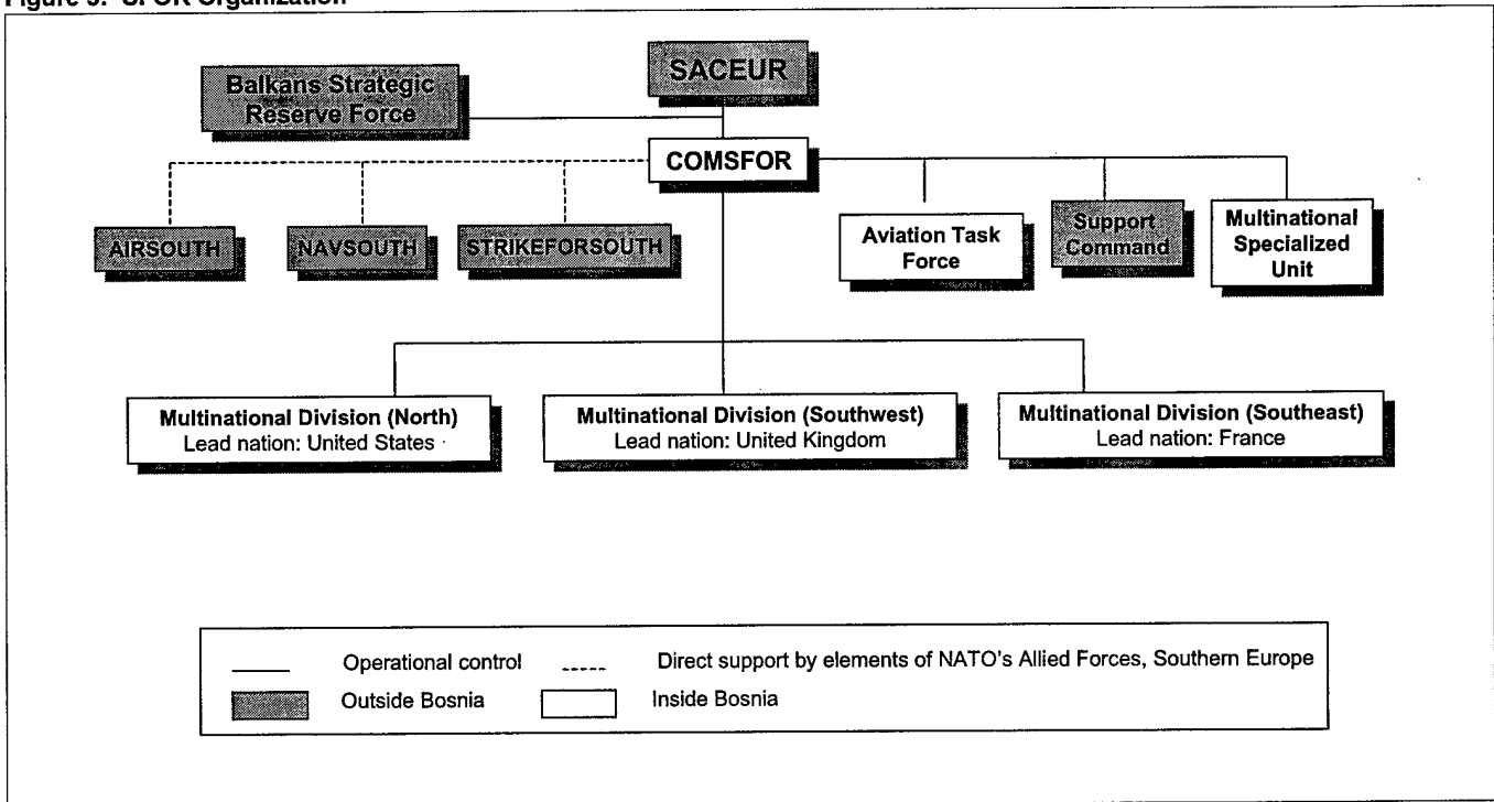
Figure 5: SFOR Organization
