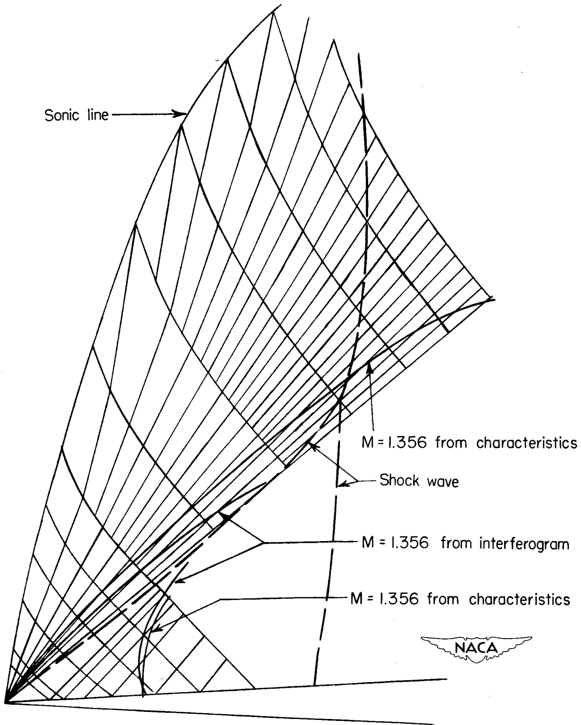
Figure 6.- Characteristic network for flow about leading edge of wedge. \alpha = 5.5^\circ ; M_0 = 0.894 .
