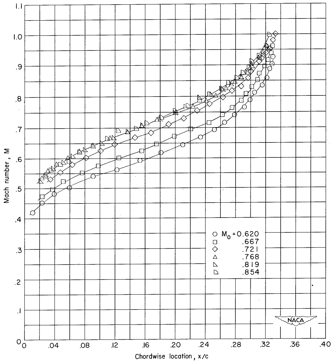
Figure 10.- Mach number distributions on surface of hexagon between leading edge and first corner. ( 14.5^\circ semiangle wedge.)
