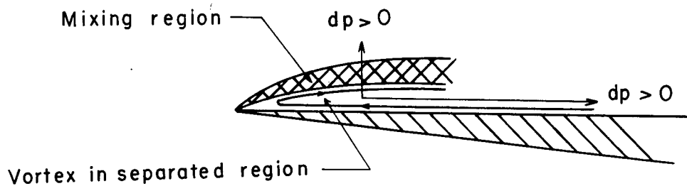
(a) Large separated region.
