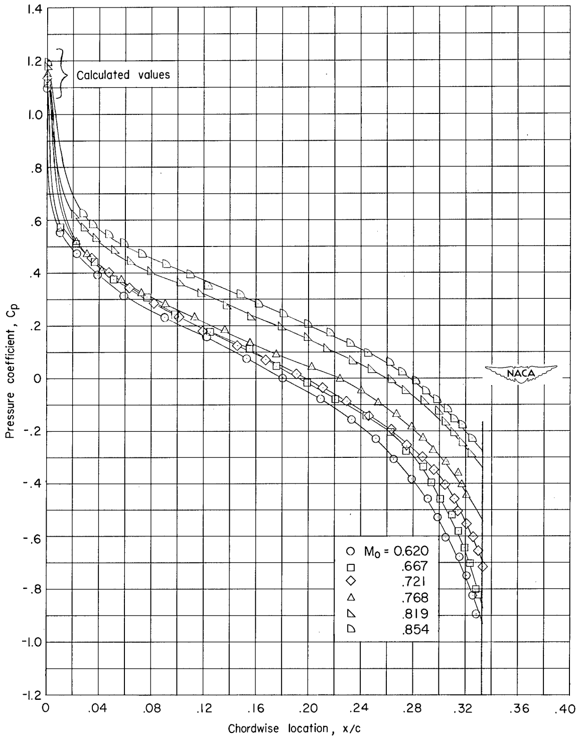
Figure 11.- Pressure distributions on surface of hexagon between leading edge and first corner. ( 14.5^\circ semiangle wedge.)
