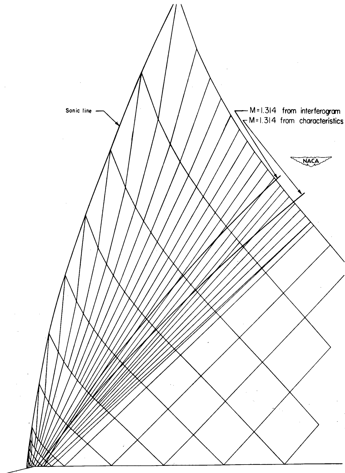
Figure 8.- Characteristic network for flow around hexagon. M_0 = 0.819 .
