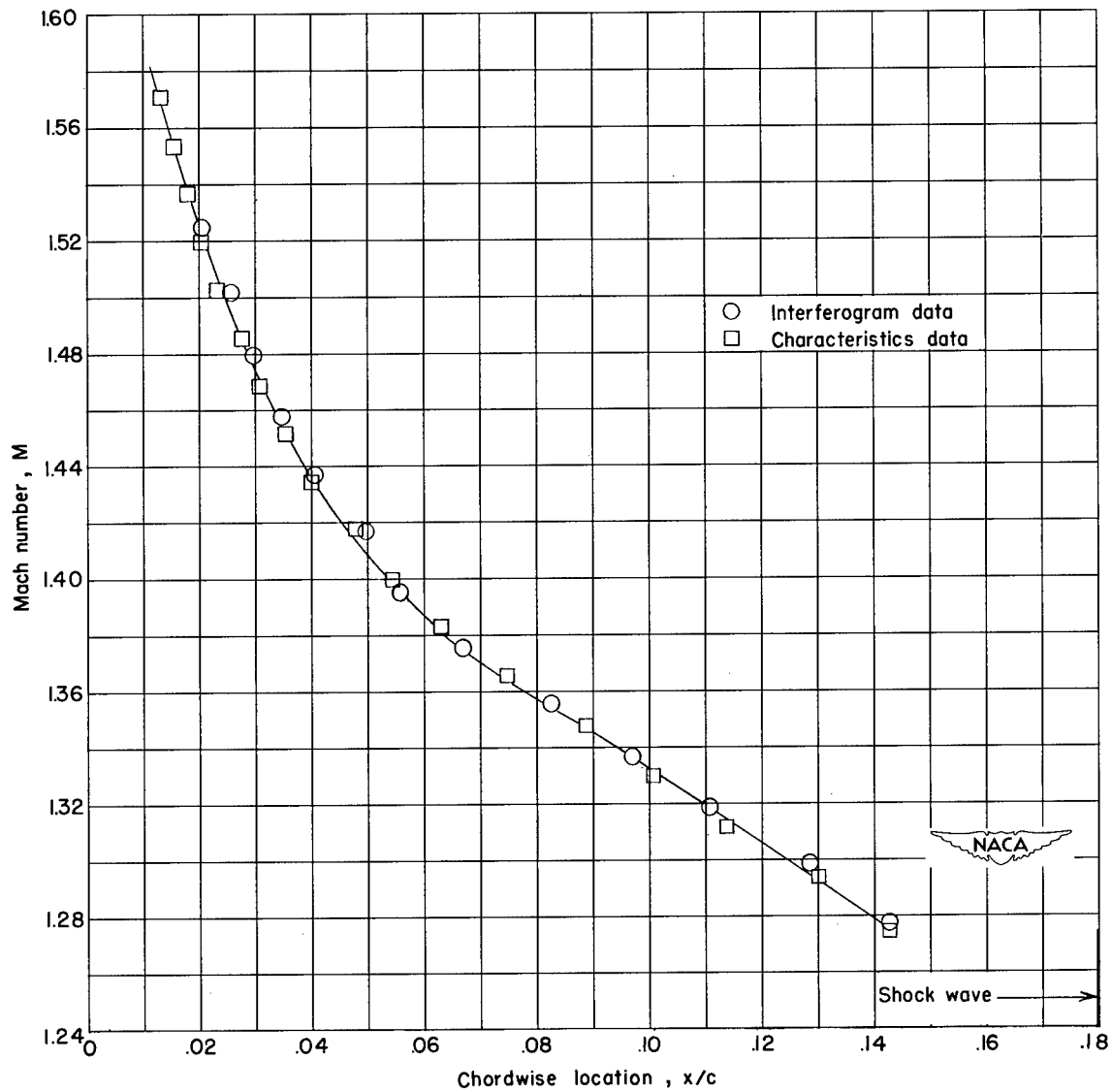
Figure 7.- Comparison of Mach number distributions on wedge surface ( \alpha = 5.5^\circ ) between the oblique shock wave and the normal shock wave. M_0 = 0.894 .
