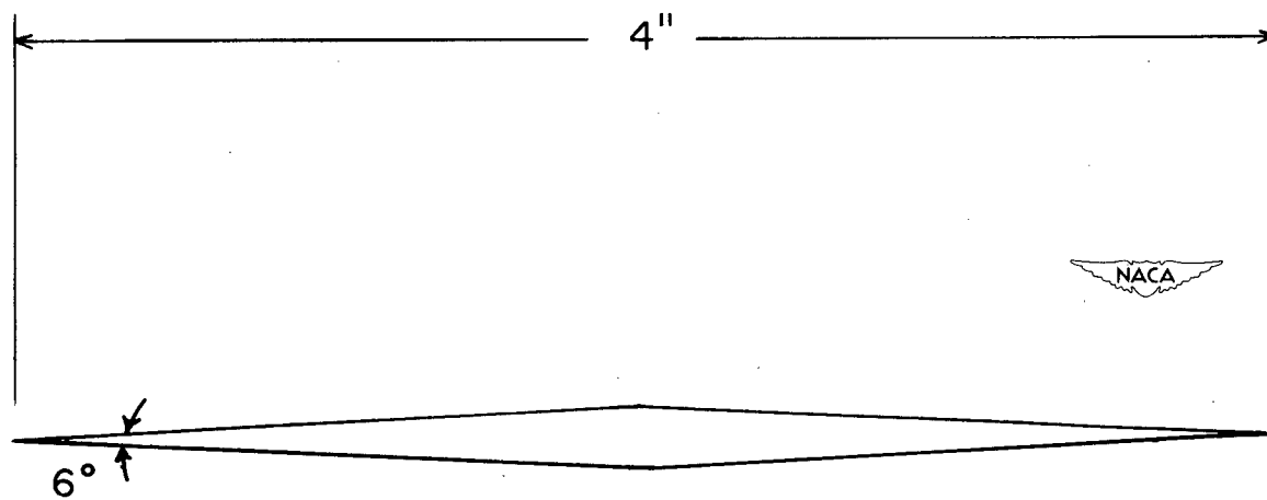
(b) Symmetrical wedge.
