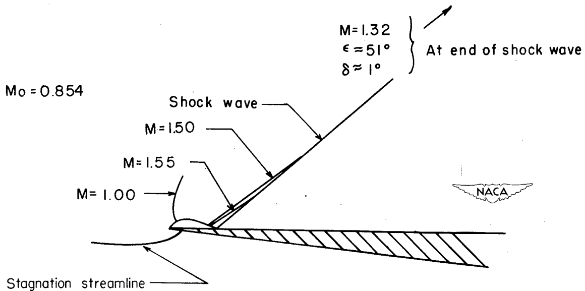
(b) Very small separated region.
