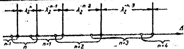
Fig. 3. Location of the regions of existence of various cycles on the axis.
