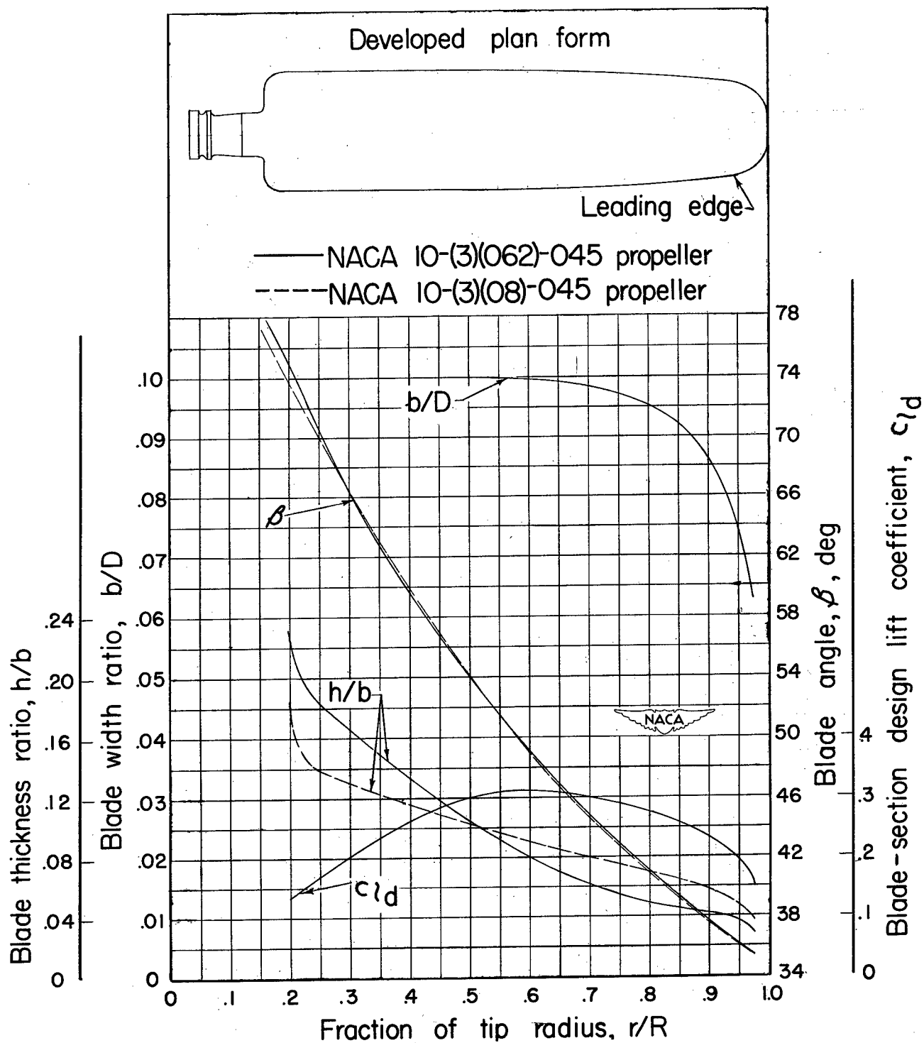
Figure 2.- Blade-form curves for NACA 10-(3)(062)-045 and for NACA 10-(3)(08)-045 propellers.
