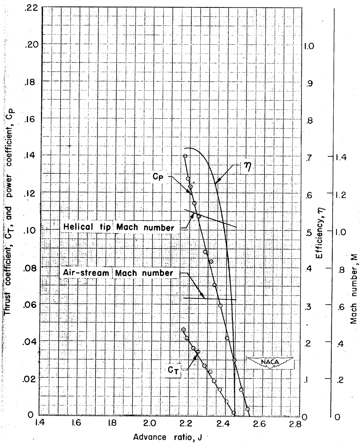
(c) Air-stream Mach number, 0.63.
