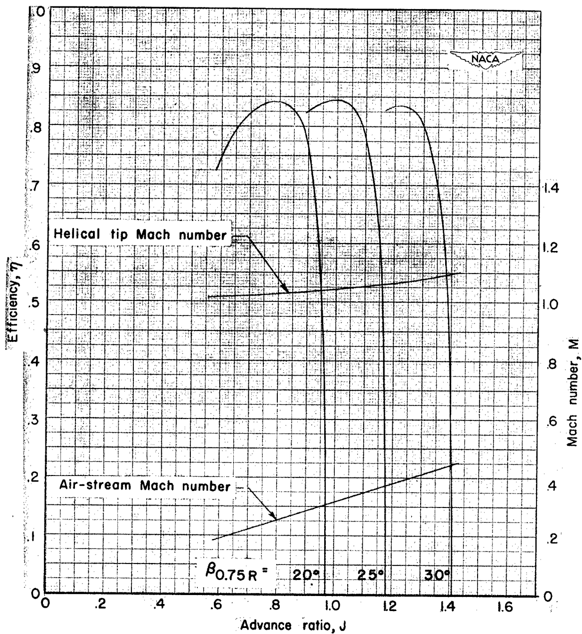
(c) Efficiency.
