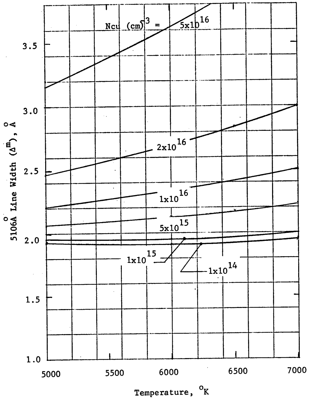
FIGURE 8. THEORETICAL WIDTH OF THE 5106 Å COPPER LINE AS A FUNCTION OF TEMPERATURE AND COPPER DENSITY ( p = 80 \text{ atm} , l = 1.27 \text{ cm} , \Delta T = 1.55 \text{ Å} )
