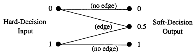
Figure 28. Erasure Channel.
