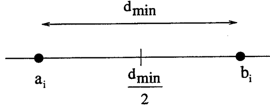
Figure 10. Bipolar Modulation.
