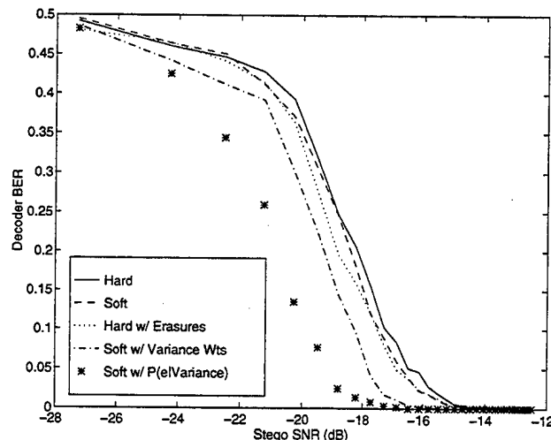
Figure 30. Comparison of Side Information Techniques.
