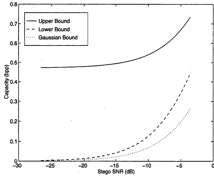
Figure 5. Generic Steganographic Channel Capacity.
