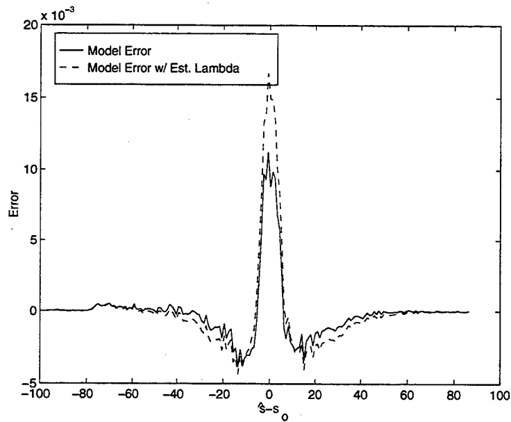
Figure 26. Laplacian Model Error.
