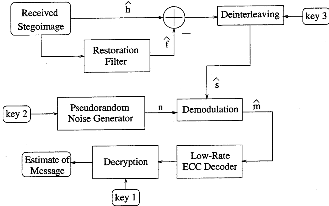
Figure 9. SSIS Decoder.
