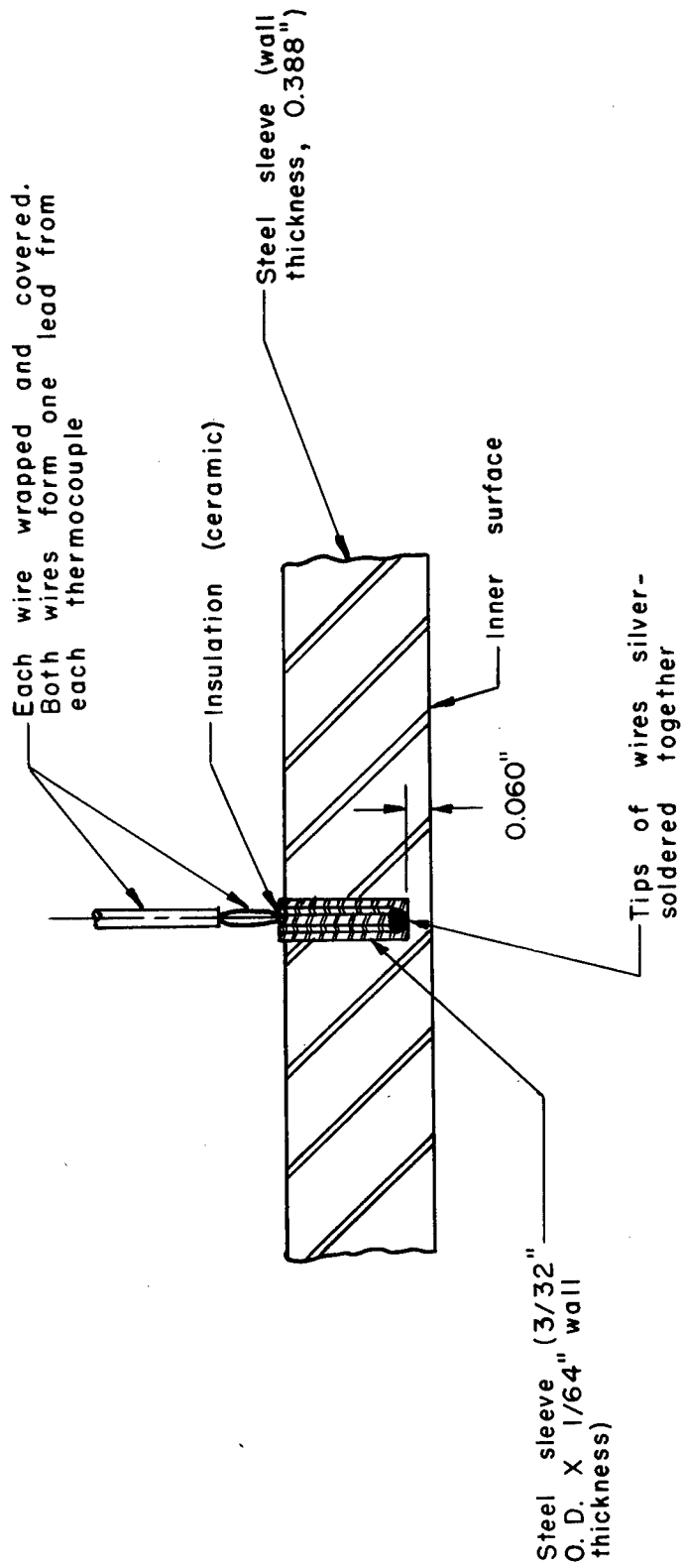
Figure 2.- Thermocouple installation.
