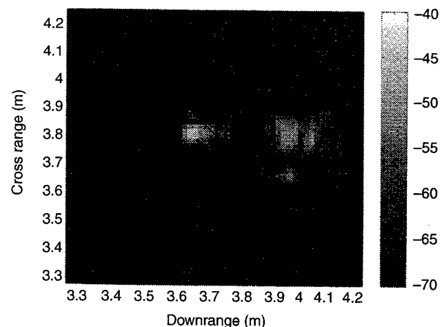
Figure 2. ISAR image of VFY-218 scale model for frequencies 8 to 16 GHz and angles 0 to 40°.
