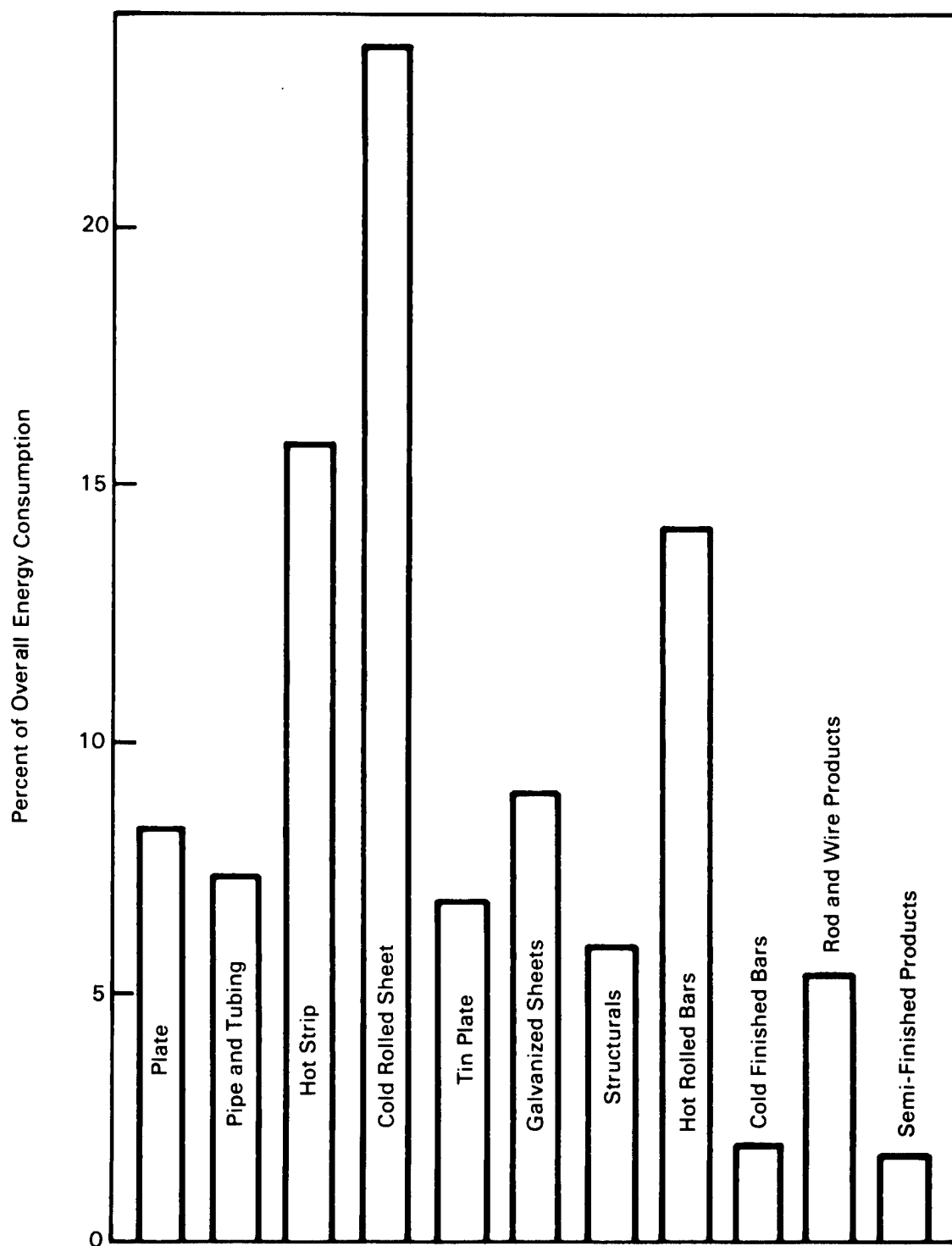
FIGURE 4.2. Distribution of Energy Use in the Major Energy-Consuming Processes
