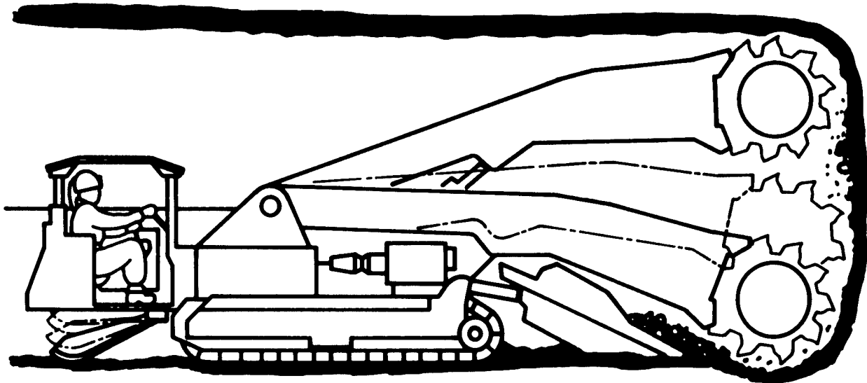
FIGURE 2.4. One Type of Continuous Mining Machine
