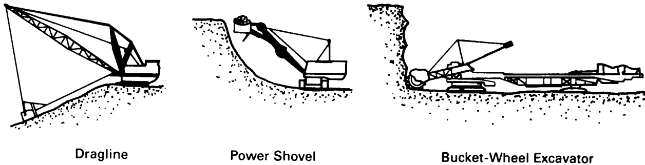
FIGURE 2.2. Surface Mining Exposing and Digging Equipment
