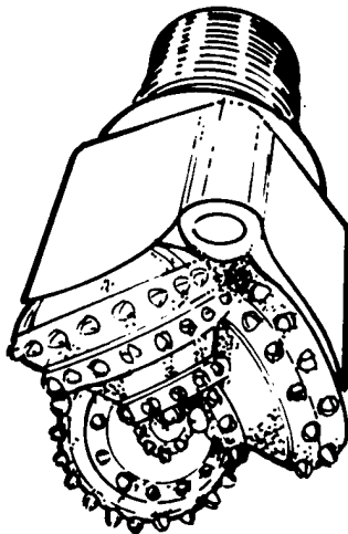
Rolling Cutter Bit
