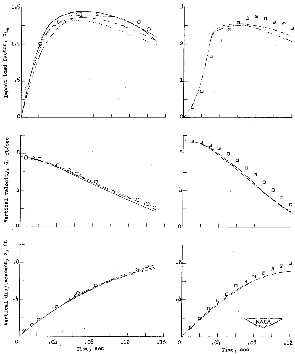
Figure 10.- Comparisons of theoretical and experimental impact time histories for 0° and 30° angles of dead rise.
