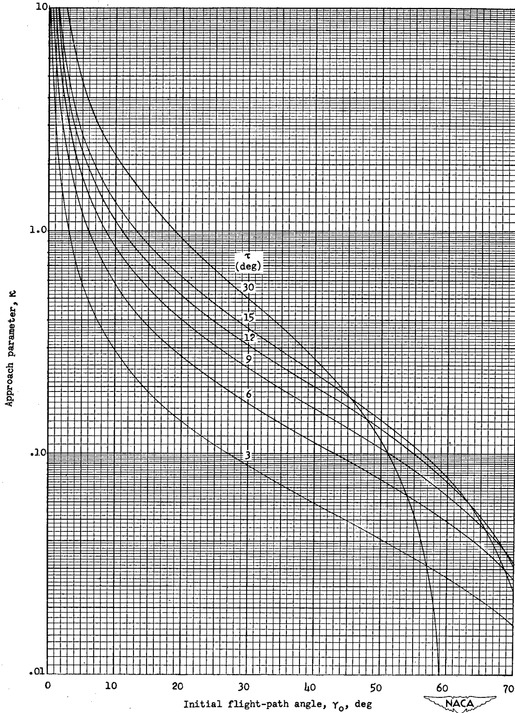
Figure 4.- Variation of approach parameter with trim and flight-path angle. \kappa = \frac{\sin \tau}{\sin \gamma_0} \cos(\tau + \gamma_0) .
