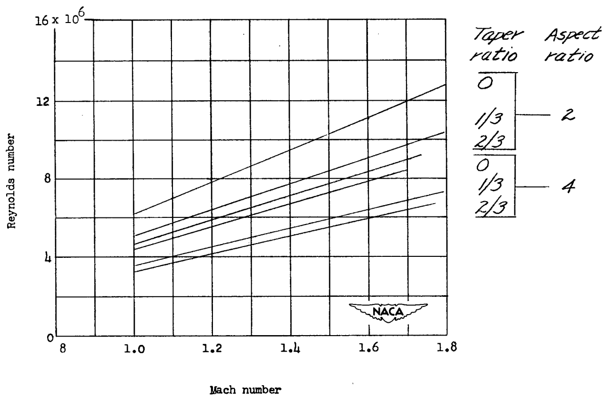
Figure 3.- Variation of Reynolds number with Mach number for each test configuration. Reynolds number based on mean aerodynamic chord of exposed wing surfaces.
