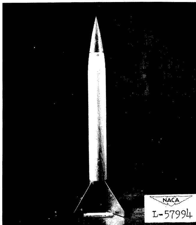
(a) Wingless body.
