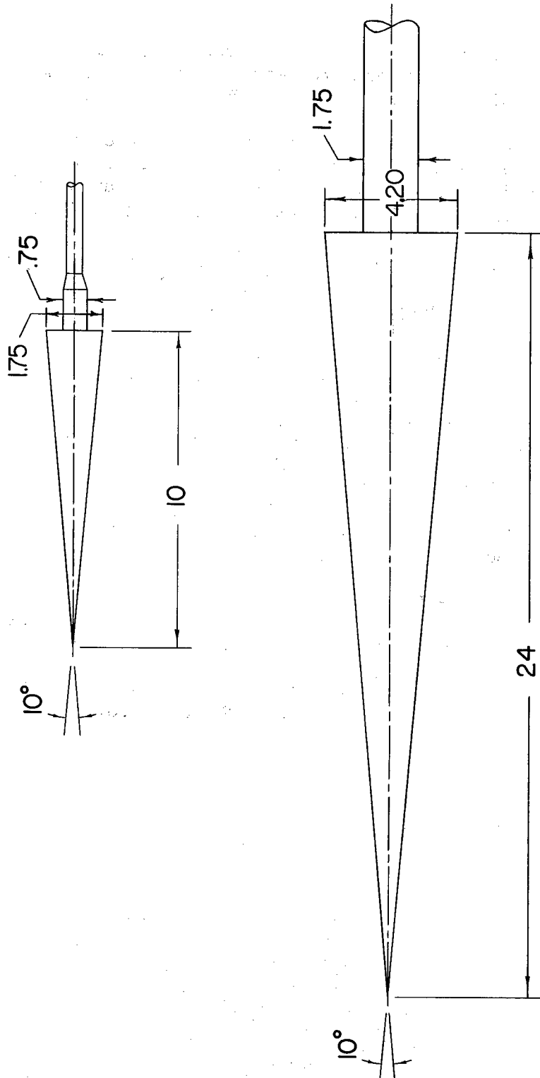
Figure 1.- Sketch of 10° cones. All dimensions are in inches.
