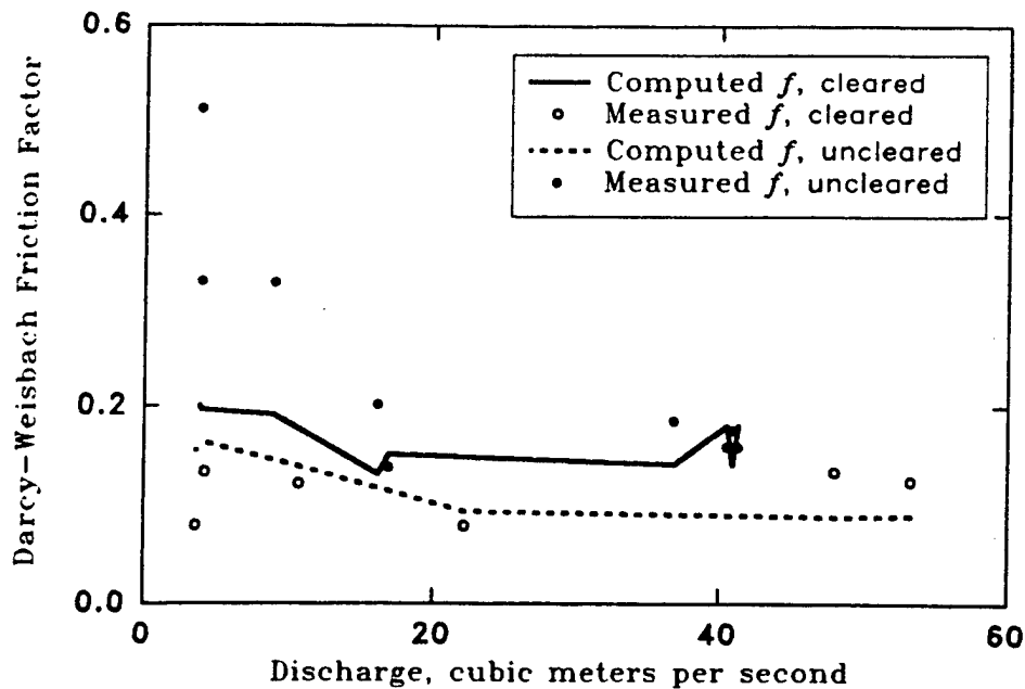
Figure 2. Measured and computed Darcy-Weisbach friction factors versus discharge for cleared and uncleared reaches. — computed f , cleared; \circ measured f , cleared; ..... computed f , uncleared; \bullet measured f , uncleared.
