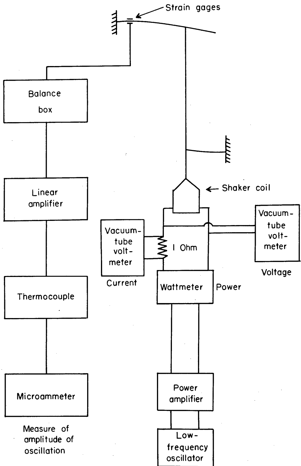
Figure 19.- Block diagram of instrumentation used for three-dimensional tests.
