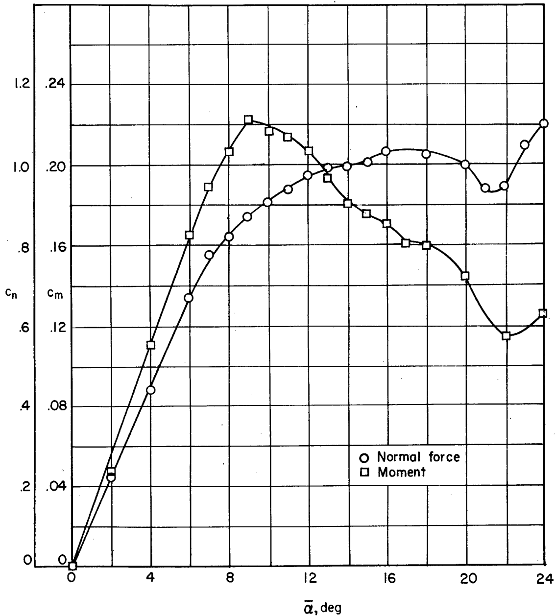
Figure 15.- Variation of static-normal-force and static-pitching-moment coefficients with angle of attack for two-dimensional 65A010 airfoil at Mach number of 0.35.
