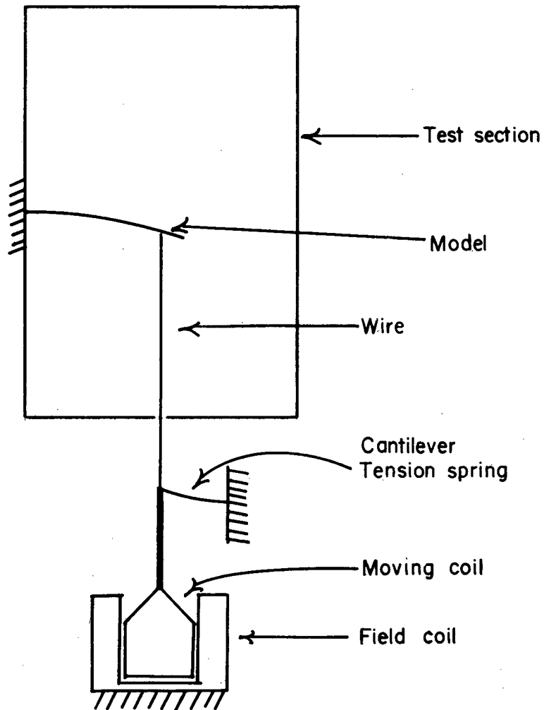
Figure 17.- Schematic drawing of test setup for three-dimensional measurements.
