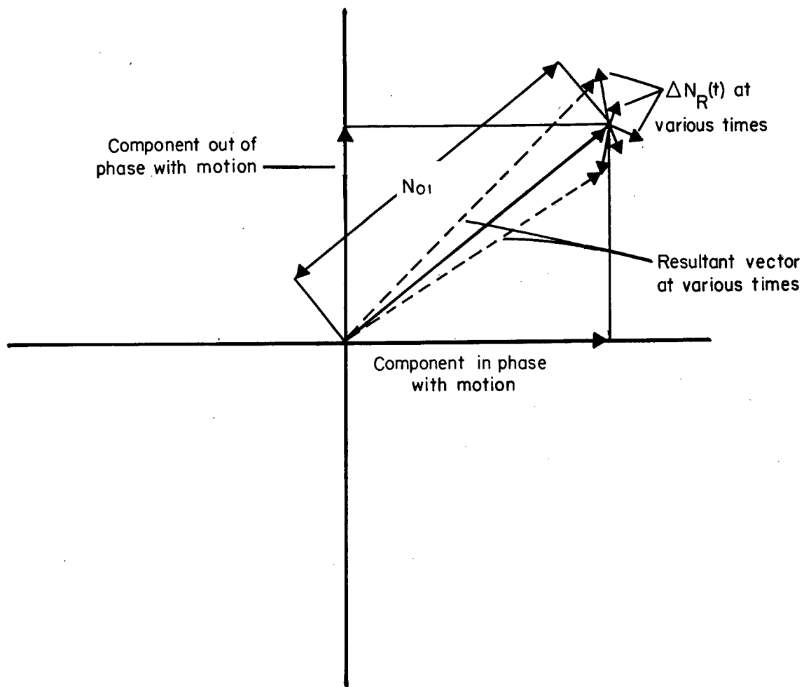
Figure 5.- Vector diagram of filter output tuned to frequency of oscillation.
