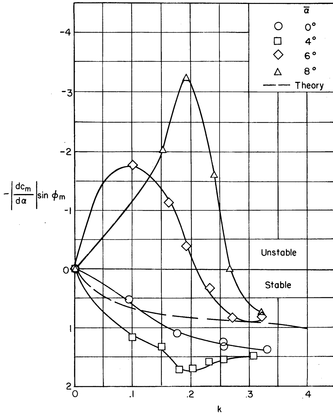
Figure 14.- Variation of damping-moment coefficient with reduced frequency for two-dimensional 65A010 airfoil oscillating in pitch about the mid-chord at Mach number of 0.7.
