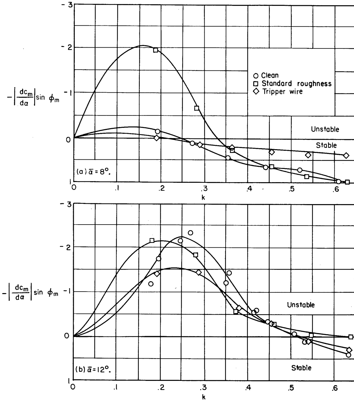
Figure 26.- Variation of damping-moment coefficients with reduced frequency for 65A010 airfoil having three different leading-edge conditions.
