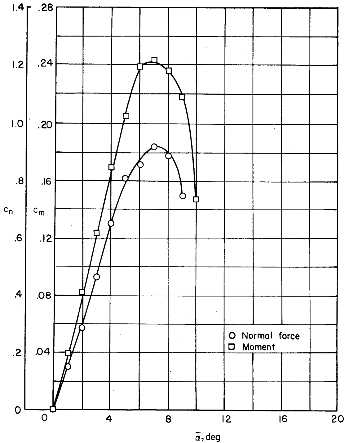
Figure 16.- Variation of static-normal-force and static-pitching-moment coefficients with angle of attack for two-dimensional 65A010 airfoil at Mach number of 0.7.
