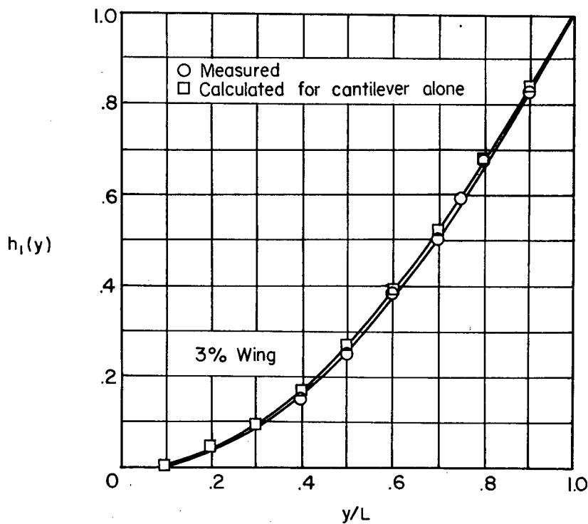
Figure 18.-- Comparison of actual bending modes for three-dimensional tests with calculated fundamental bending modes for same wings as ideal cantilevers.
