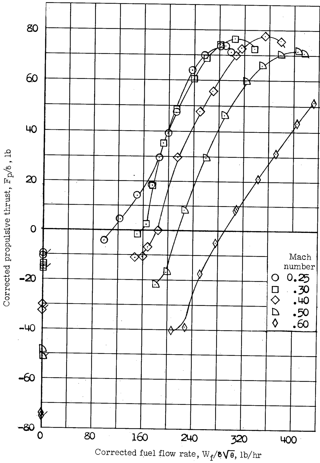
Figure 6.- Corrected pulse-jet propulsive thrust as a function of corrected fuel rate at zero degrees yaw angle for Mach numbers of 0.25, 0.3, 0.4, 0.5, and 0.6.
