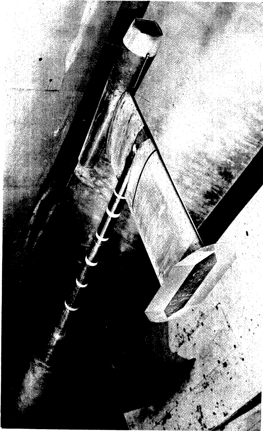
Figure 4.- Installation of pulse-jet engine in Langley 16-foot transonic tunnel for exploratory investigation of the effect of engine firing pulses on airfoil pressure distribution.
