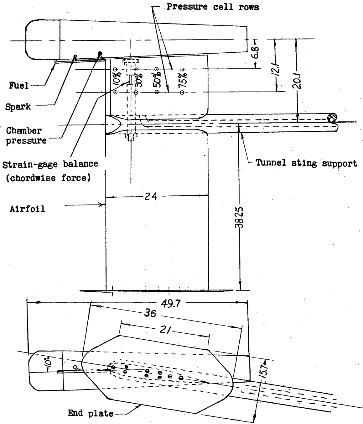
Figure 5.- Detail sketch showing pulse-jet engine mounting and location of pressure cells in simulated rotor blade for investigation of engine firing on airfoil surface pressures.
