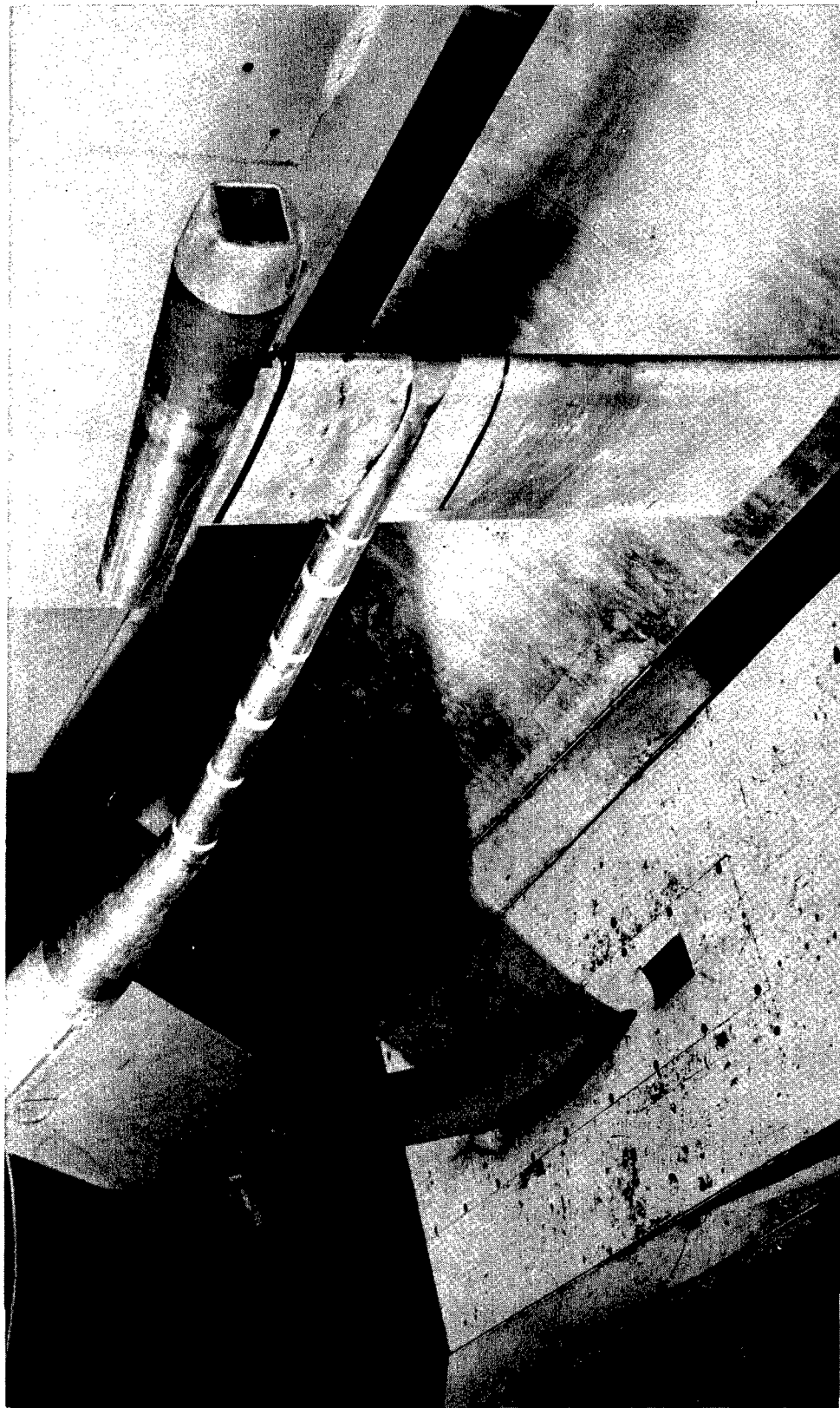
L-86901 Figure 3.- Installation of pulse-jet engine in Langley 16-foot transonic tunnel for investigation of the effects of velocity and yaw angle on propulsive characteristics.
