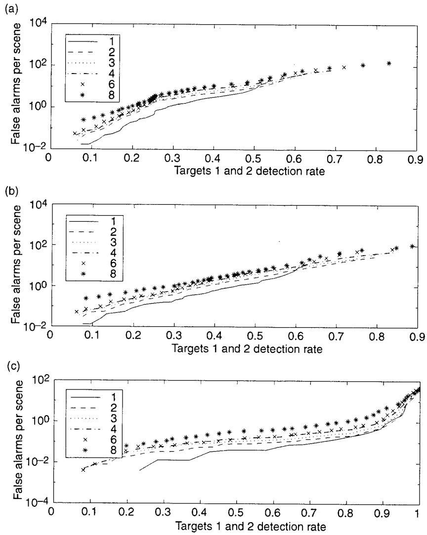
Figure 2. Target-detection rate versus false alarms. Legends show filter counts of 1 to 4, 6, and 8 and three circle radii (a) 3, (b) 5, and (c) 10 pixels.
