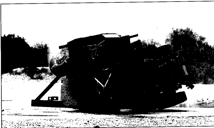
Shown above is the PLS truck as it rolls over on a specially engineered ramp.
