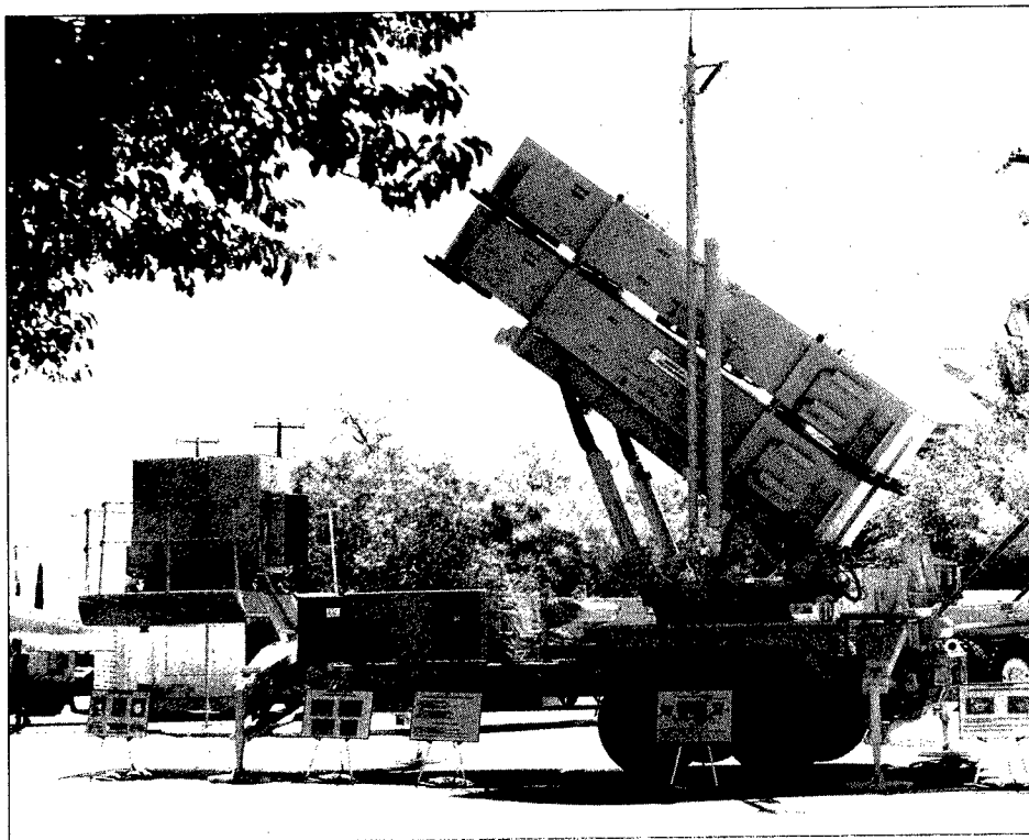
PAC-3 launcher.
