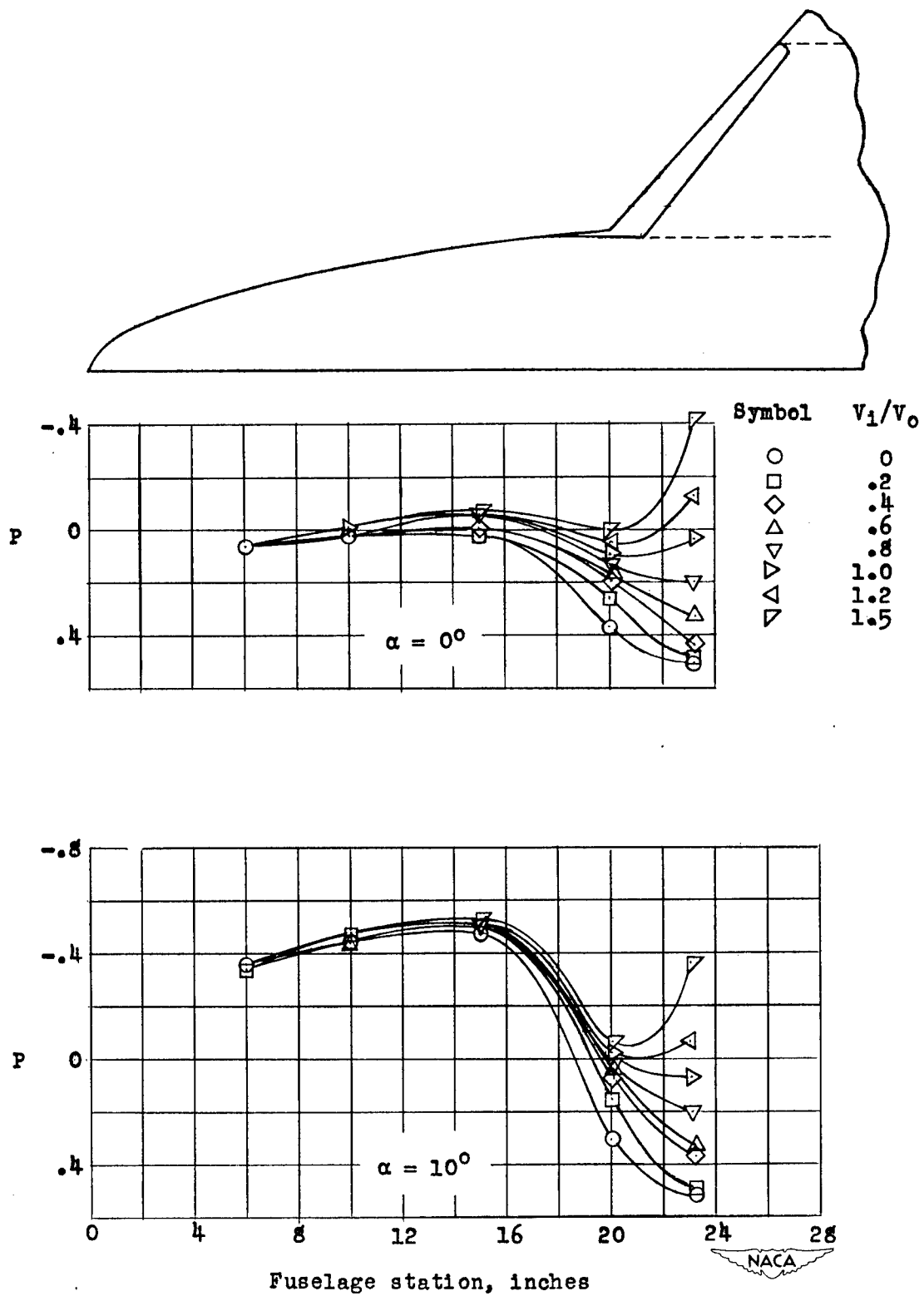
Figure 10.- Static-pressure distribution over nose of final-inlet-model fuselage.
