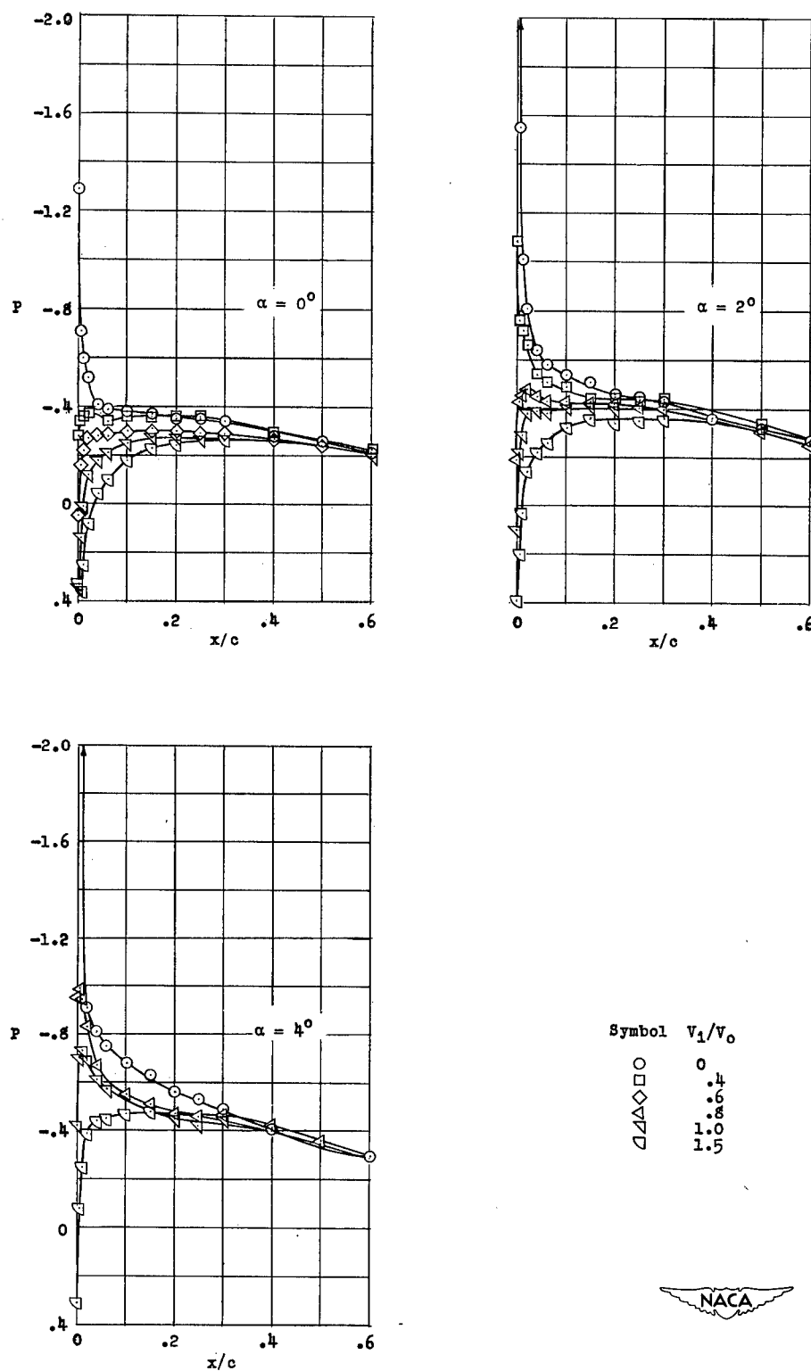
Figure 6.- Static-pressure distribution over the upper surface at station 10 of the original inlet.
