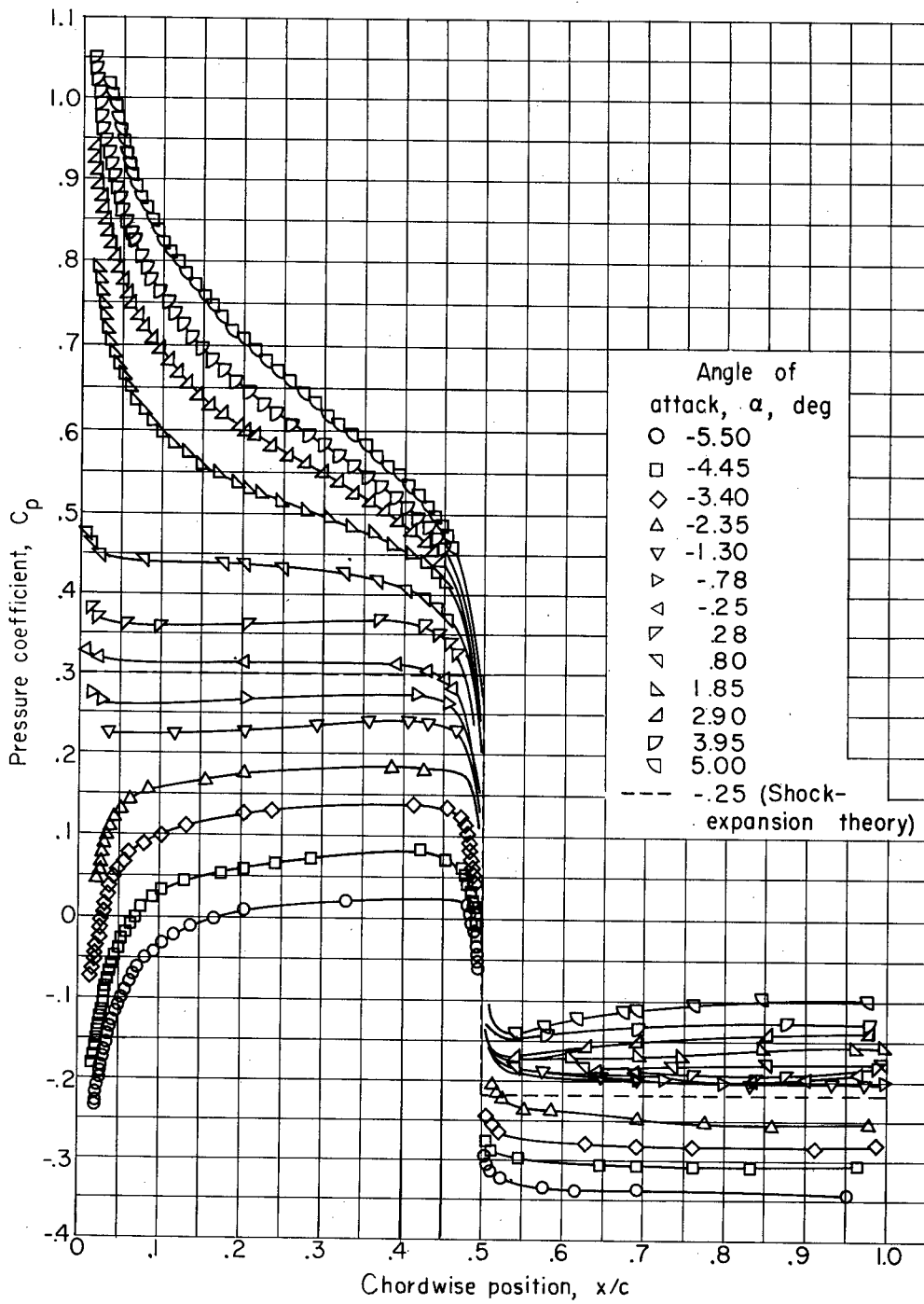
(a) t/c = 0.10 ; M = 1.30 .
