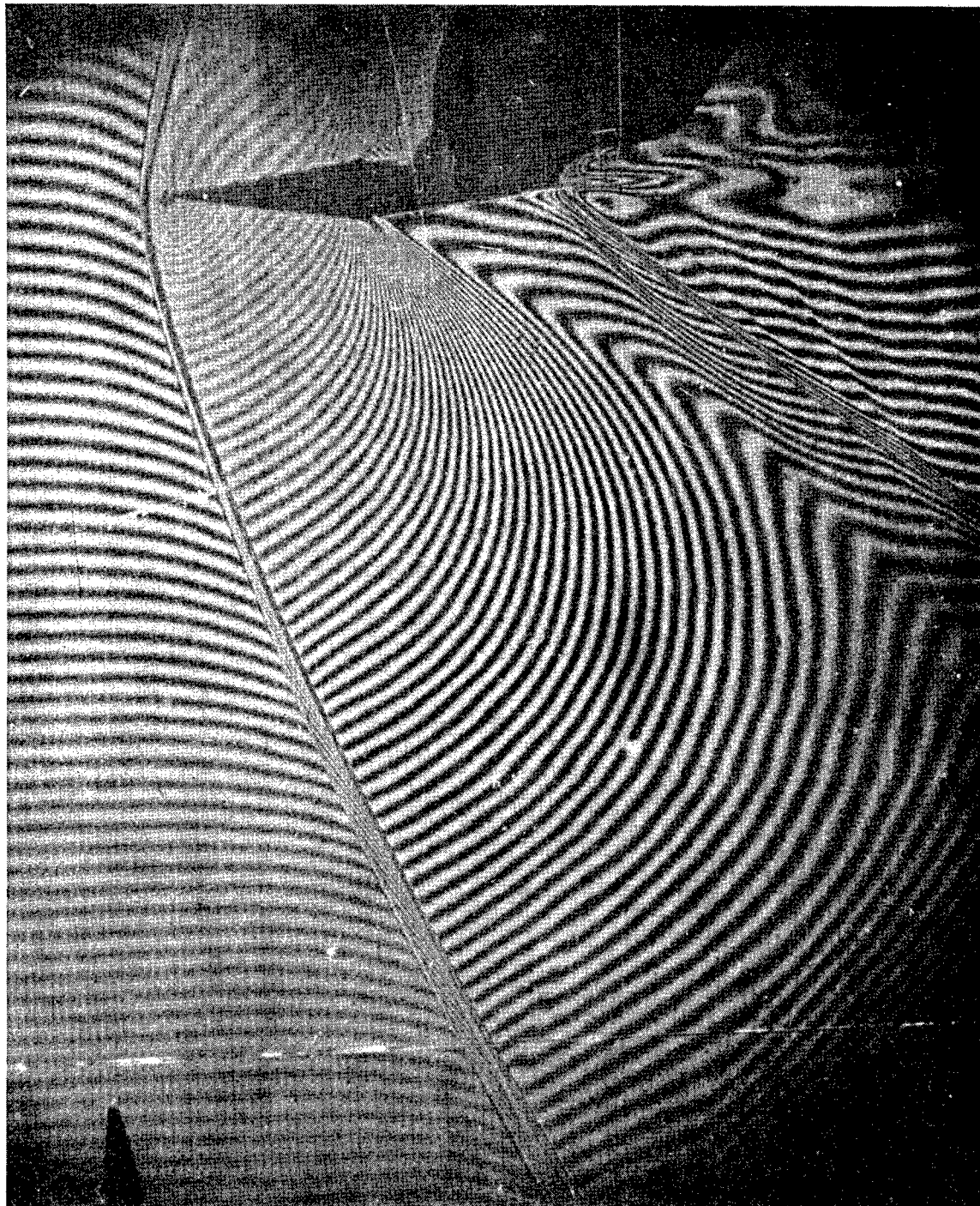
(b) \alpha = 0.95^\circ .
