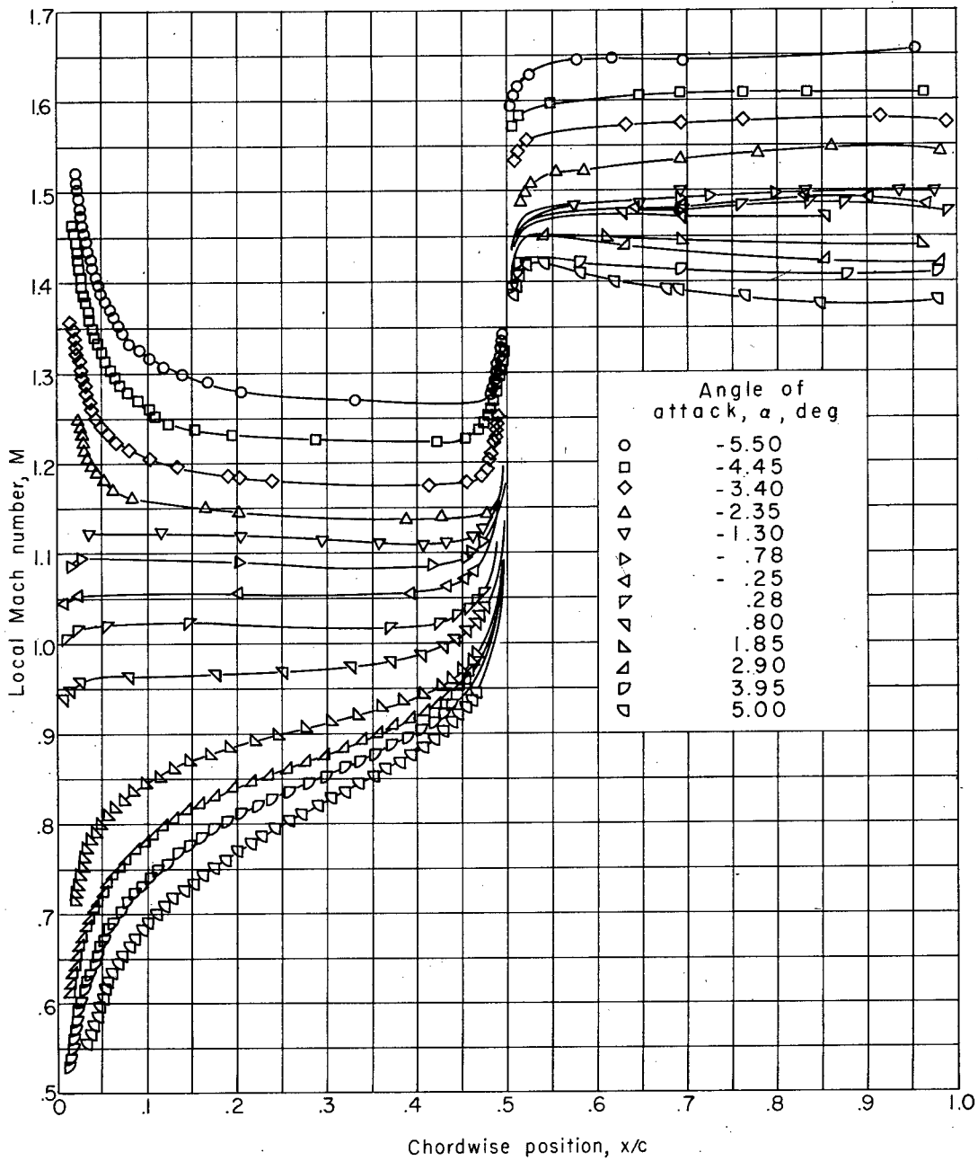
(a) t/c = 0.10 ; M = 1.30 .
