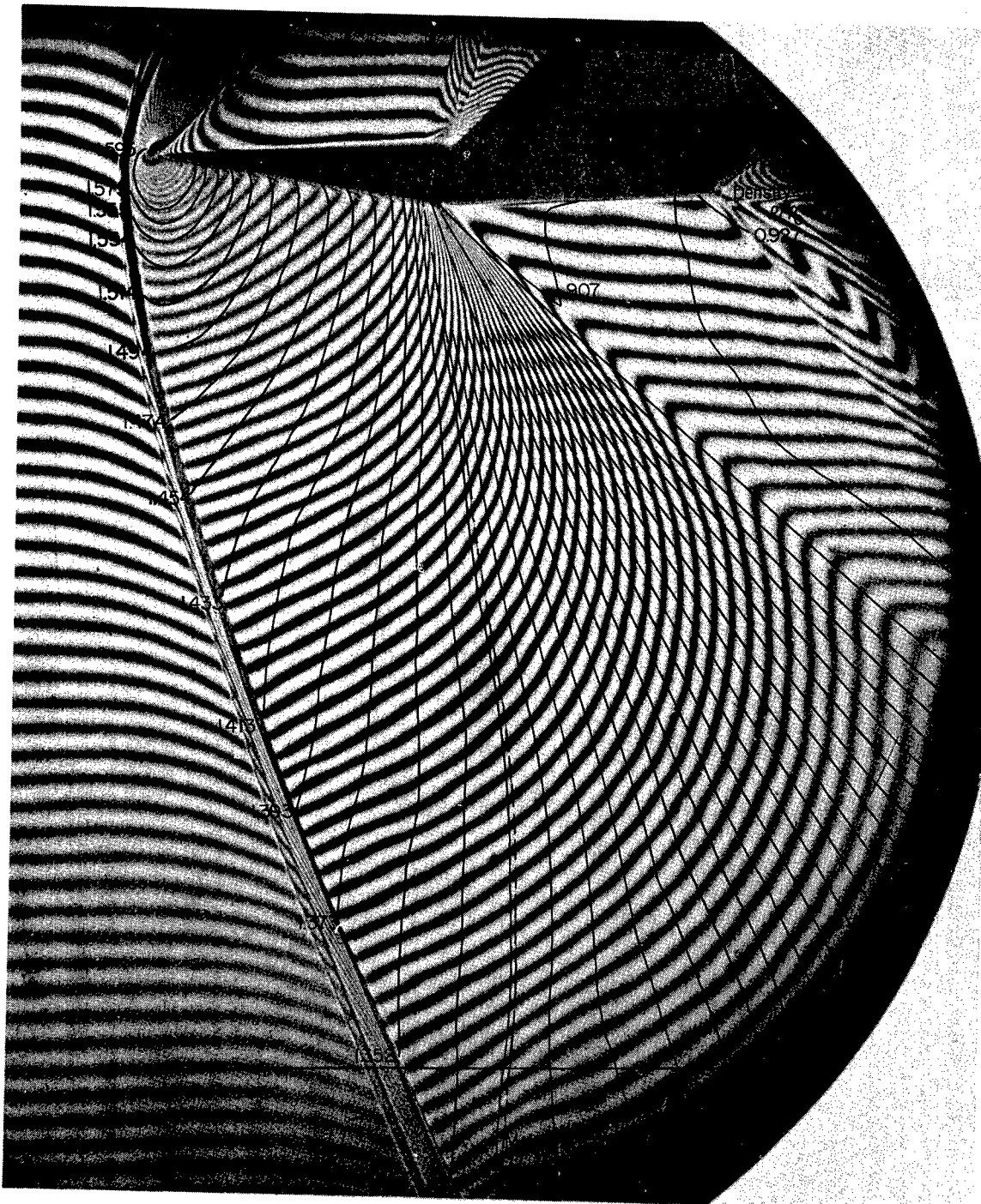
(e) \alpha = 3.95^\circ .
