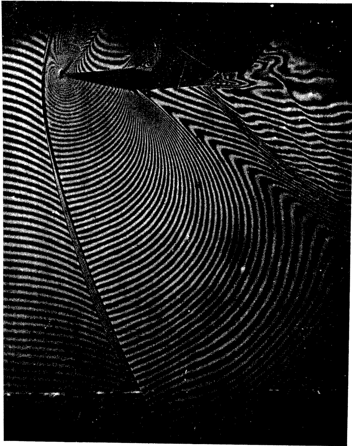
(e) \alpha = 4.25^\circ .
