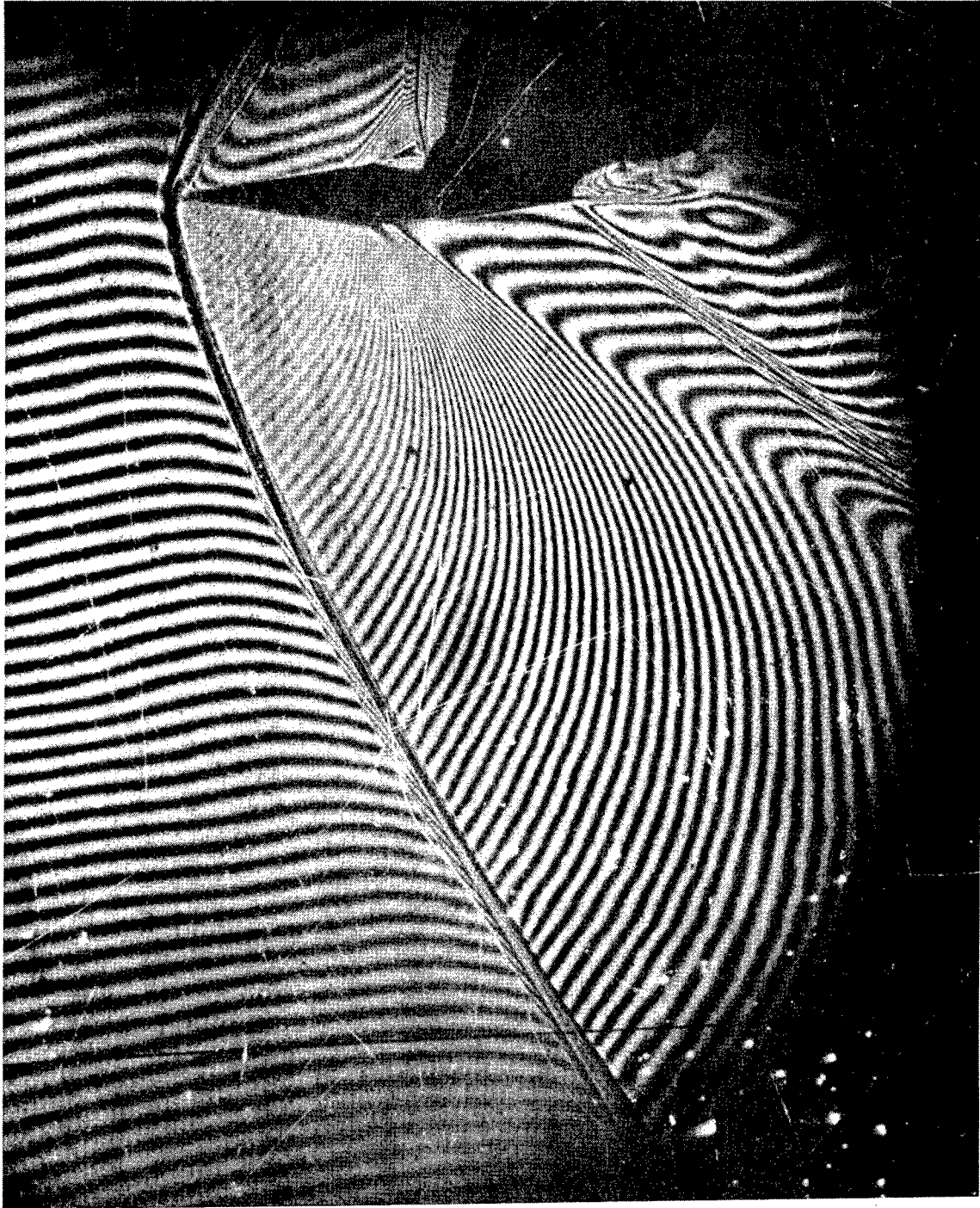
(e) \alpha = 4.00^\circ .
