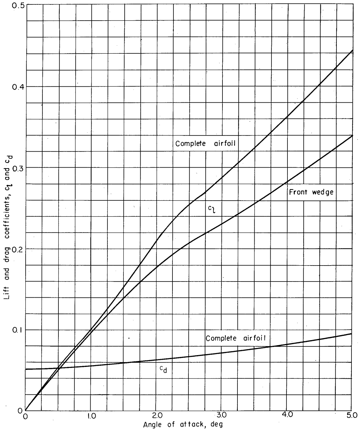
(a) \xi_0 = 1.26 ( t/c = 0.10 ; M = 1.30 ).
