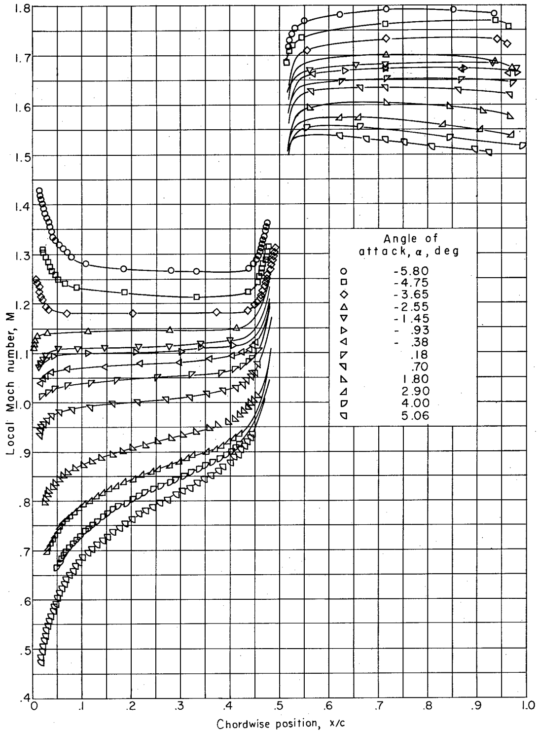
(c) t/c = 0.142 ; M = 1.41 .
