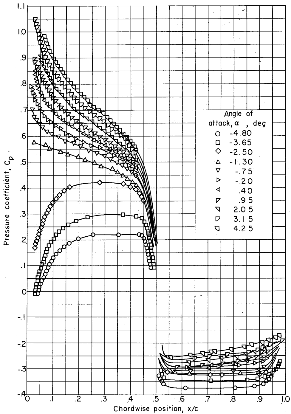
(b) t/c = 0.142 ; M = 1.30 .
