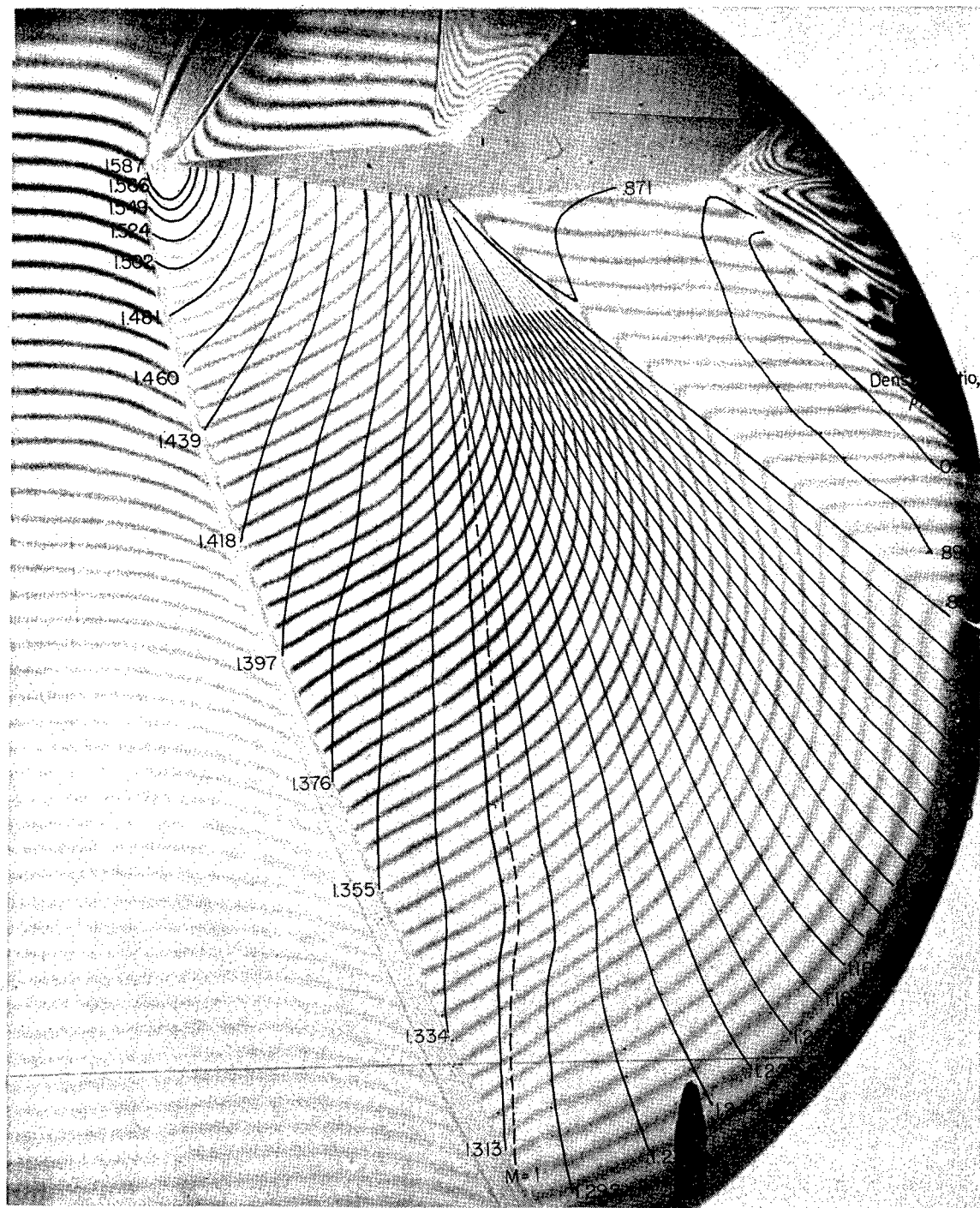
(a) \alpha = 2.90^\circ .
