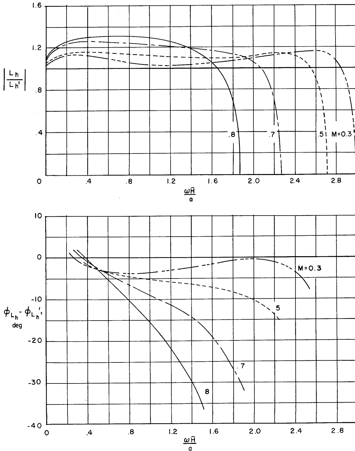
Figure 6.- Effect of variation in Mach number at constant height-semichord ratio H = 7.60 on the magnitude and phase angle of the lift of a translating wing.
