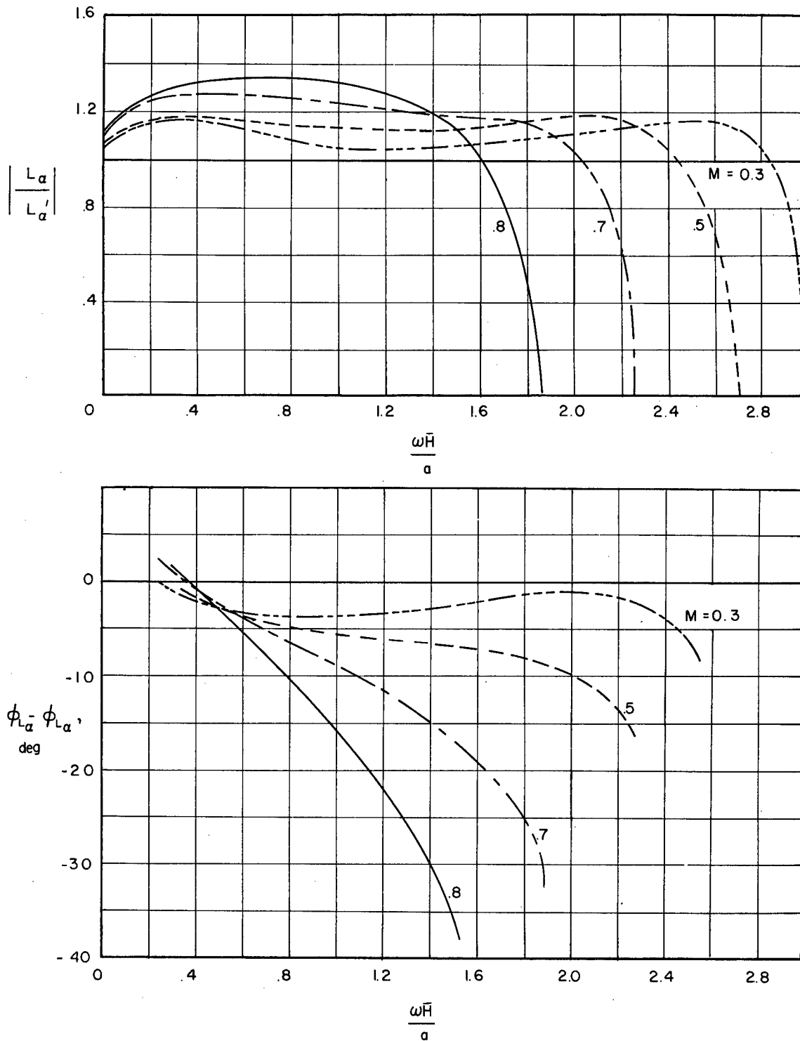
Figure 5.- Effect of variation in Mach number at constant height-semichord ratio H = 7.60 on the magnitude and phase angle of the lift of a pitching wing.
