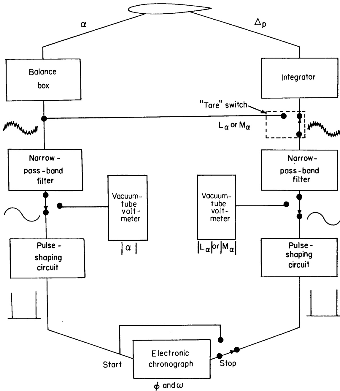
Figure 3.- Schematic diagram of instrumentation.
