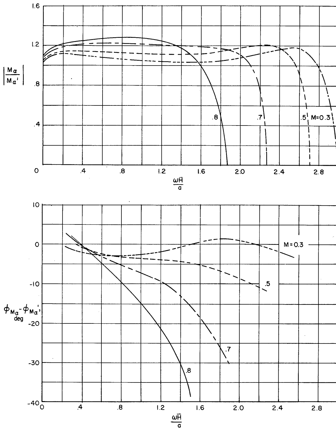
Figure 7.- Effect of variation in Mach number at constant height-semichord ratio H = 7.60 on the magnitude and phase angle of the moment of a pitching wing.
