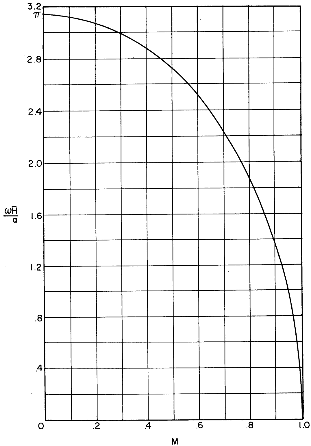
Figure 1.- Fundamental critical values of frequency parameter \frac{\omega H}{a} as a function of Mach number.
