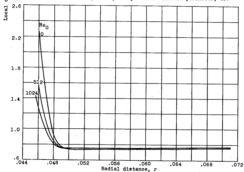
Figure 12. - Concluded. Local concentration factor as function of radial distance of inlet opening. Inlet velocity ratio, 0.7.
